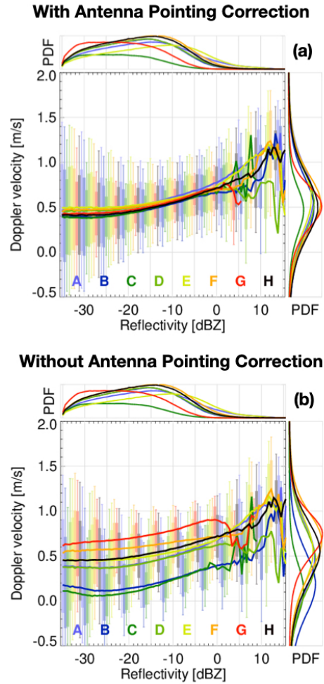
315 Figure 8: Reflectivity–Doppler velocity (Z–V) relationships of ice clouds for temperatures between -30^{\circ}\text{C} and -40^{\circ}\text{C} for the month of January 2025. Panels (a) and (b) depict the Z–V relationships with and without the antenna pointing correction, respectively. Each color represents a different frame ID, while the vertical bars indicate the 10th, 25th, 75th, and 90th percentiles, and the solid lines represent the median. The overlaid probability density functions (PDF) on the top and right axes illustrate the distribution of reflectivity and Doppler velocity number of samples contributing to each range. Note that the C-CD L2a product inverts the 320 velocity sign with respect to the C-NOM L1b product
