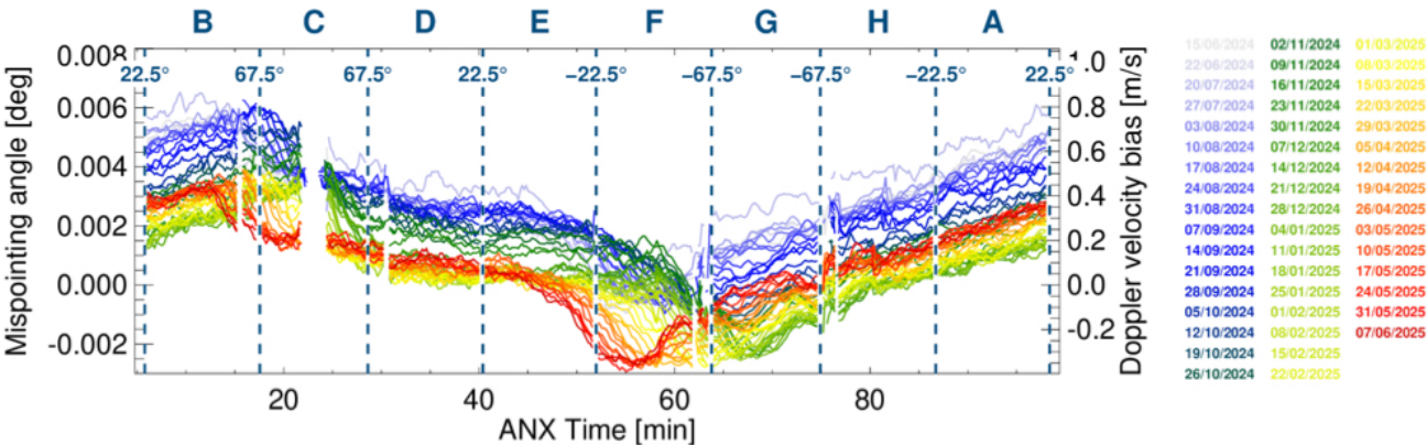
210 Figure 4: Weekly averaged EarthCARE’s CPR antenna mispointing angle as a function of ANX time (time since ascending node crossing) derived from clear-sky surface Doppler velocity measurements collected over sea surface (free of ice) and snow-covered land from June 2024 to June 2025. The letters on top correspond to the frame ID, which denote the different segments of the orbit,
