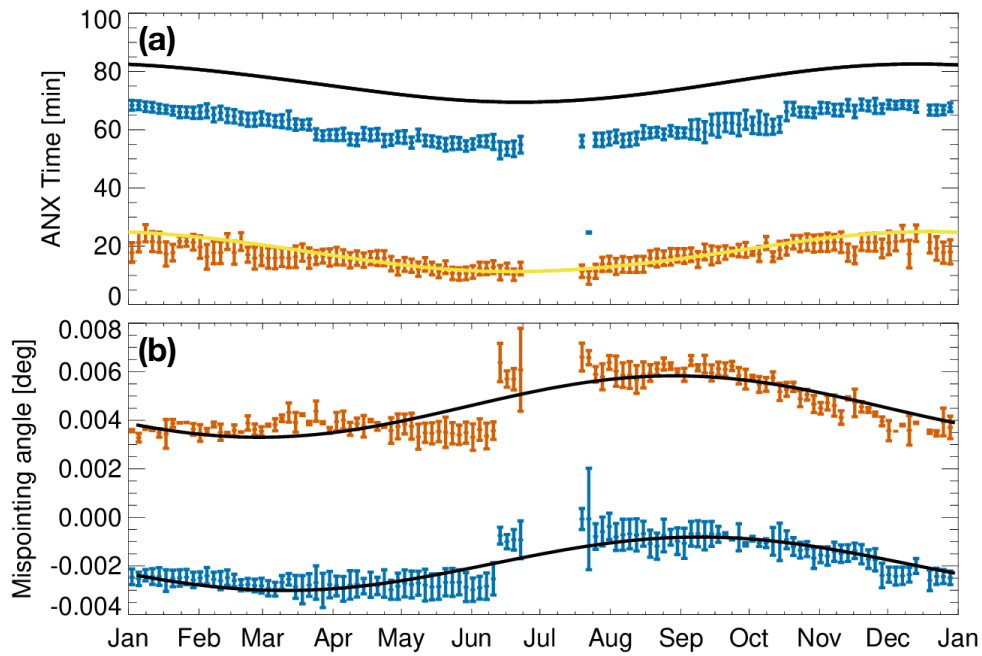
Figure 5: Panel (a) shows the ANX time of the minimum (blue) and maximum angles (red) of the weekly averaged mispointing trends as a function of time of year. The yellow and black lines denote the spacecraft's daylight entry and exit times, respectively. Panel (b) presents the minimum (blue) and maximum (red) angles of the weekly averaged mispointing trends as a function of time of year, with black lines representing fitted harmonics. In both panels, the vertical bars indicate the standard deviation. Gaps correspond to periods not yet covered by CPR measurements.
