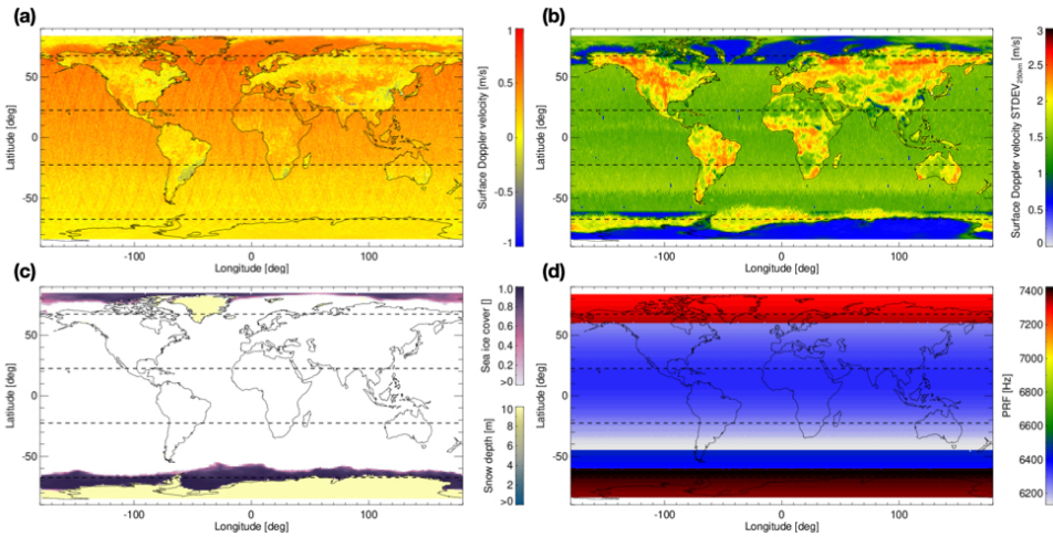
205 Figure 3: Panels (a) and (b) depict the global surface Doppler velocity tendency and variability, represented by the median of the mean and standard deviation values, both calculated from orbit-to-orbit measurements within a 250 km along-track window collected from August to November 2024. Panel (c) depicts the ECMWF average model sea ice cover and snow depth for the same period, and panel (d) the default variable EarthCARE CPR's pulse-repetition frequency (PRF) configuration changing as a function of latitude. The horizontal dashed lines are plotted to indicate the boundaries of the orbit's segments, defined by frame IDs: (A) +22.5° to -22.5° ascending, (B) +22.5° to +67.5° ascending, (C) +67.5° ascending to +67.5° descending, (D) +67.5° to +22.5° descending, (E) +22.5° to -22.5° descending, (F) -22.5° to -67.5° descending, (G) -67.5° descending to -67.5° ascending, and (H) -67.5° to -22.5° ascending.
