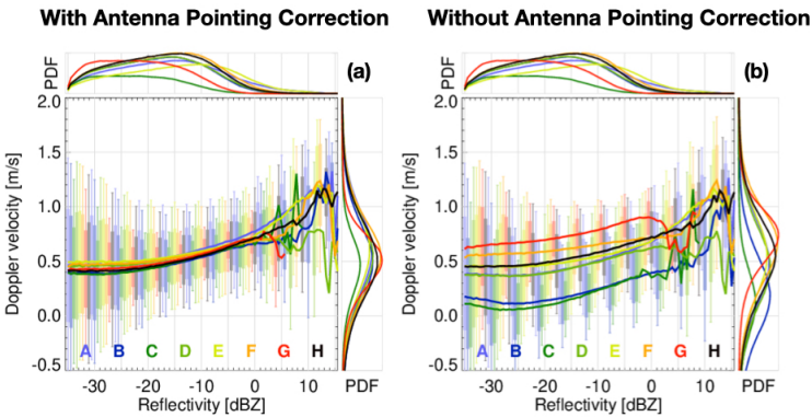
355 Figure 8: Reflectivity–Doppler velocity (Z–V) relationships of ice clouds for temperatures between -30°C and -40°C for the month of January 2025. Panels (a) and (b) depict the Z–V relationships with and without the antenna pointing correction, respectively. Each color represents a different frame ID, while the vertical bars indicate the 10th, 25th, 75th, and 90th percentiles, and the solid lines represent the median. The overlaid probability density functions (PDF) on the top and right axes illustrate the distribution of reflectivity and Doppler velocity number of samples contributing to each range. Note that the C-CD L2a product inverts the velocity sign with respect to the C-NOM L1b product 360
