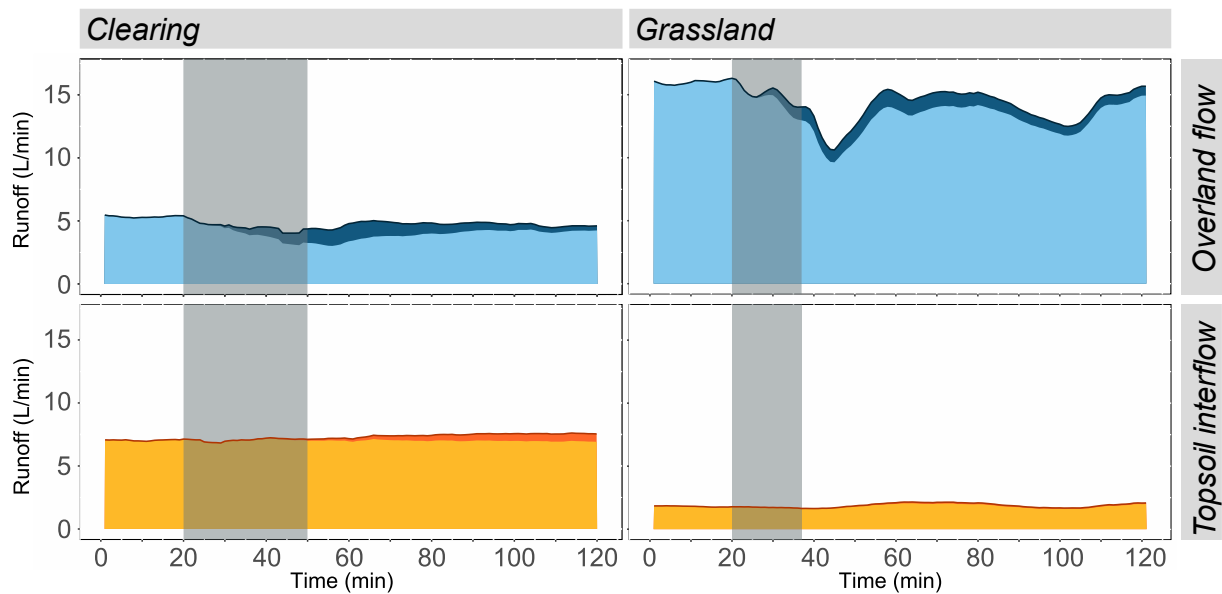
Figure 7: Overland flow (top row, blue) and topsoil interflow (bottom panel, orange) rates, with the contribution of the deuterium -labelled water represented by the darker shades of blue and orange, respectively for the plot in the clearing (left) and the plot in the grassland (right). The grey shading indicates the time of the application of the deuterium -labelled water. Note that time 0 in the figure for the clearing (left) corresponds to minute 138 th minute in Figure 4a, and for the plot in the grassland (right) to minute 50 in Figure 4b.
