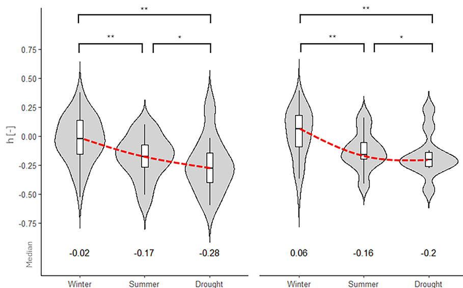
Figure 6. (Left) Violine plots of h -Index values (GW1), below median value of the integrated boxplot per season. (Right) Violine plots of h -Index values (GW2), below median value of the integrated boxplot per season. Comparison between Winter ( n = 37 ), summer ( n = 22 ), and drought ( n = 9 ). Significant difference between groups indicated by * ( *** p = 0.001 , ** p = 0.01 , * p = 0.05 , Wilcoxon Signed-Rank Test). Red dotted line showing decline in median h -Index value between seasons.
