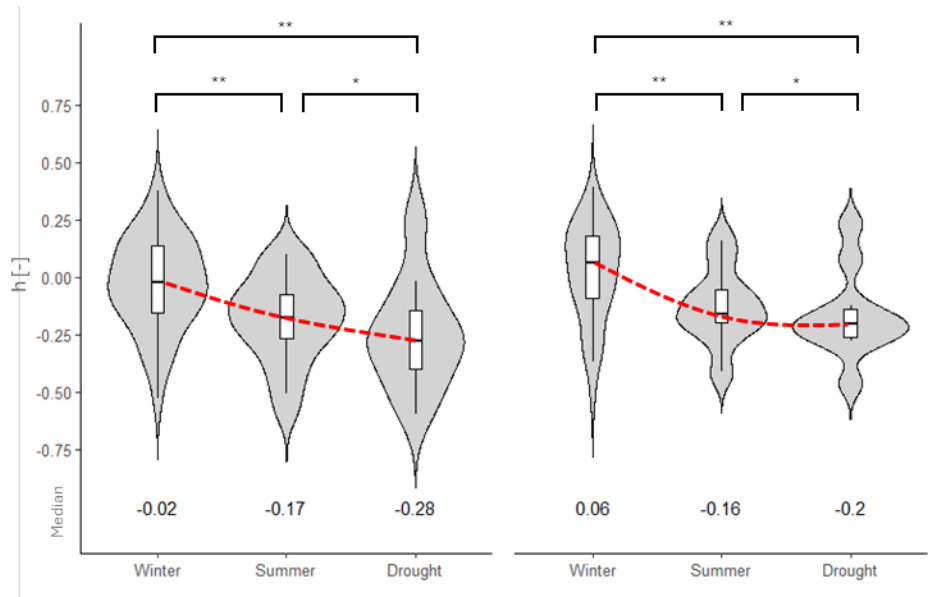
Figure 6: (Left) Violine plots of h-index values (GW1), below median value of the integrated boxplot per season. (Right) Violine plots of h-index values (GW2), below median value of the integrated boxplot per season. Comparison between Winter (n= 37), summer (n=22), and drought (n= 9). Significant difference between groups indicated by * (** p = 0.001, ** p = 0.01, * p = 0.05, Wilcoxon Signed-Rank Test). Red dotted line showing decline in median h-index value between seasons.
