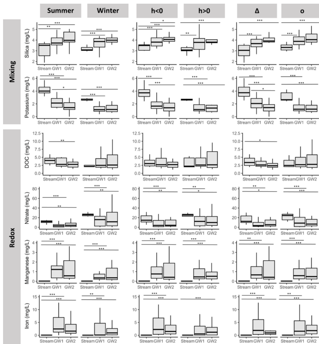
Figure 9: Boxplots of water chemistry parameters separated by (a) season (Summer / Winter), (b) hysteresis direction ( h < 0 / h > 0 ), and (c) hydraulic conditions (Gaining / Losing). (a) Mixing proxies between groundwater and surface water represented by Silica (GW) and Potassium (SW). (b) Redox-sensitive compounds representing the redox chain: DOC, Nitrate, Manganese, and Iron. Significant differences (* p < 0.05 , ** p < 0.01 , *** p < 0.001 ; Wilcoxon rank-sum test) between the sampling locations Stream, GW1, and GW2 are indicated by stars above the boxplots. Transect between Stream, GW1, and GW2; n = 48
