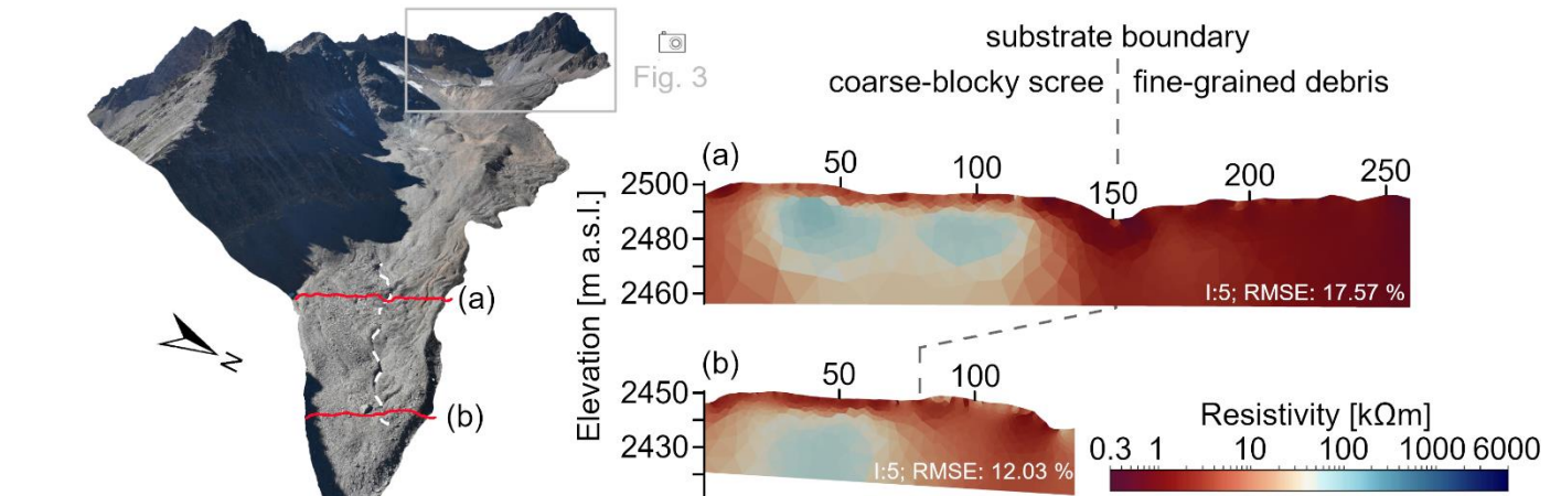
Figure 4: ERT surveys on the Oberferden rock glacier. Position of the substrate boundary is highlighted by the dashed white line on the rock glacier surface. Image extent of Fig. 3 is also marked for orientation by the grey box.
