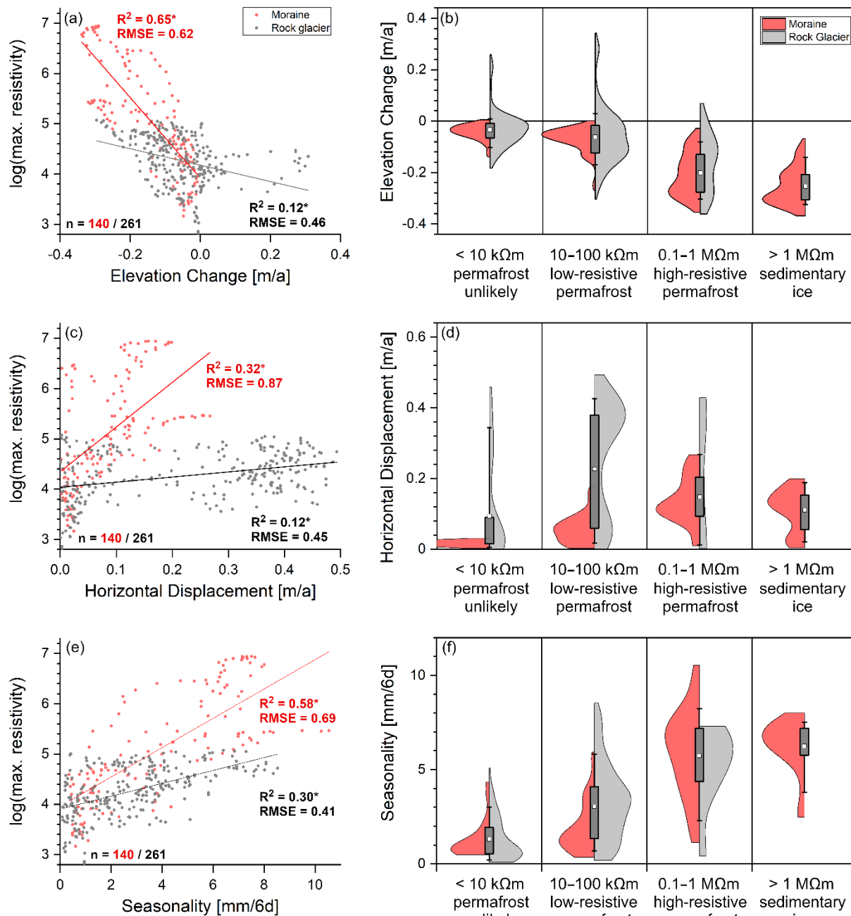
Figure 6: Comparison of InSAR-detected elevation change, horizontal displacement and seasonality with the logarithm of maximum resistivity (in \Omega\text{m} ) below each respective pixel along all 2D ERT profiles. In the left column, the logarithm of the maximum resistivity is plotted against the elevation change (a), horizontal displacement (c) and seasonality (e), while in the right column, the distribution of each parameter is shown for four different resistivity classes (b, d, e). "*" indicates the significance of the respective correlation ( \alpha = 5\% ).
