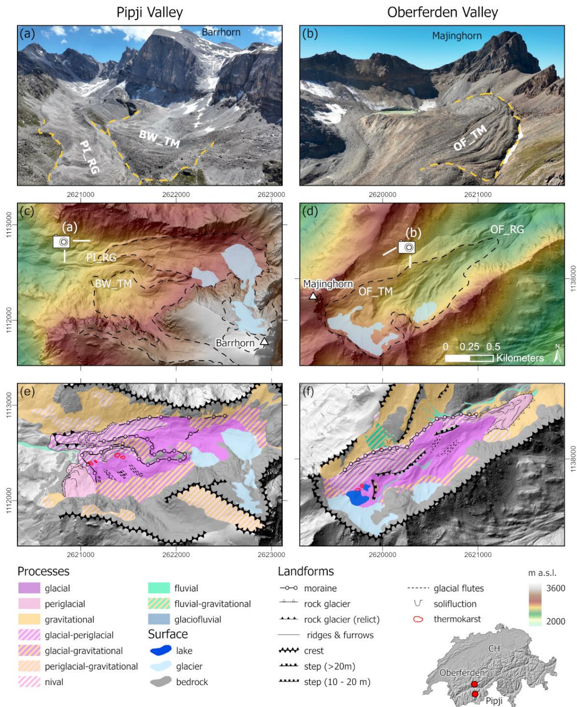
145 Figure 1: Overview of the Pipji Valley (left column) and Oberferden Valley (right column). Aerial images of the study sites are shown in (a) and (b). The middle panels (c) and (d) present the relief of the study sites including the glacial extent of the Little Ice Age (1850 AD) and the image positions of (a) and (b). Geomorphological maps of the sites are shown in the lower panels (e) and (f). Mapping was conducted based on aerial images, digital elevation models and field observations in summer 2023 and 2024. Basemaps provided by © swisstopo.
