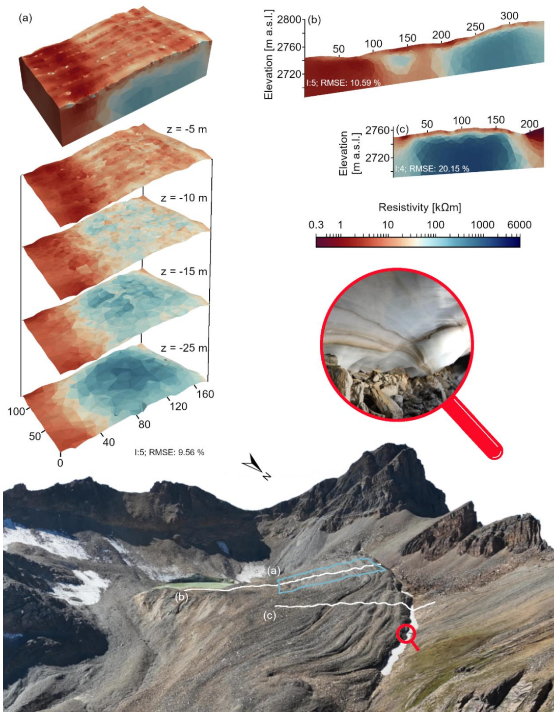
Figure 3: ERT surveys on the Oberferden thrust moraine complex. A q3D model is shown in (a), whereas two 2D cross profiles are shown in (b) and (c). The locations of the ERT surveys are shown in the background image. The magnifier shows an outcrop of massive ice in a thermo-erosional cave in the distal moraine flank (see also Fig. A1 b, d).
