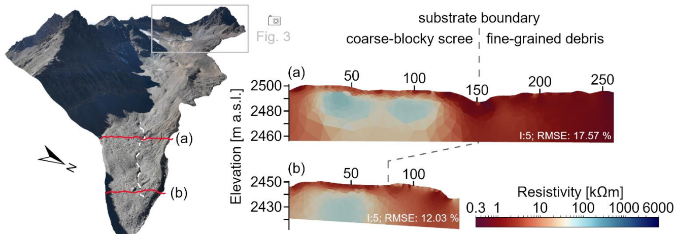
320 Figure 4: ERT surveys on the Oberferden rock glacier. Position of the substrate boundary is highlighted by the dashed white line on the rock glacier surface. Image extent of Fig. 3 is also marked for orientation by the grey box.
