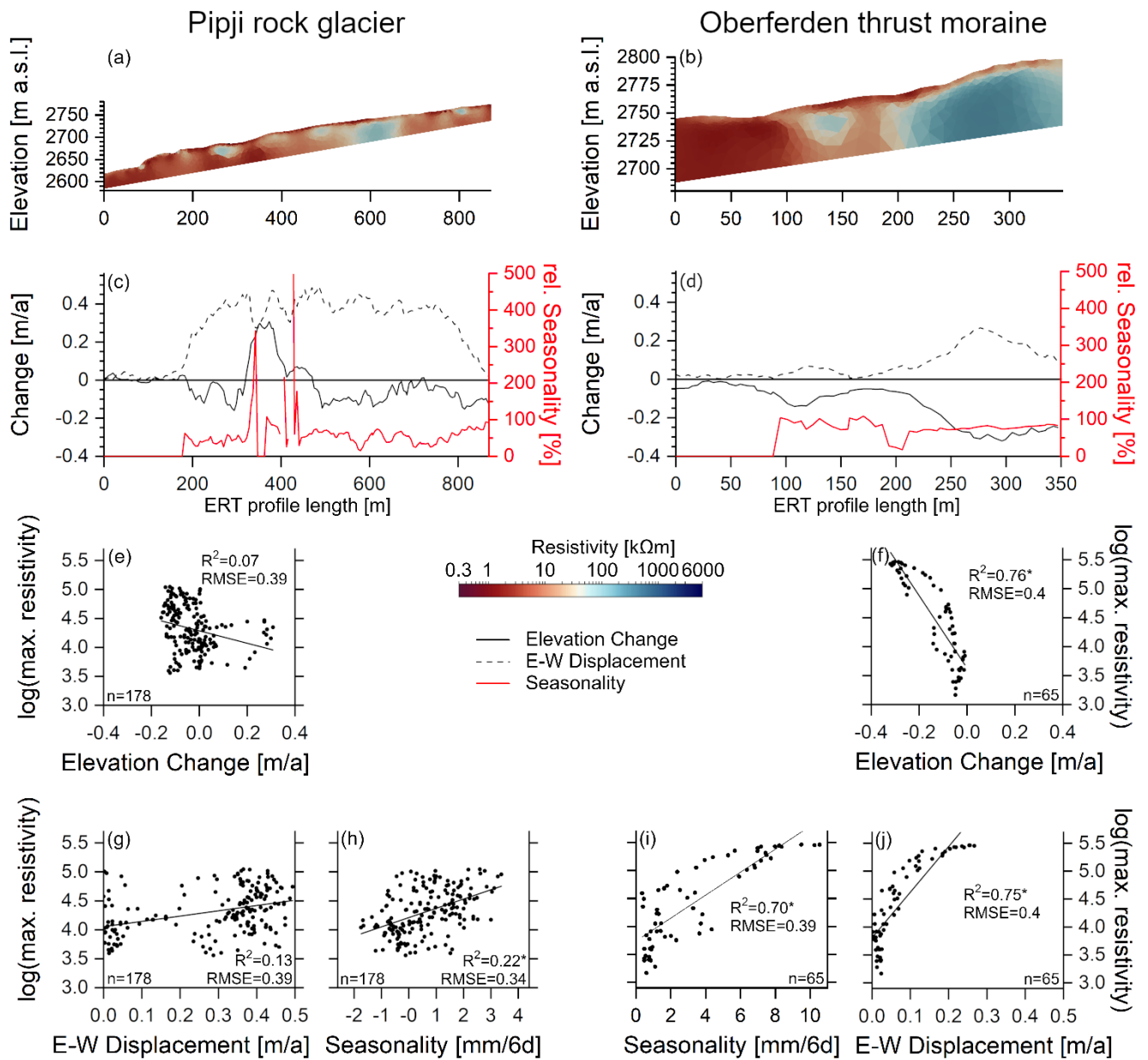
Figure 7: Comparison of the ERT pseudo sections ((a) & (b)) with DInSAR-derived elevation change, horizontal displacement and seasonality ((c) & (d)) along the longitudinal profile of the Pipji rock glacier ((a) & (c)) and the cross profile of the Oberferden thrust moraine complex ((b) & (d)). In the subplots (e) to (j), the individual scatterplots for the relationships are shown. "*" indicates the significance of the respective correlation ( \alpha = 5\% ). Please note the different scalings of x- and y-axis for the two columns.
