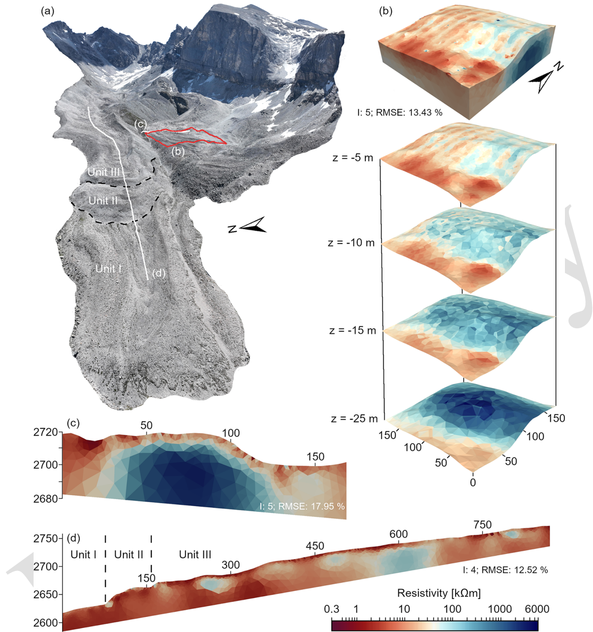
Figure 2. ERT surveys in the Pipji and Barrwang glacier forefields. An overview of the survey location is given in (a). A q3D ERT grid is shown in (b), whereas a 2D cross profile of the thrust moraine complex and a longitudinal profile along the rock glacier are shown in (c, d).
