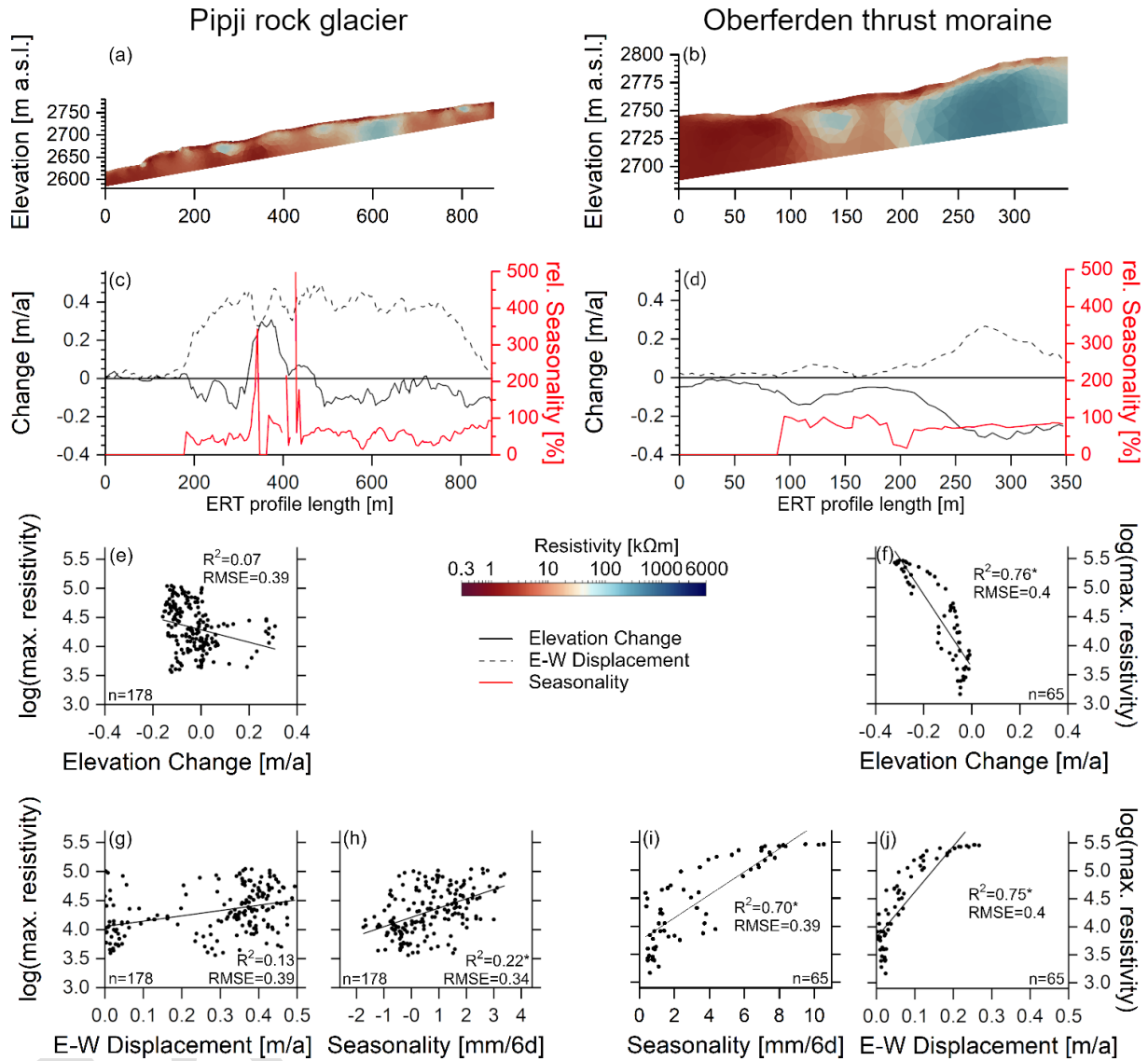
Figure 7. Comparison of the ERT pseudo sections (a, b) with DInSAR-derived elevation change, horizontal displacement and seasonality (c, d) along the longitudinal profile of the Pipji rock glacier (a, c) and the cross profile of the Oberferden thrust moraine complex (b, d). In the subplots (e–j), the individual scatterplots for the relationships are shown. “*” indicates the significance of the respective correlation ( \alpha = 5\% ). Please note the different scalings of x- and y-axis for the two columns.
