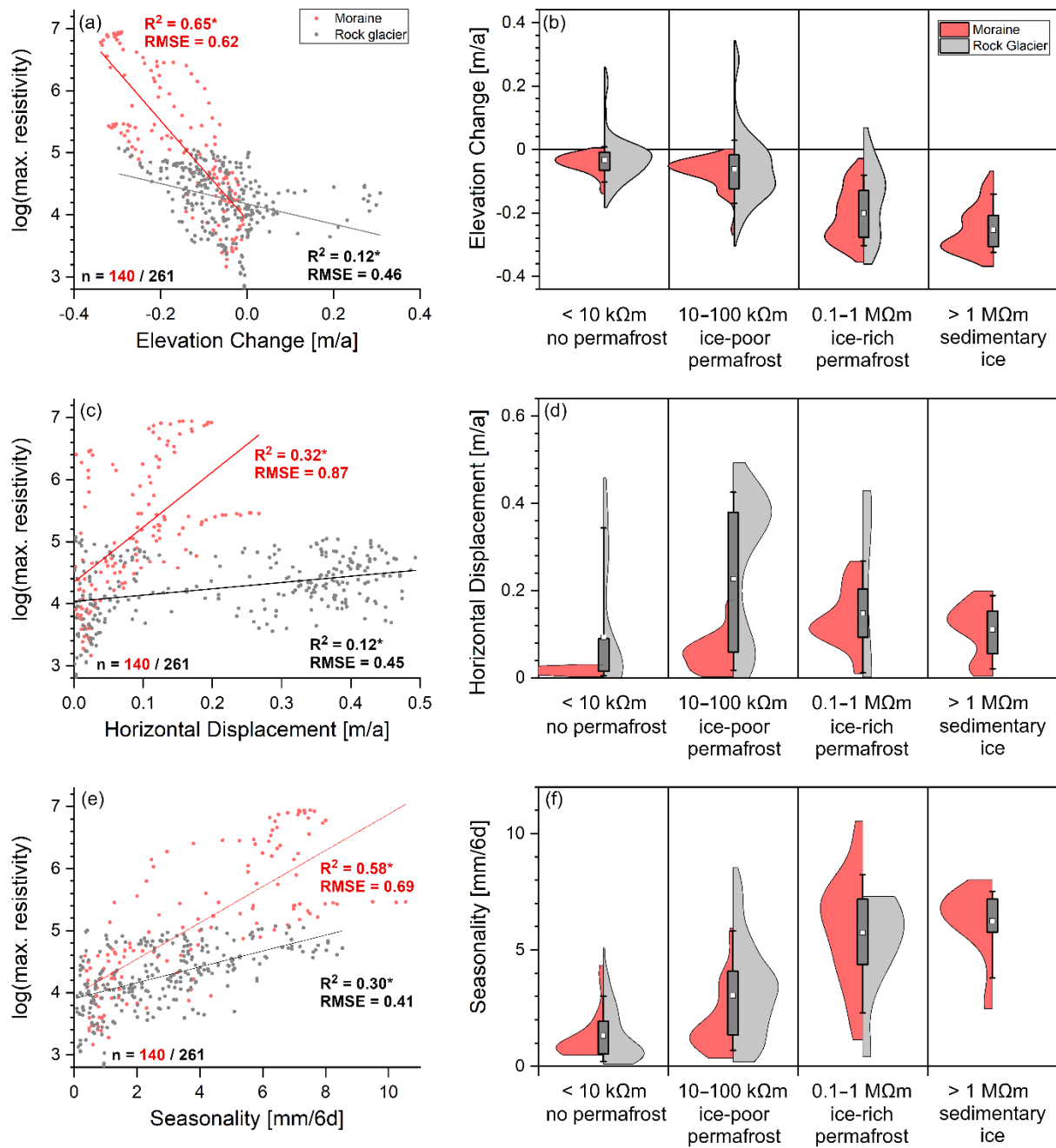
410 Figure 6: Comparison of InSAR-detected elevation change, horizontal displacement and seasonality with the logarithm of maximum resistivity (in \Omega\text{m} ) below each respective pixel along all 2D ERT profiles. In the left column, the logarithm of the maximum resistivity is plotted against the elevation change (a), horizontal displacement (c) and seasonality (e), while in the right column, the distribution of each parameter is shown for four different resistivity classes (b, d, e). “*” indicates the significance of the respective correlation ( \alpha = 5\% ).
