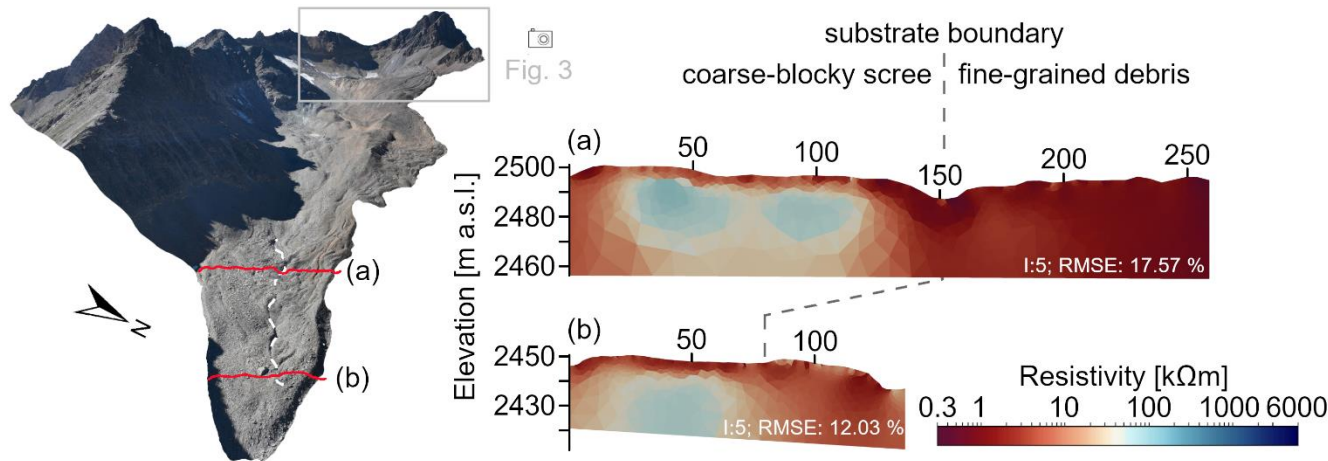
330 Figure 4: ERT surveys on the Oberferden rock glacier. Position of the substrate boundary is highlighted by the dashed white line on the rock glacier surface. Image extent of Fig. 3 is also marked for orientation by the grey box.
