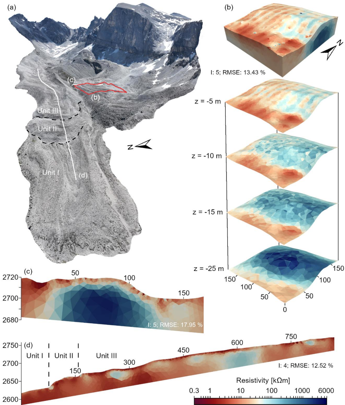
Figure 2: ERT surveys in the Pipji and Barrwang glacier forefields. An overview of the survey location is given in (a). A quasi-three-dimensional 3D ERT grid is shown in (b), whereas a two-dimensional 2D cross profile of the thrust moraine complex and a longitudinal profile along the rock glacier are shown in (c) & (d).
