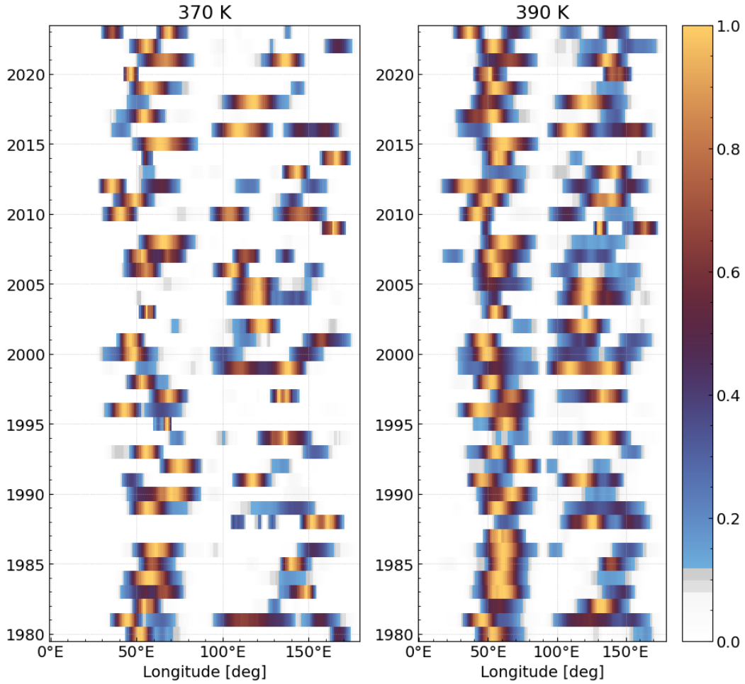
Figure 9. Mean JJA Hovmöller diagram of normalized zonal mean ( 15^{\circ}\text{N} - 45^{\circ}\text{N} ) of the residual MSF for 1980-2023 period at 370 K and 390 K. Bright colors indicate where the maximum residual MSF values tend to cluster.
