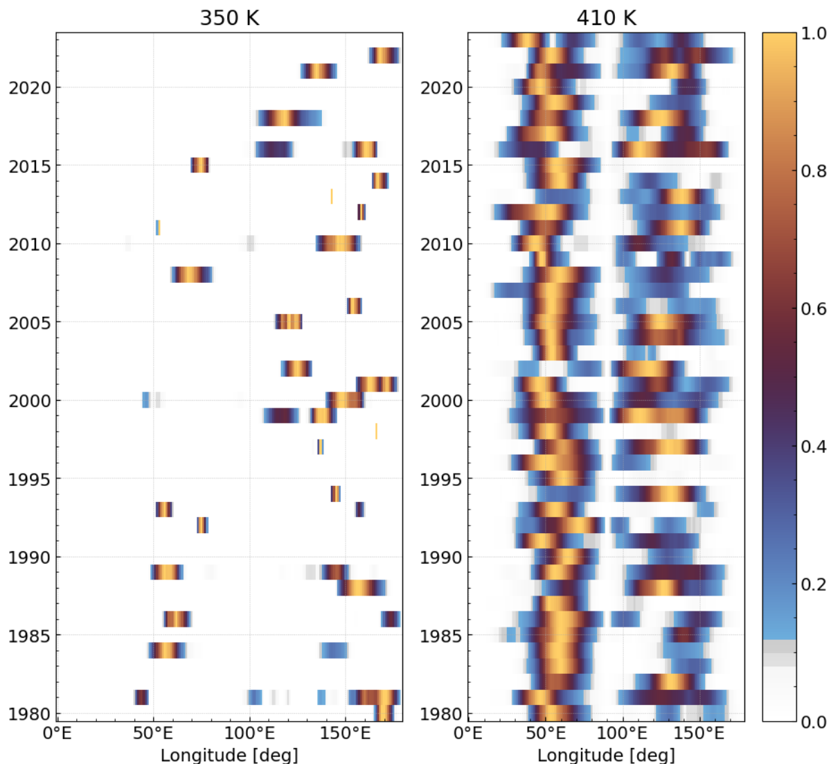
Figure E1. Mean JJA Hovmöller diagram of normalized zonal mean ( 15^{\circ}\text{N} - 45^{\circ}\text{N} ) of the residual MSF for 1980-2023 period at 350 K and 410 K. Bright colors indicate where the maximum residual MSF values tend to cluster.
