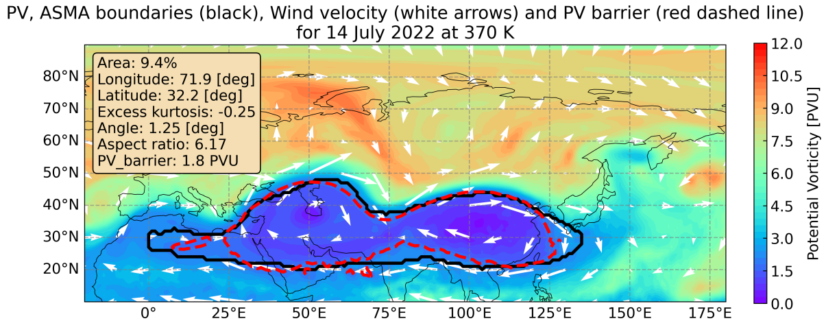
Figure 8. Horizontal plot of the ASMA boundaries (thick black line), potential vorticity color map (PV_MEAN as defined in Ploeger et al. (2015)), wind velocity (arrows), PV barrier (red dashed line), and corresponding moments quantities for 14 July 2022 at 370 K.
