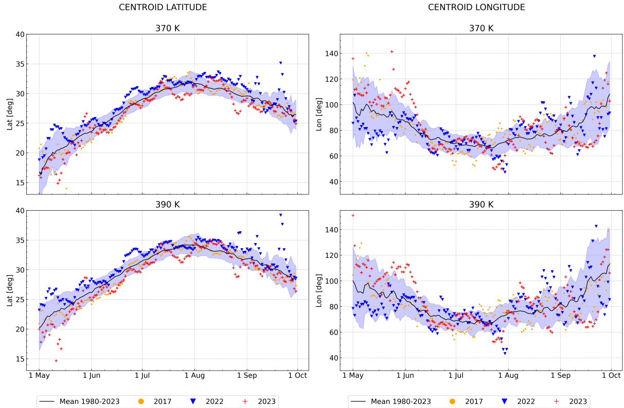
Figure 11. Climatological (1980-2023) time-series (black dotsline ) of the centroid position of the ASMA latitude (left hand side) and longitude (right hand side), and individual years of 2017 (yellow dots), 2022 (blue dotsdownward-pointing triangle ) and 2023 (red dotsplus ) at 370 K and 390 K. The lavender background denotes the standard deviation of the climatological data.
