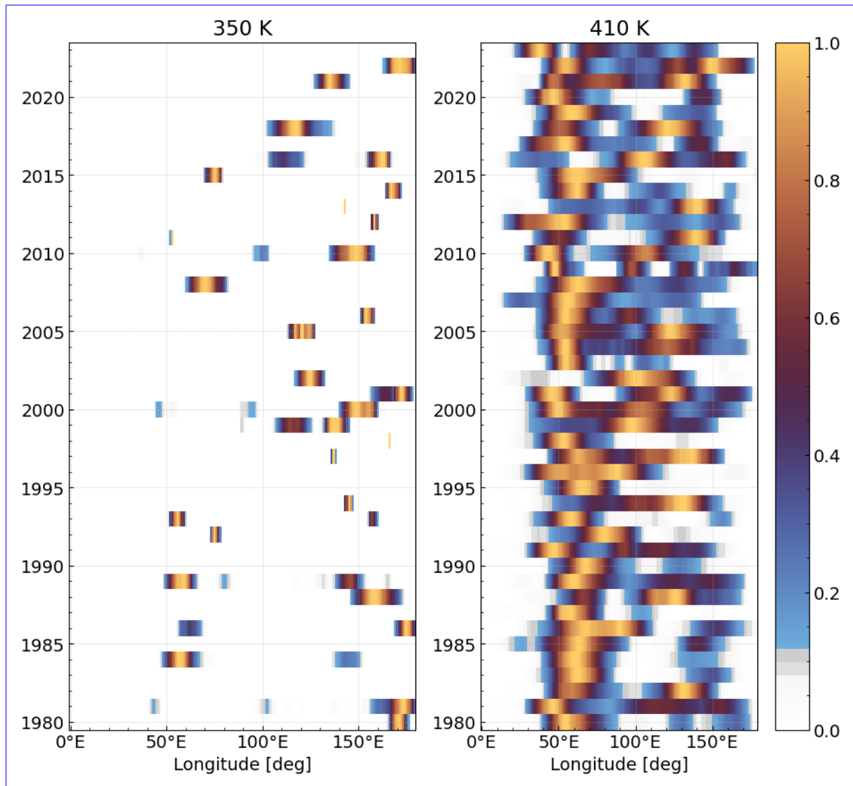
Figure E1. Mean JJA optimized background values (right) and Hovmöller diagram of normalized zonal mean ( 15^{\circ}\text{N} - 45^{\circ}\text{N} 15^{\circ}\text{N} - 45^{\circ}\text{N} ) of the residual MSF for 1980-2023 period at 350 K and 410 K . Reddish colors Bright colours indicate where the centroid longitudinal position of the ASMA tends maximum residual MSF values tend to cluster.
