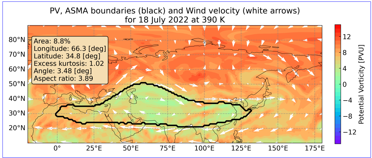
Figure 6. Horizontal plot of the ASMA boundaries (thick black line), potential vorticity (colormap), wind velocity (arrows) and corresponding moments quantities for 18.07.2022-18 July 2022 at 390 K.
