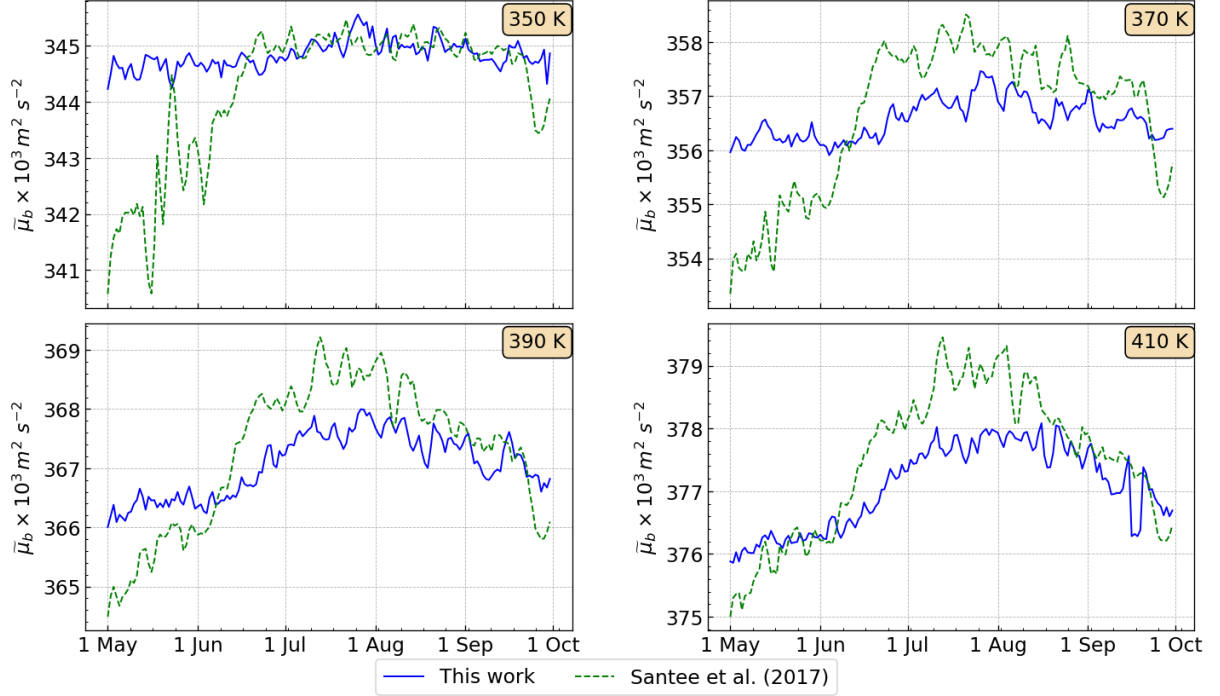
Figure 3. The Montgomery streamfunction optimized background values \widetilde{\mu}_b using our approach (blue line) \widetilde{\mu}_b and according to Santee et al. (2017) (green dashed line) \mu_b at 350, 370, 390 and 410 K for the Asian monsoon season 2023.
