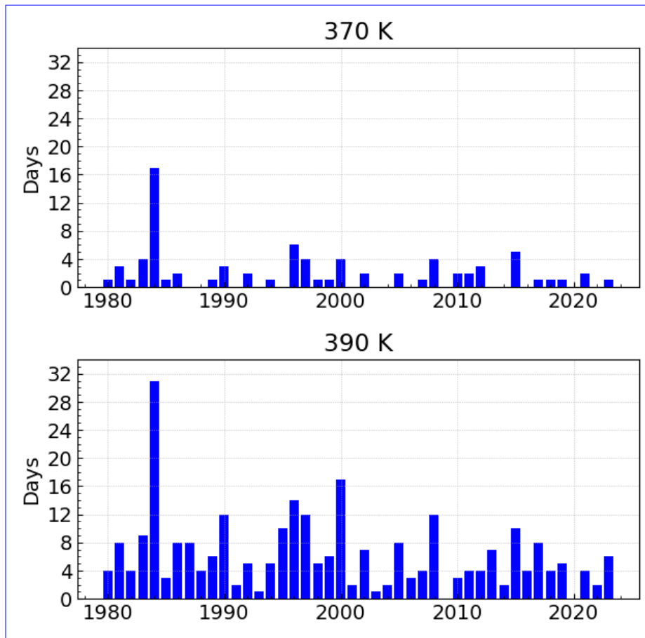
Figure 10. Number of days per year when normalized residual zonal mean R_{i,j} is above the threshold ( > 0.5 ) in both the western and eastern part at 370 K (lefttop) and 390 K (rightbottom) indicating bimodality i.e., the simultaneous existence of two parts (modes) of the ASMA. The separation line that splits the western and eastern part is defined as average centroid longitude of the ASMA for the corresponding year.
