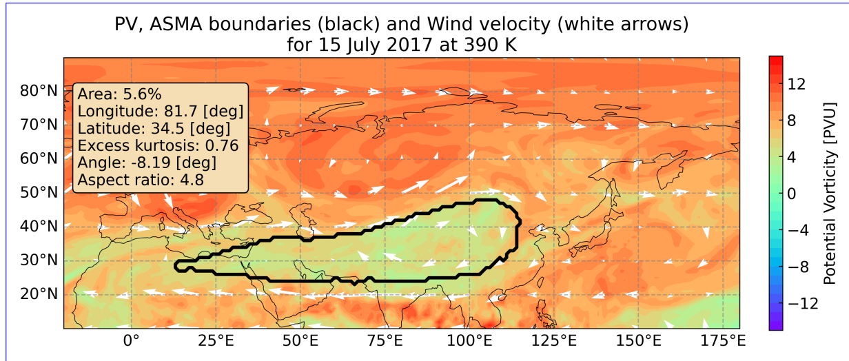
Figure 5. Horizontal plot of the ASMA boundaries (thick black line), potential vorticity ( colormap colour map ), wind velocity (arrows) and corresponding moments quantities for 15.07.2017 15 July 2017 at 390 K.
