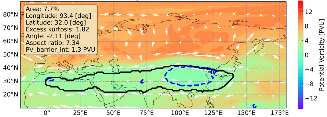
Figure C2. Horizontal plot of the ASMA boundaries (thick black line), potential vorticity colormap colour map (PV_MEAN as defined in Ploeger et al. (2015)), wind velocity (arrows), interpolated PV barrier (blue dashed line) and corresponding moments quantities for 20.08.2022 20 August 2022 at 370 K.
