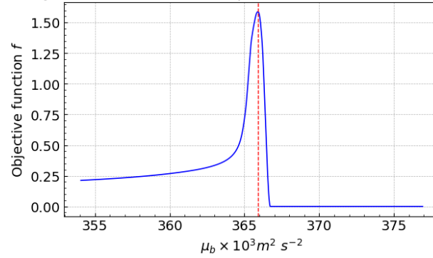
The objective function f , 06 September 2008 12:00 UTC at 390 K
