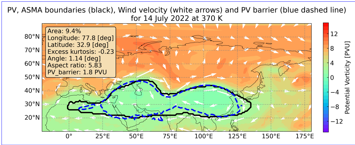
Figure 8. Horizontal plot of the ASMA boundaries (thick black line), potential vorticity colormap-colour map (PV_MEAN as defined in Ploeger et al. (2015)), wind velocity (arrows), PV barrier (blue dashed line) and corresponding moments quantities for 14.07.2022-14 July 2022 at 370 K.
