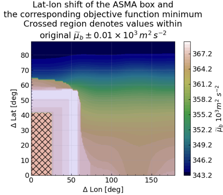
Figure B1. Sensitivity results of the latitude-longitude shift of the ASMA box and corresponding \bar{\mu}_b using the MSF values from 01.08.2023 1 August 2023 at 390 K. Crossed region highlights values within original background value \pm 0.01 \times 10^3 \text{ m}^2 \text{ s}^{-2} .
