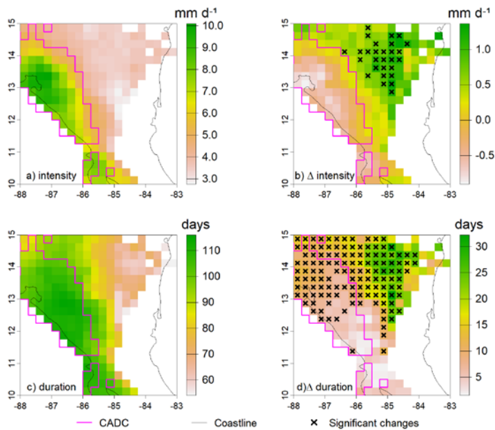
Figure 3: Historical values as simulated by the model ensemble of MSD intensity (a) and duration (c) for 1970-1999, and the projected changes (b and d) with \pm 3 °C of global warming, using the dates in Figure 2 in the MSD definition. Grid cells marked with an "X" indicate the change is significant at a 5% level based on a Wilcoxon (Mann-Whitney) test. The magenta line is the boundary of the Central America Dry Corridor (CADC), the black line denotes the coastline. Grid cells with less than 50% of years having an MSD, in both historical and future periods, are white. In addition, if less than half of the models in the ensemble show an MSD, the grid cell is white.
