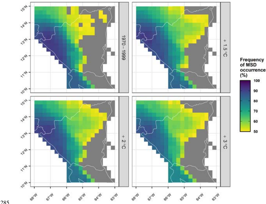
Figure 8: The frequency of MSD occurrence as a % of years for the different global warming levels depicted in Figure 7, for regions exhibiting an MSD in at least 50% of years.
