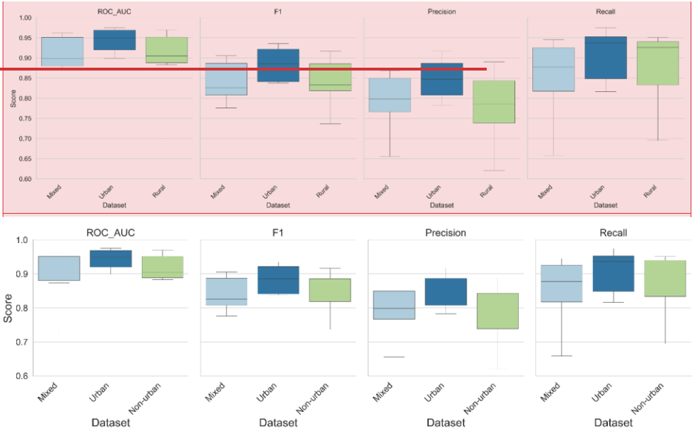
Figure 10 Comparison of model performance across different dataset configurations
