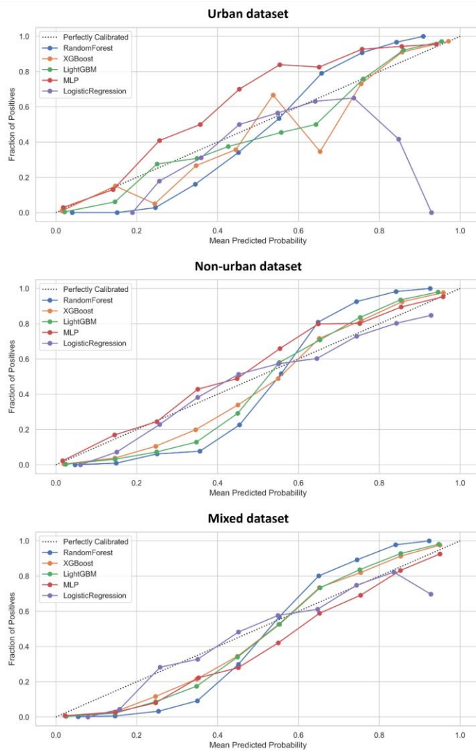
520 Figure 12 Calibration plots for each model and dataset
