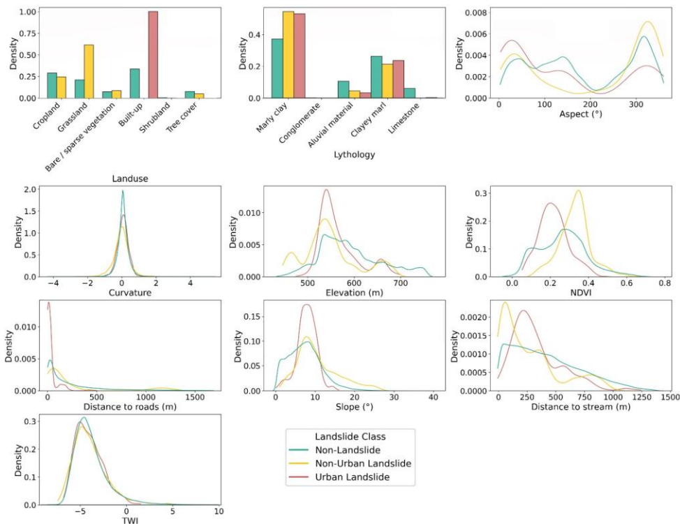
Figure 4 Density distributions of landslide conditioning factors
