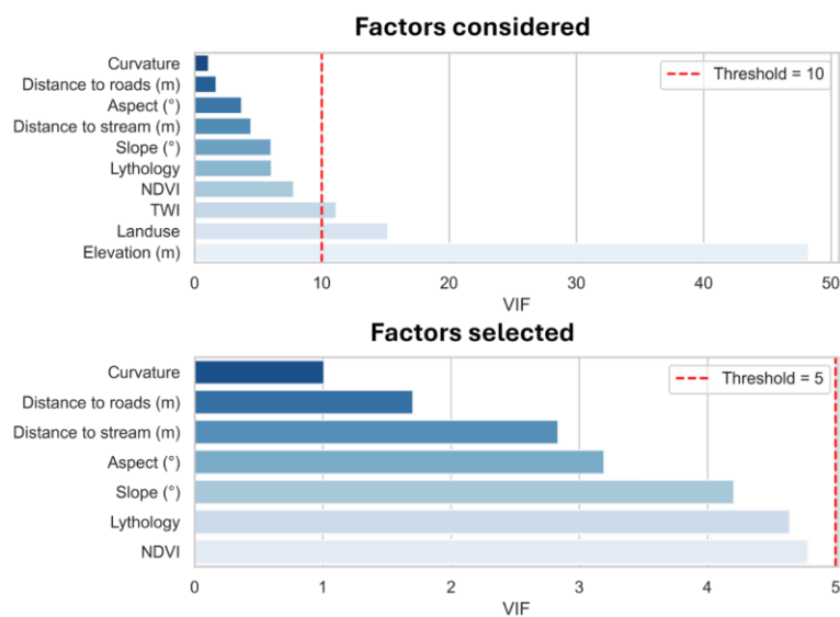
Figure 7 VIF analysis of landslide conditioning factors
