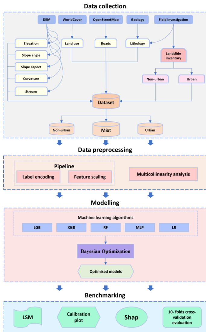
Figure 5 Flowchart of the methodology adopted
