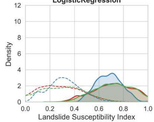
LogisticRegression
