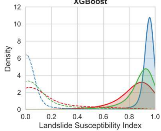
XGBoost
