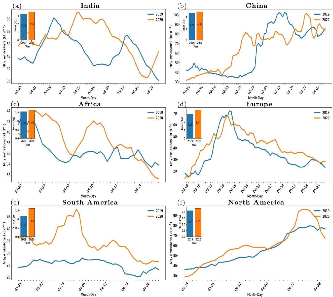
Figure 10: The timeseries of estimated daily (at 10-day scale) \text{NH}_3 emissions and total emissions (bar plots) during the COVID-19 lockdown periods in the year 2020 and pre-COVID year 2019 over different regions across the world.
