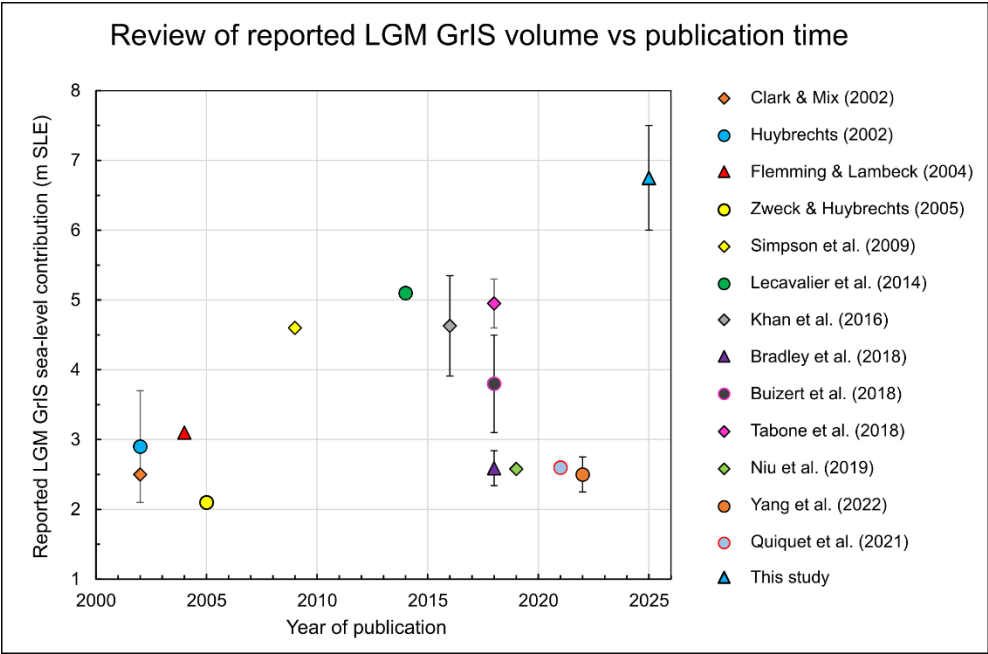
Figure 18. Review of previously modelled and/or reported GrIS volumes during the ILGM (in m SLE, expressed as ‘sea-level contribution’) plotted against year of study publication, and compared against this study’s estimates (blue triangle data point). Note that datapoints lacking error bars relate to when no range or uncertainty was reported in original studies.
