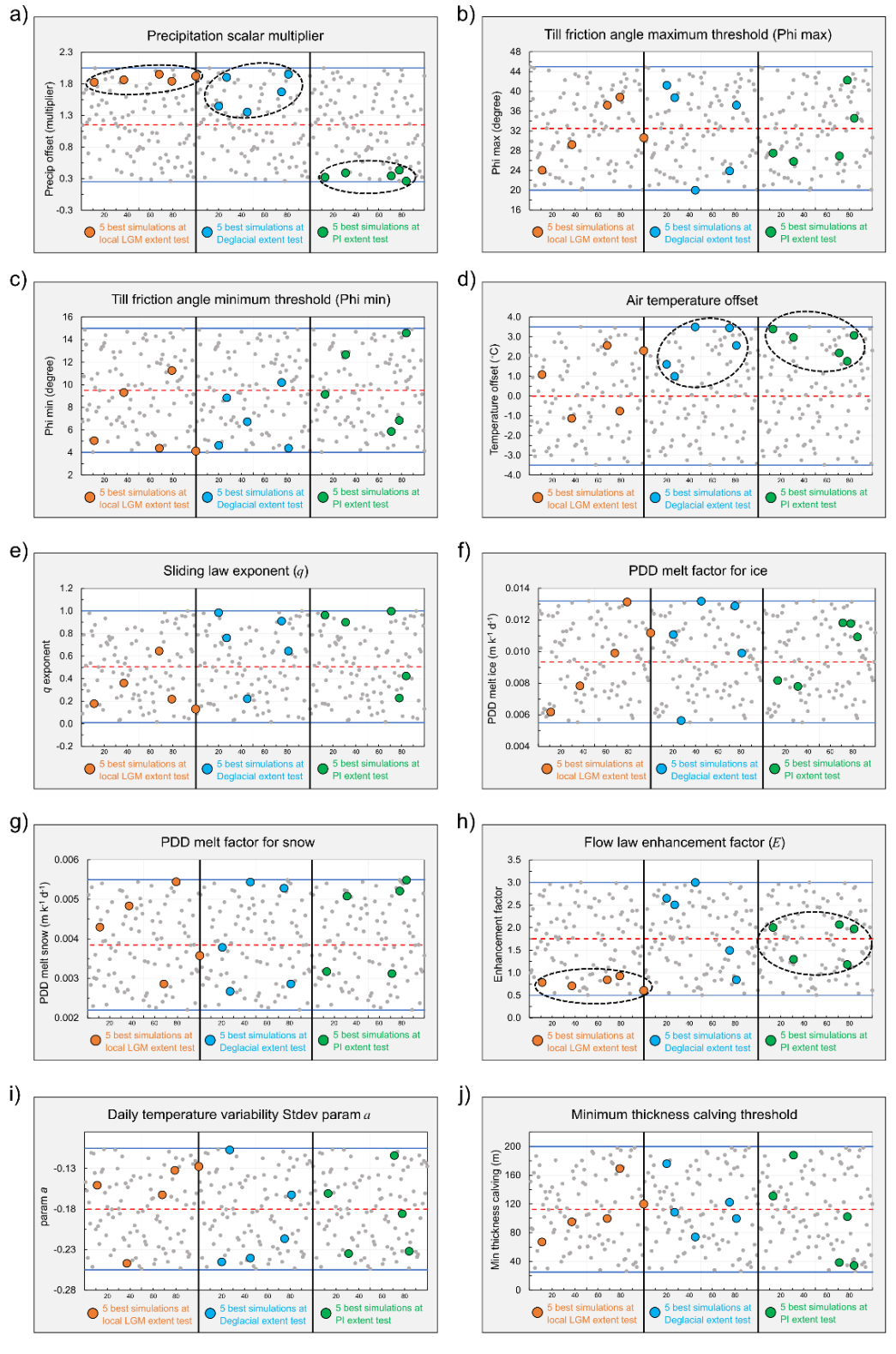
Figure 24. Values of the 10 ensemble-varying parameters for all simulations (n = 100, grey dots) and for the five best-scoring simulations (larger coloured dots) at each of the three model-data comparison tests (separated by vertical black lines). Dashed black ellipses (in panels a, d, and h) highlight best-fit parameter ‘clusters’, defined as such when the parameter values for the five best-fit simulations (coloured dots) cover a range < 50 % of the parameter value range (highlighted by horizontal blue lines) originally sampled with the Latin Hypercube technique (also see Table 1). All X axes represent ensemble simulation numbers (0 – 100).
