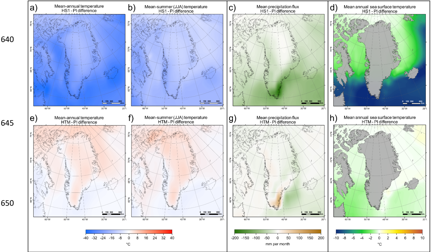
Figure 7. Fields of differences in input mean annual (panels a, e) and mean summer (JJA-mean; panels b, f) surface air temperature, precipitation rate (panels c, g), and sea-surface temperature (panels d, h) between Heinrich Stadial 1 (17.5 kyr BP: peak cooling during our simulations) and the PI era (1850 AD) for panels a-d, and between the Holocene Thermal Maximum (6 kyr BP: peak warming during our simulations) and the PI for panels e-h.
