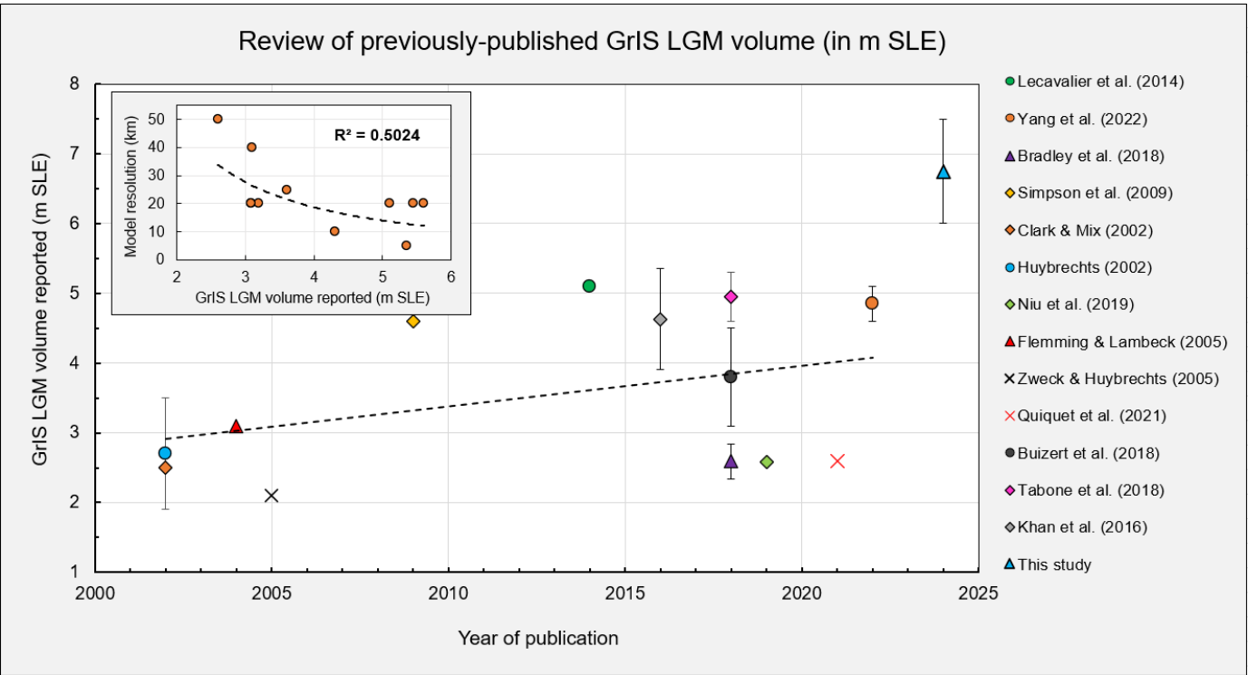
Figure 18. Review of previously modelled and/or reported GrIS volumes during the ILGM (in m SLE, expressed as ‘sea level contribution’), and compared against this study’s estimates. An increasing trend of reported values through time can be observed, along with a negative correlation between model horizontal grid resolution and reported modelled LGM volumes.
