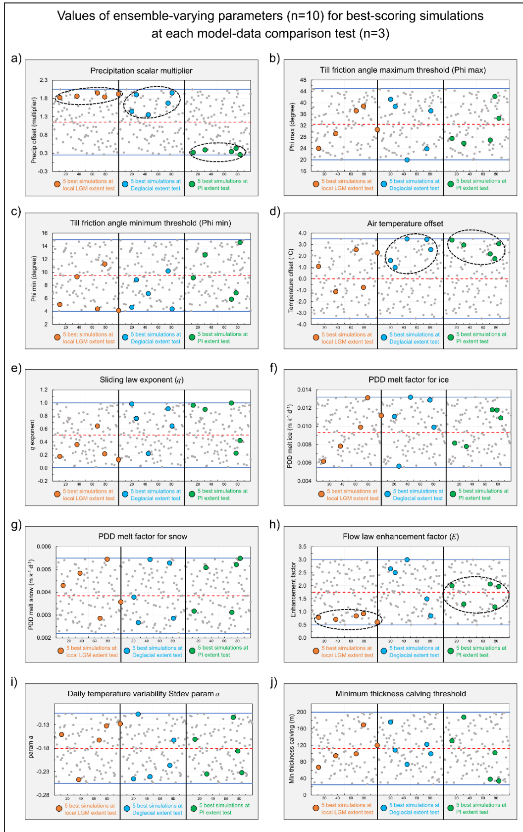
Figure 24. Values of the 10 ensemble-varying parameters for all simulations ( n = 100 , grey dots) and for the five best-scoring simulations (larger coloured dots) at each of the three model-data comparison tests (separated by vertical black lines). Dashed black ellipses (in panels a, d, and h) highlight best-fit parameter ‘clusters’, defined as such when the parameter values for the five best-fit simulations (coloured dots) cover a range < 50 % of the parameter value range (highlighted by horizontal blue lines) originally sampled with the Latin Hypercube technique (also see Table 1). All X axes represent ensemble simulation numbers (0 – 100).
