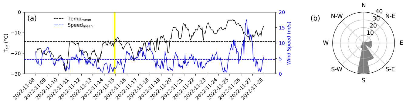
Figure A1. (a) Hourly air temperature and wind speed average during field campaign at CS test field. The vertical yellow bar indicates the UAV mission. (b) The prevailing wind directions at the CS test field during the field campaign.
