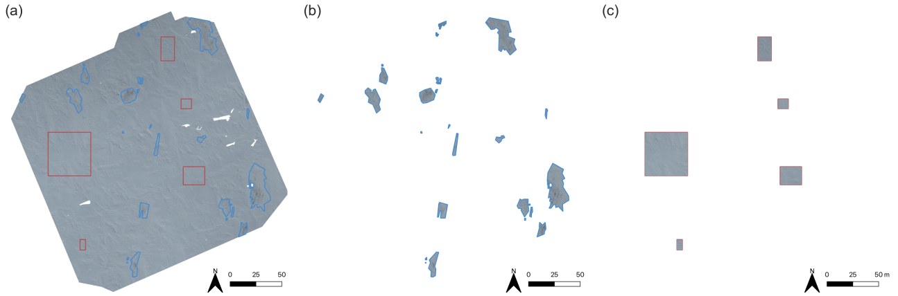
Figure A4. Masks used to create the three sub-data sets "entire field" (a), "sediment" (b) and "no sediment" (c) in the RGB orthomosaic.
