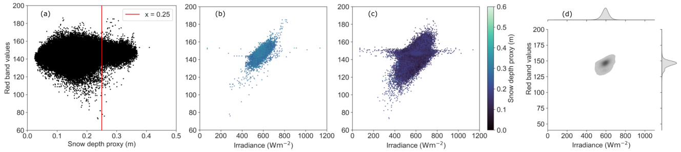
Figure A5. (a) scatter plot of red band intensity versus snow depth proxy (m) for "no sediment" sub-dataset ( r_s = 0.08 ). The red line indicates the visible cluster separation. (b) Scatter plot of red band intensity versus irradiance ( \text{Wm}^{-2} ) for "no sediment" dataset, considering only data points where the snow depth proxy exceeds 0.25 m ( r_s = 0.69 ). (c) Same as (b) but for snow depth proxy values below 0.25 m ( r_s = 0.41 ). Statistics details are provided in TableA1. These plots reveal that the horizontal cluster observed the red band intensity range of 140 to 160 disappears when considering only snow depth proxy values is connected to the snow depth as it disappears when considering only snow depth proxy values above 0.25 m, indicating a connection to snow depth. For snow depth proxy values below 0.25 m, the entire irradiance range is present, suggesting a link to topography. However, the red band intensity shows no direct dependence on the snow depth proxy, and a more detailed analysis is beyond the scope of this study. (d) Highlights that the horizontal extent of the cluster corresponds to a region with low data density.
