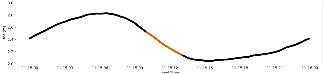
Figure A6. Tidal movements (m) at the Scott Base tidal gauge from the sea level recorder (nitrogen bubbler system with a paroscientific pressure transducer located on a bottom-mounted spigot of the osmosis boom and barometer). The data is recorded in 5 minute intervals. The orange part of the plot marks the flight survey.
