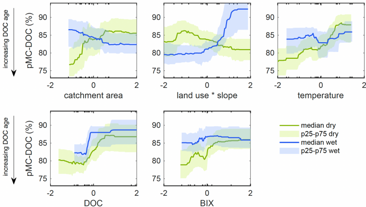
Figure 4. Partial dependence plots of the marginal effects of each predictor on 14 C-DOC based on the best GAMs developed for the dry and wet seasons. All predictors were standardised prior to analysis, so that negative values on the x-axes indicate below-mean values, while positive values indicate above-mean values. The small dashes on the horizontal axes indicate the distribution of predictor values and are duplicated on both axes. Note: higher pMC-DOC corresponds to lower DOC age.
