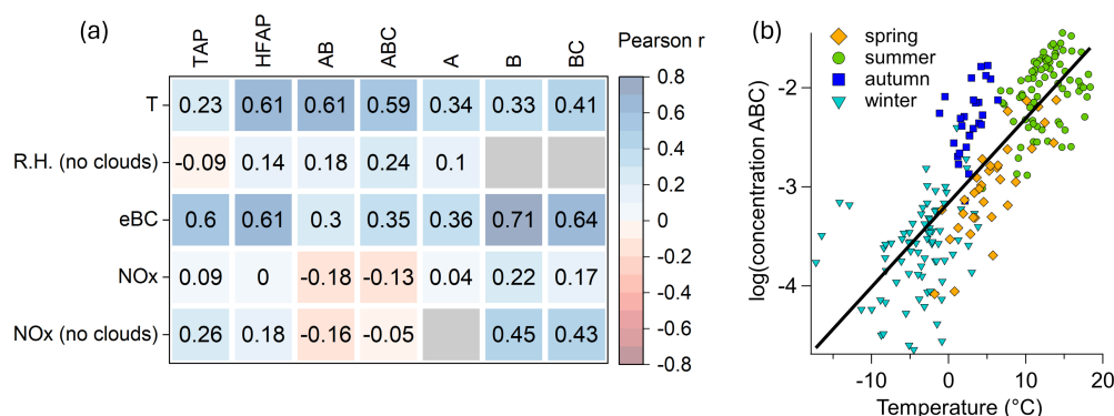
Figure 5. Relation of concentration of particles types to meteorological parameters and air pollution. (a) Pearson correlation coefficient matrix of 1 hour-h mean values. Grey (empty) relations do not reach the 95 % confidence level. (b) scatter plot of the common logarithm of daily mean ABC particles against ambient temperature ( r = 0.82 ). The transition between snow free and snow-covered periods (e.g., from autumn to winter) is less apparent than in Fig. 3 (b), as the temporal context is lost and ABC particles remain present to varying extents throughout the winter.
