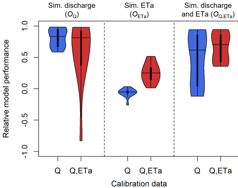
270 Figure 2: Model performance for simulated discharge ( O_Q ), actual evapotranspiration ( O_{ETa} ), and discharge and actual evapotranspiration ( O_{Q,ETa} ) when using discharge (Q; blue boxes), or both discharge and actual evapotranspiration (Q, ETa; red boxes) as calibration data. The figure shows the median of the 100 best performing parameter values of each catchment. To present results for all twelve study catchments, performance values were normalized by an upper benchmark (equal to 1) and a lower benchmark (equal to the median performance of the uncalibrated model). A value of zero means that model performance after calibration is equal to the model performance of the lower benchmark.
