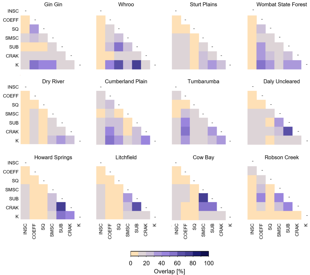
345 Figure 6: Overlap of the two point clouds of behavioural parameter sets for a given parameter pair when calibrating the model solely to discharge ( O_Q ) and solely to actual evapotranspiration ( O_{ETa} ). The orange squares show the parameter combinations with a lack of overlap in the two-dimensional space. Values range from 0 to 100% of the total area of the normalized parameter space (as visualized in Fig. 5).
