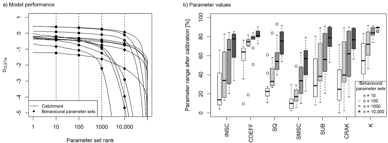
425 Figure 8: Definition of behavioural parameter sets and its impact on a) model performance O_{Q,Et\alpha} and b) parameter values, i.e., 430 ratio of the range of parameter values after calibration with O_{Q,Et\alpha} relative to the range of possible parameter values before 435 calibration (see Fig. S1 for an explanation of the parameters). Results are shown for all twelve study catchments.
