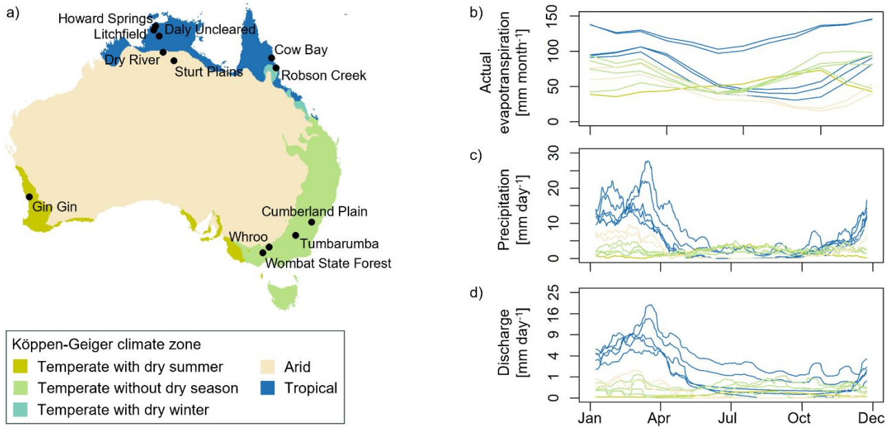
180 Figure 1. Location and characteristics of the twelve study catchments. (a) Location and Köppen-Geiger climate zone (Peel et al., 2007) of the study catchments. (b-d) Regime curves for actual evapotranspiration (remote-sensing based data), precipitation, and discharge. The regime curve is calculated as the mean value at each day of the year using the hydrological years 2004-2013. Regime curves were smoothed with a fifteen-day moving average.
