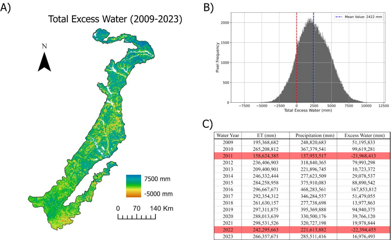
325 Figure 10. (A) Spatial distribution of total excess water (mm/m 2 ) across the Post Oak Savannah ecoregion from 2009 to 2023. The amounts range from −5000 mm/m 2 to 7500 mm/m 2 . (B) Frequency distribution of total excess water across the ecoregion, with red and blue dashed lines indicating 0 total excess water and the mean, respectively. (C) Annual summary of ET, P, and resulting excess water (mm). Negative values in the table (highlighted) indicate water years having net water deficits.
