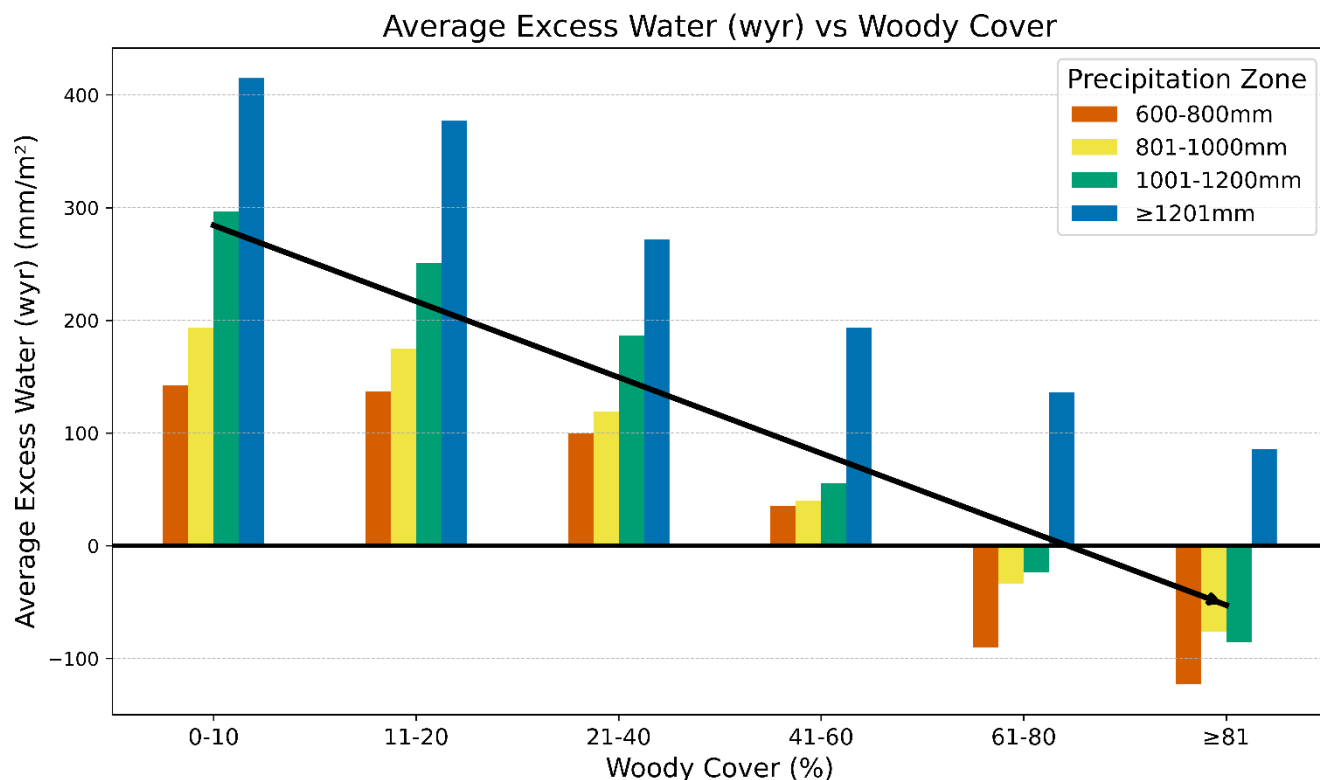
Figure 11. Mean annual excess water (mm/m 2 ) as a function of woody cover (%) and precipitation zone. The black trend line indicates the overall decrease in excess water with rising woody cover. Positive values represent net surpluses, whereas negative values denote net deficits.
