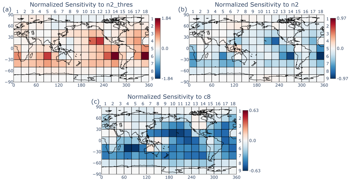
Figure 10. Map of normalized sensitivity, S_j^+ , of a) n2\_thres , b) n2 , c) c8 . The spatial pattern of SVD 1 (Fig. 8) resembles the sensitivity of two of its strongest components, n2\_thresh and n2 , but not c8 , despite c8 's importance (Fig. 9).
