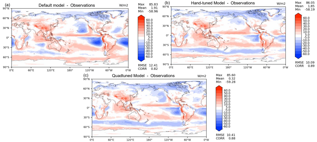
Figure 2. Biases of SWCF in various versions of EAM-taus: (a) default (untuned), (b) hand-tuned, and (c) quad-tuned . Without tuning, the stratocumuli in EAM-taus are too bright. These biases can be reduced almost as much by automated quad-tuning (c) as they can by laborious hand-tuning (b).
