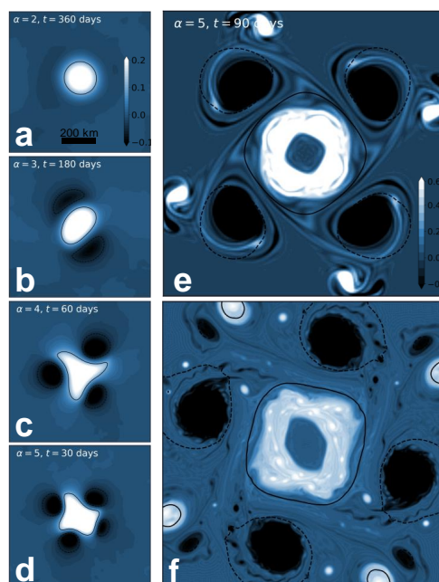
Figure B1. Eddy stability numerical simulations. (a–d) Snapshots of the upper-layer streamfunction from low-resolution two-layer Quasi-Geostrophic (QG) simulations, initialized with \alpha = [2, 3, 4, 5] . (e) Upper-layer vorticity snapshot from a high-resolution two-layer QG simulation, using the same parameters as in (d); dashed and solid contours show -0.05 and 0.1 streamfunction contours, respectively. (f) Surface vorticity snapshot from a high-resolution Surface Quasi-Geostrophic (SQG) simulation, also using the same parameters as in (d).
