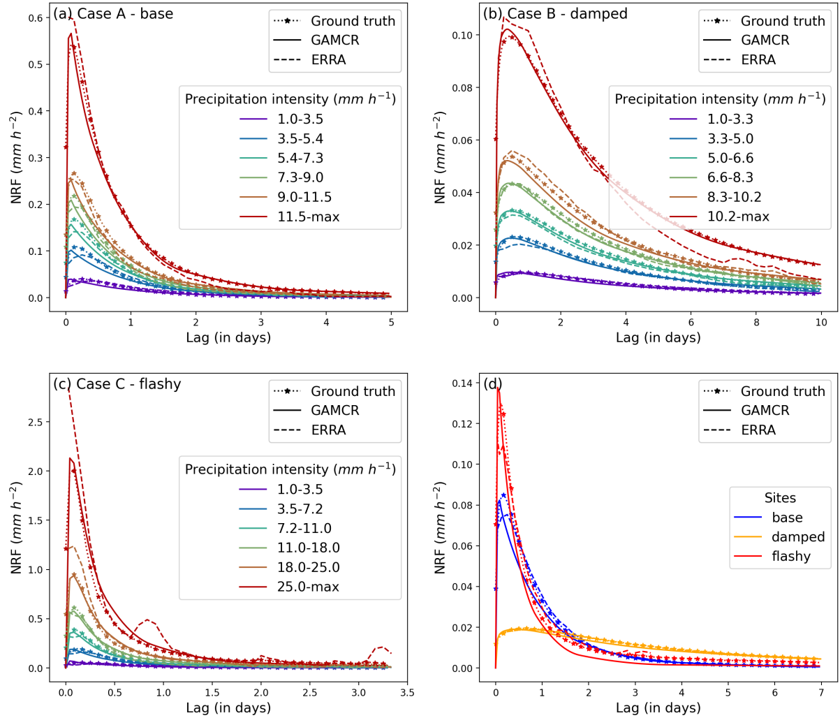
Figure 6. NRFs averaged across different precipitation intensity ensembles from GAMCR, ERRA and the ground truth, for the base (a), damped (b), and flashy (c) synthetic time series. Readers should note the different scales of NRFs between flashy, base and damped scenarios. Panel (d) combines the overall average NRFs for the three cases in a single plot .
