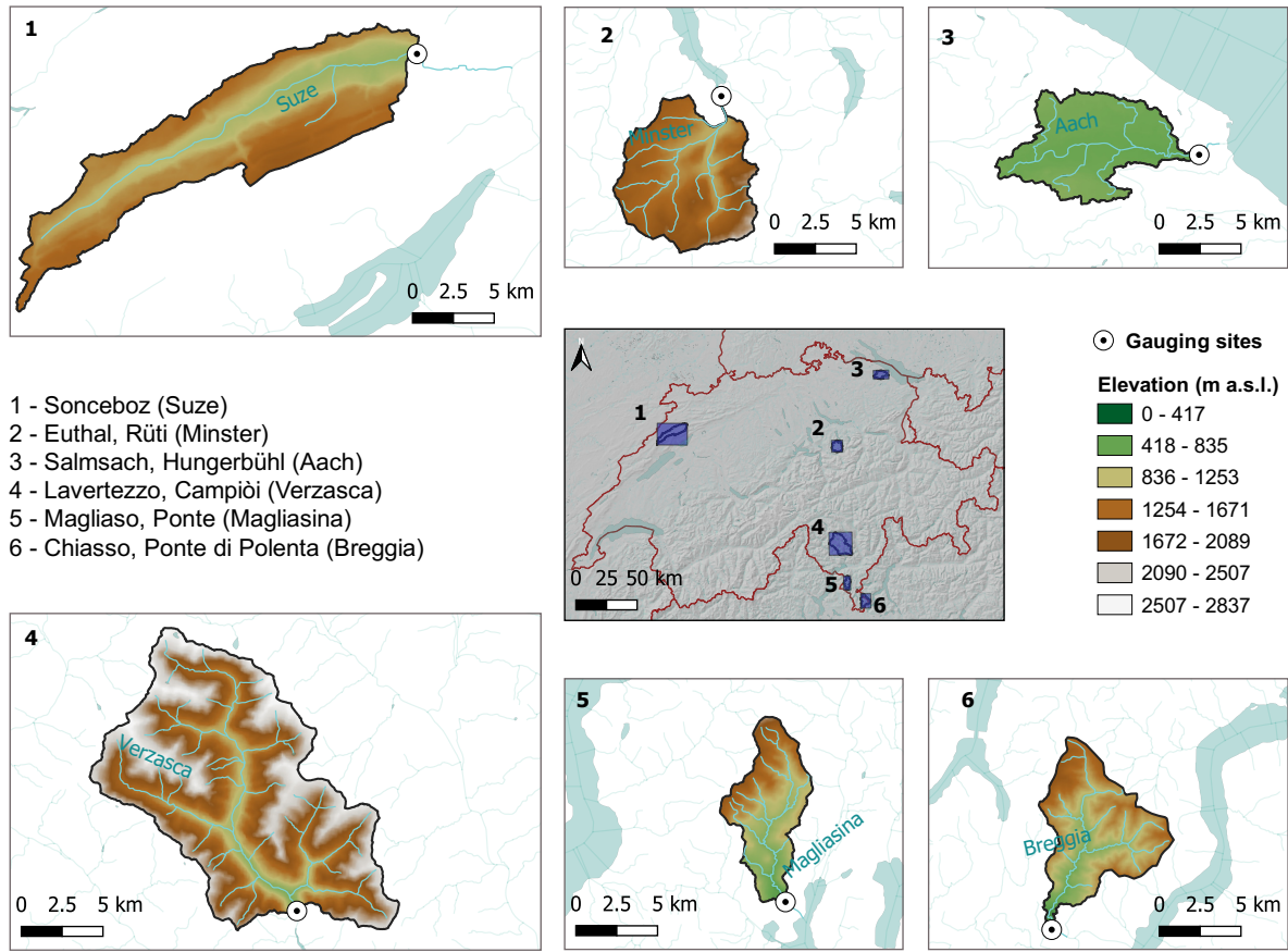
Figure 3. Map of Switzerland showing the six catchments analyzed, along with their corresponding gauging stations (listed on the left with the river names in brackets). Each catchment is displayed in a separate plot for a detailed view of its dimensions and elevation ranges. Numbers mark the catchments' locations within Switzerland and can be seen on the map in the center. The sixth gauging station (Chiasso, Ponte di Polenta) also provided the streamflow time series used to create the synthetic dataset with precipitation data from Lugano.
