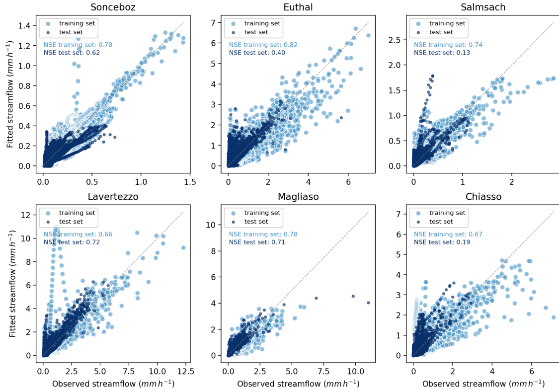
Figure 8. Fitted streamflow estimated through GAMCR for the six investigated sites. The larger light blue dots show measured and fitted discharges during the 2005–2017 snow-free seasons (training set); The smaller dark blue dots indicate measured and predicted discharges during 2018 and 2019 snow-free seasons (test set). 1:1 lines are shown in grey.
