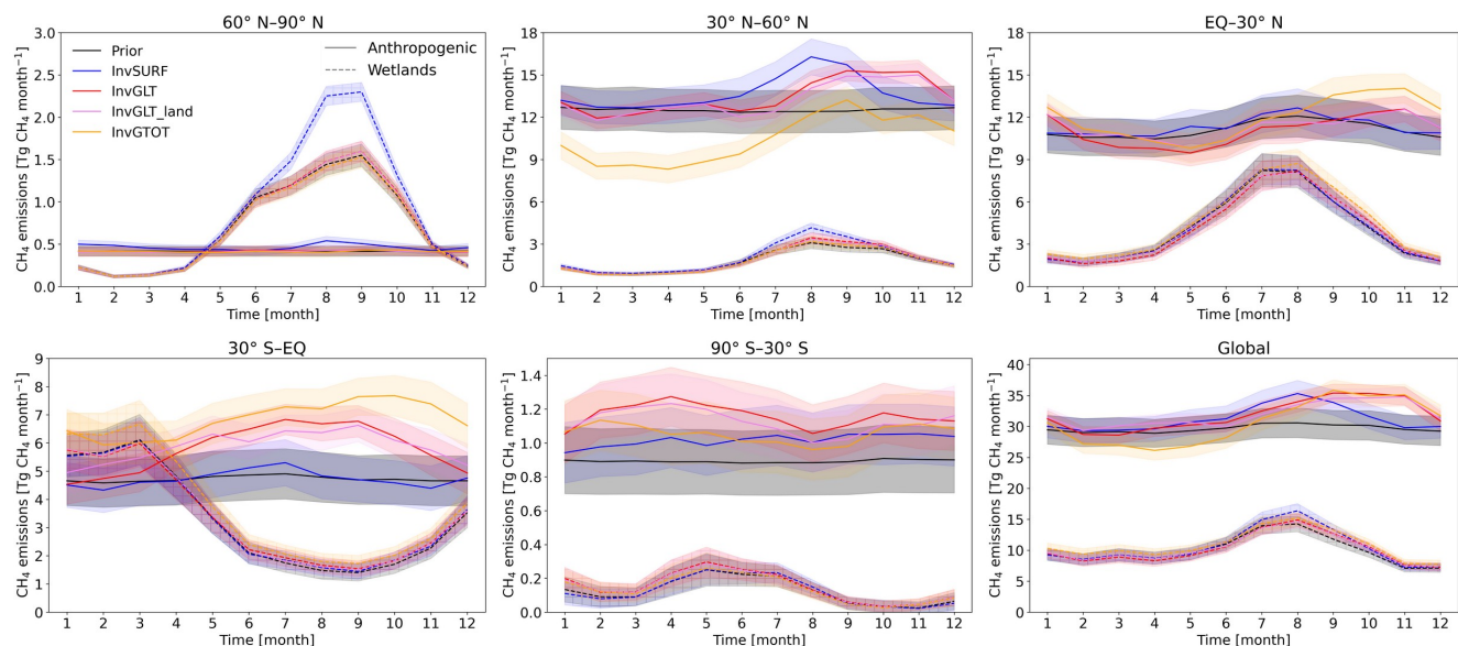
Figure 5. Monthly mean anthropogenic and wetland \text{CH}_4 emissions at 30° latitudinal bands and global totals. The means are taken from 2016–2019. Shaded areas illustrate uncertainty as standard deviations of 500 ensemble members.
