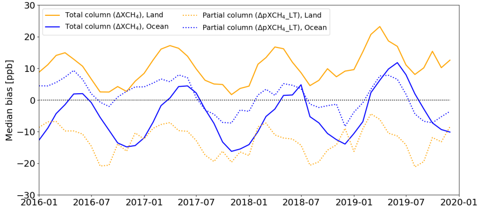
Figure 3. Global monthly median differences between posterior InvSURF and JAXA/GOSAT retrievals. Positive values indicate posterior InvSURF mole fractions being higher than the JAXA/GOSAT retrievals.
