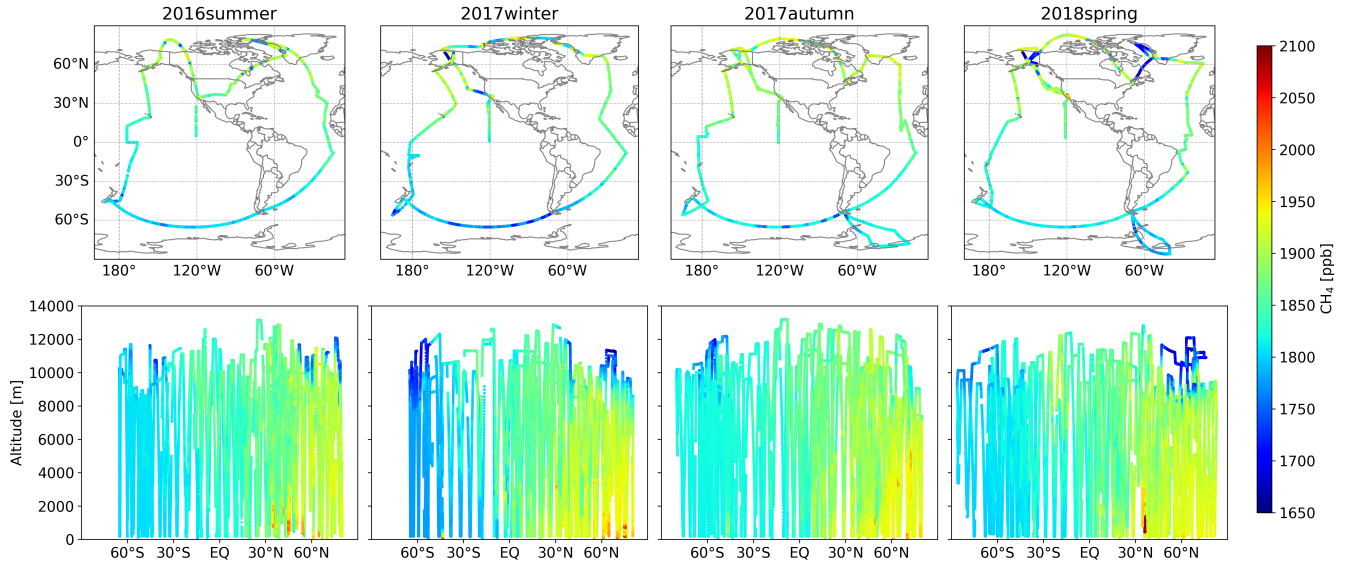
Figure A7. Observed \text{CH}_4 mole fractions from aircraft measurements of Atmospheric Tomography Mission during the study period.
