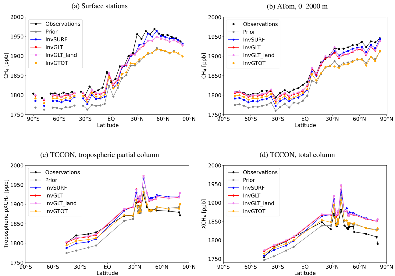
Figure 4. Mean atmospheric \text{CH}_4 , averaged over 2016–2019 at (a) surface ground-based and shipboard stations, (b) ATom observation locations, and (c) and (d) TCCON sites. For (a), the data that were assimilated in InvSURF were used. For (a) and (b), mean over five-degree latitude bands are shown. For (c) and (d), no spatial averaging is applied. The coloured lines are the posterior estimates from each inversion, which is estimated by running TM5 forward using posterior fluxes of the corresponding inversion simulation.
