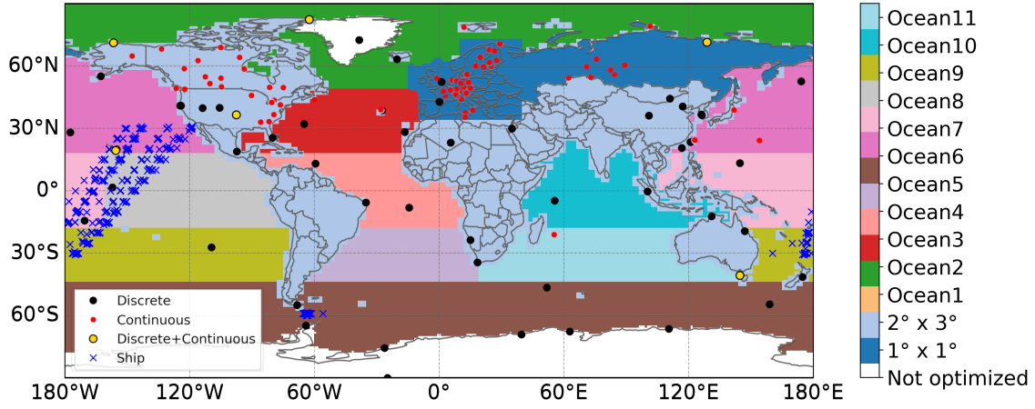
Figure A1. Location of ground-based surface observations (dots and x-marks) assimilated in the InvSURF inversion experiment (see section 2.4), and optimization regions used in CTE-CH 4 (background colours). Over land areas, the fluxes were optimized grid-wise, and ocean region-wise.
