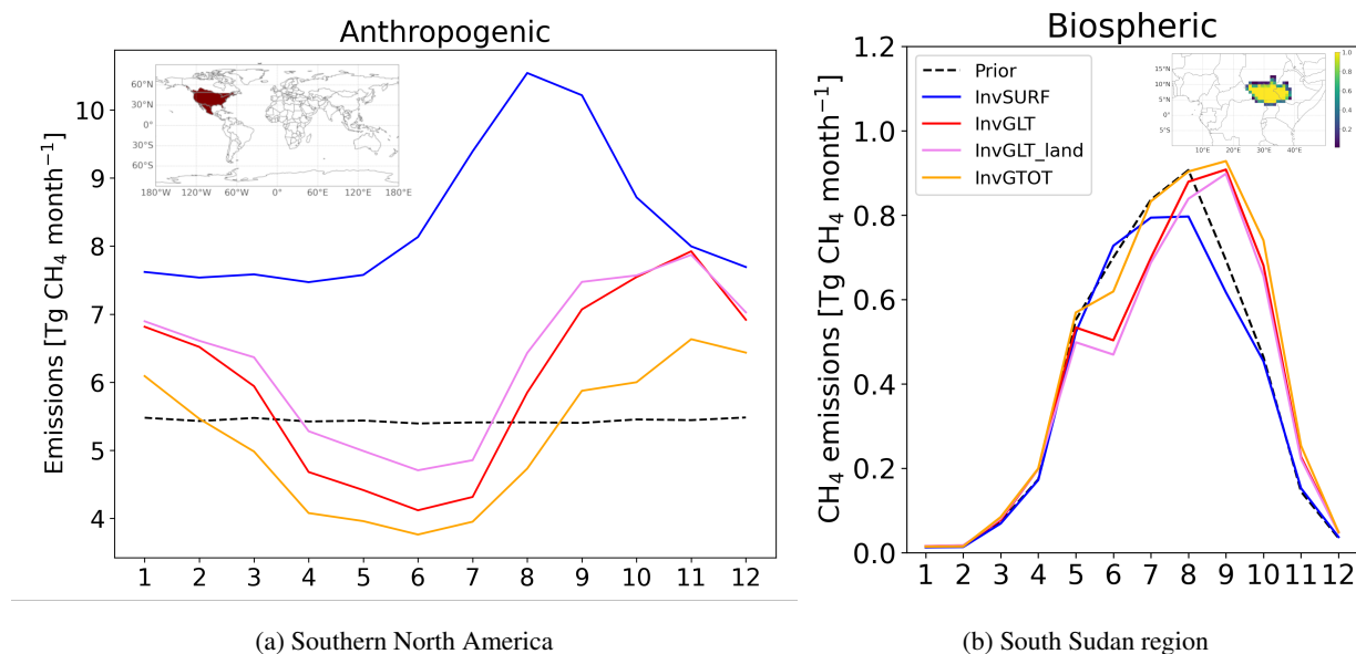
Figure A10. Average monthly CH 4 emissions in (a) southern North America and (b) South Sudan regions. The maps illustrate aggregated areas.
