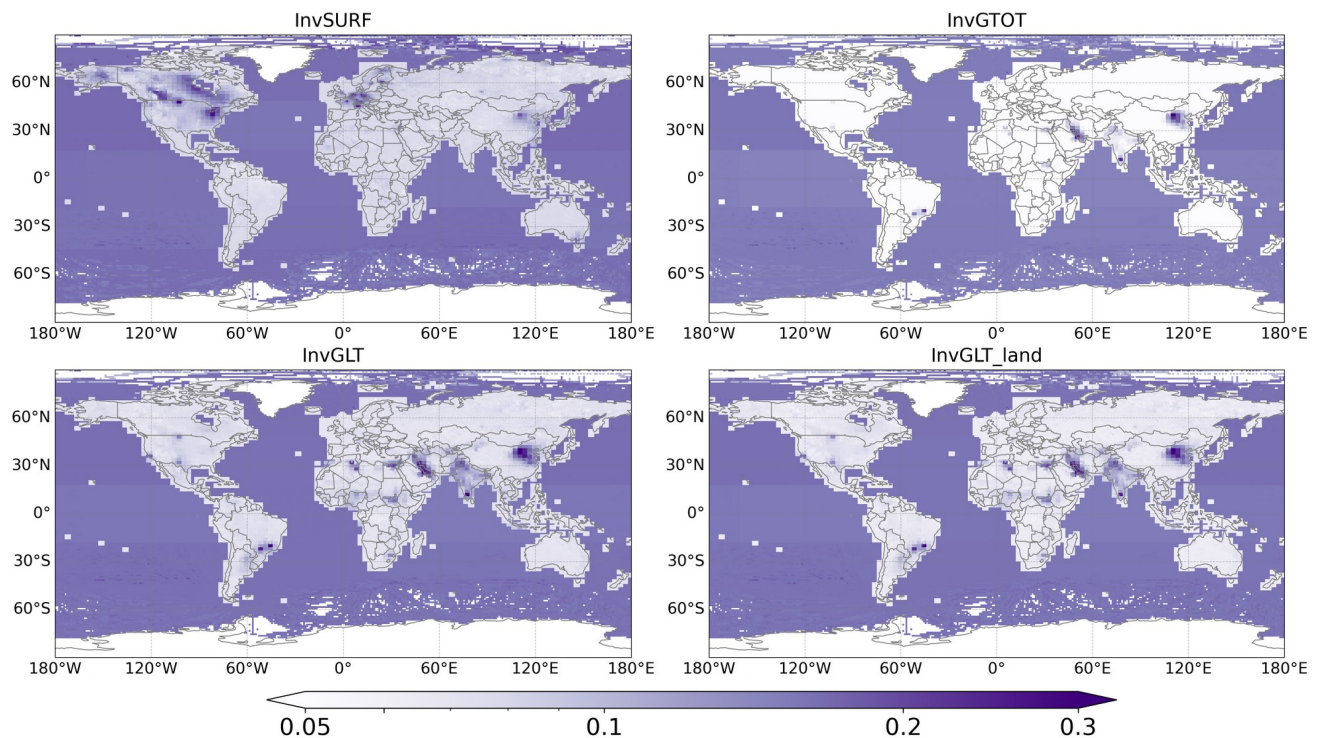
Figure 7. Annual mean uncertainty reduction rate (\sigma_{\text{prior}} - \sigma_{\text{posterior}})/\sigma_{\text{prior}} of total fluxes, averaged over 2016–2019. \sigma were calculated as standard deviation from 500 ensemble members. Note the colour is in logarithmic scale.
