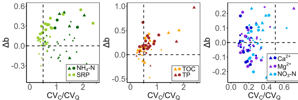
Figure 5: Change in cQ-relationships ( \Delta b ) for SRP, \text{NH}_4\text{-N} , TP, TOC, \text{NO}_3\text{-N} , \text{Mg}^{2+} , and \text{Ca}^{2+} explained by climate-changing climatic conditions. Positive \Delta b values indicate an increasing enrichment behaviour. \blacktriangle represent catchments exhibiting enrichment
