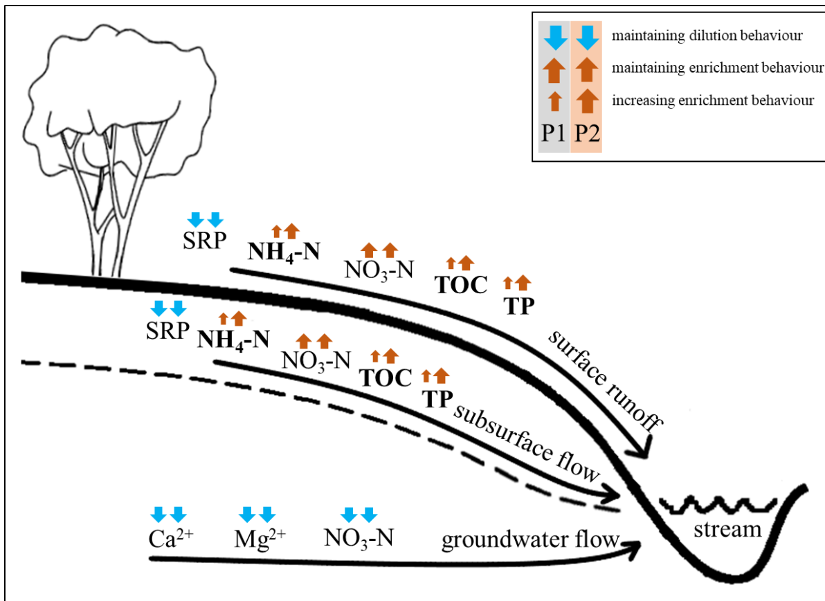
520 Figure 6: Illustration of mobilization and transportation pathways for nutrients and geogenic minerals. Change in SEM based on climate change changing climatic conditions illustrated by direction and size of the arrows. P1 – period 1 (onwards 1 st Jan. 2012) less affected by climate change . P2 – period 2 (after 1st Jan 2012) more affected by climate change (modified illustration Jordan et al. 1997).
