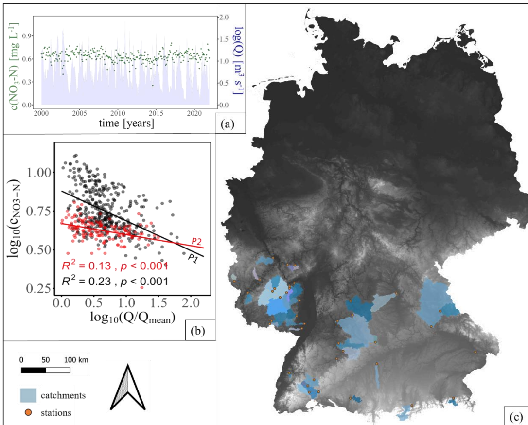
110 Figure 1: (a) Time series of discharge and nitrate (NO 3 -N) in the Fils catchment. (b) cQ-relationships for NO 3 -N in the Fils catchment, showing for period 1 (black, P1) and period 2 (red, P2—heightened presence of climate change effects). Differences between P1 and P2 were tested by ANCOVA (p<0.05) for each catchment (illustrated here for catchment Fils, p<0.001). (c) Study area in Southwest Germany with 40 catchments. Map of catchments with measuring stations (orange), with a black-white gradient indicating elevation (BKG, 2013). Map projection: UTM (EPSG: 25832).
