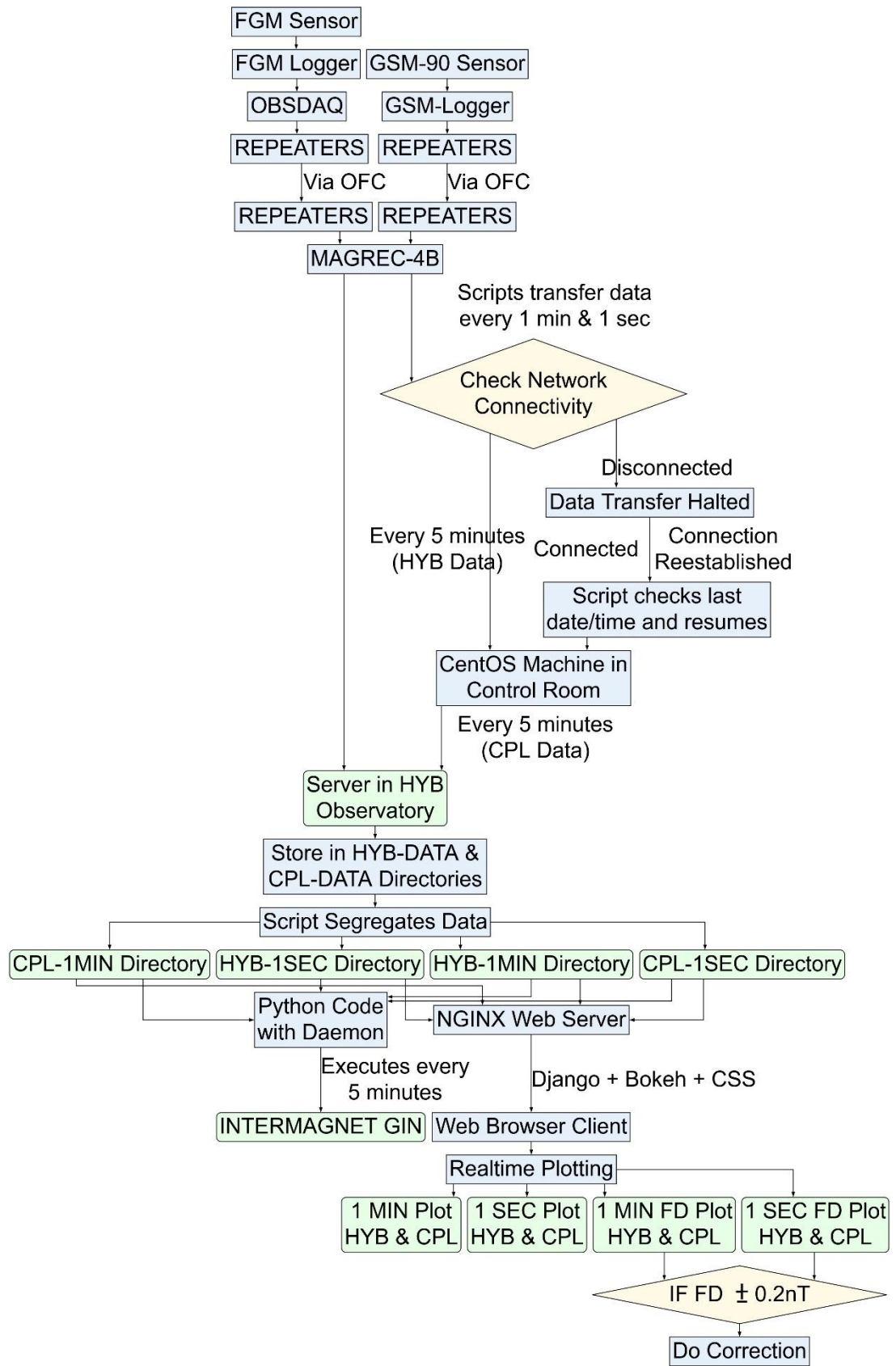
Figure 2. Schematic diagram of the processes involved in the automated quality control and data transfer pipeline for the HYB and CPL observatories
