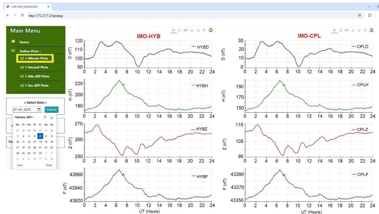
Figure 32: Real-time plotting of Vector and Scalar data at 1 min sampling interval from the HYB (left) and CPL (right) observatories of CSIR-NGRI, with the updated services in the server.
