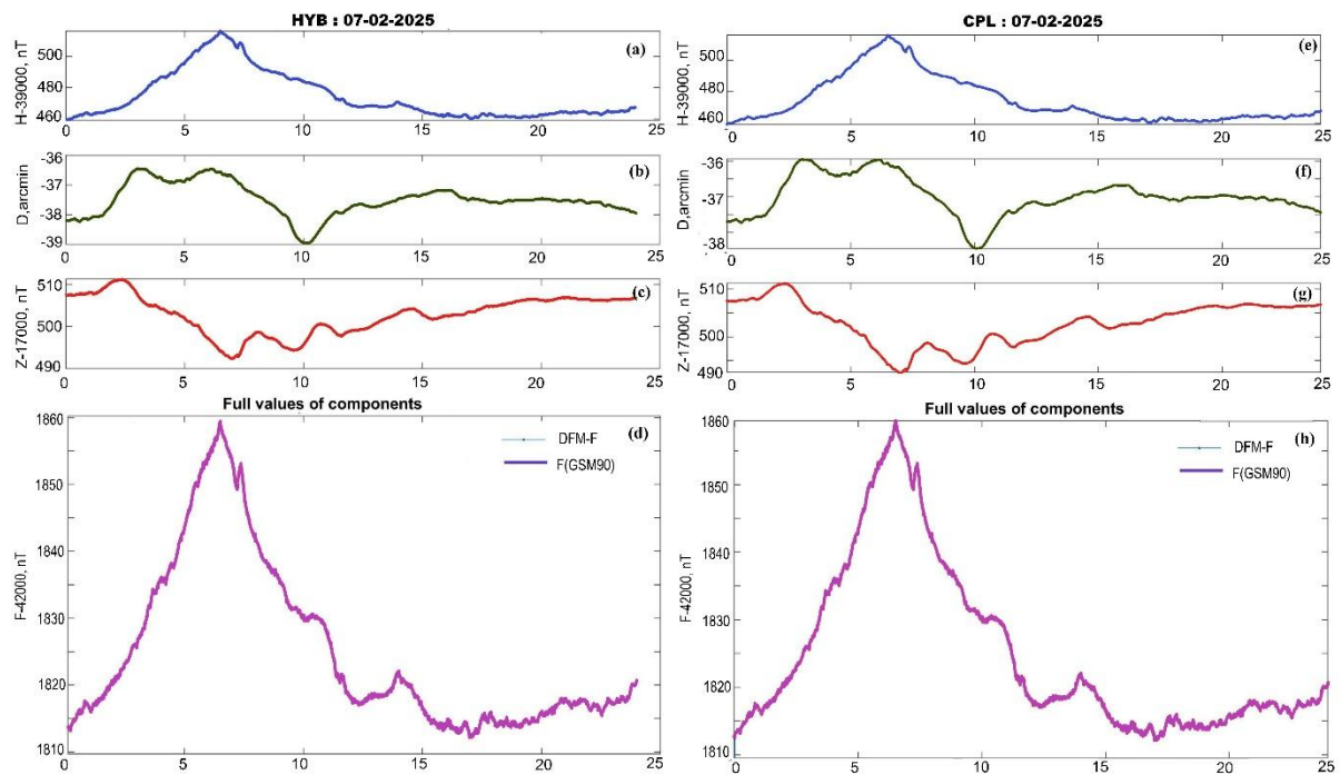
Figure 67: 1 min vector and scalar data from the HYB (left) and CPL (right) observatories after removing spikes identified through real-time first differences.
