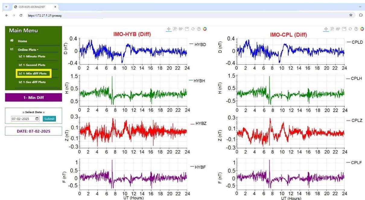
Figure 45: Real-time plotting of the first differences of vector and scalar data, sampled every minute from the HYB (left) and CPL (right) observatories
