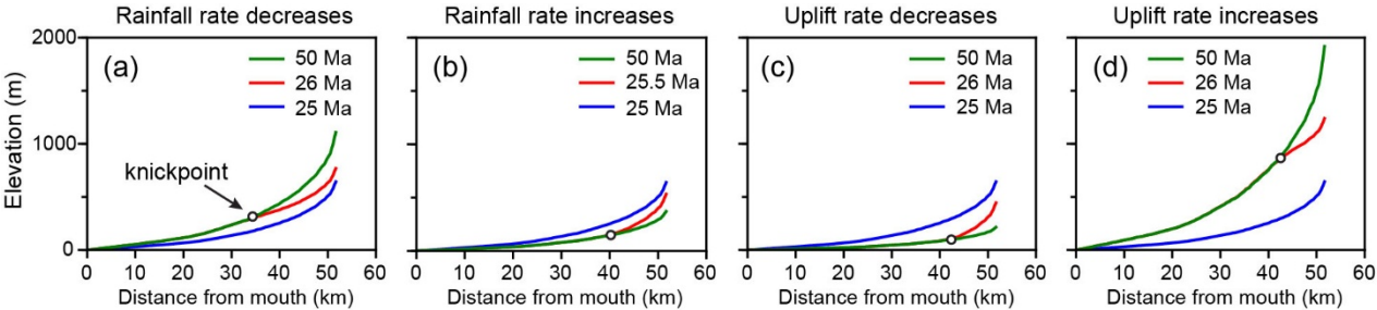
200 Figure 4. Longitudinal profiles of the trunk stream after changes in rainfall or uplift rates in model M1 (no hillslope diffusion). The changes occur at 25 Ma, affecting the steady state trunk stream in blue.
