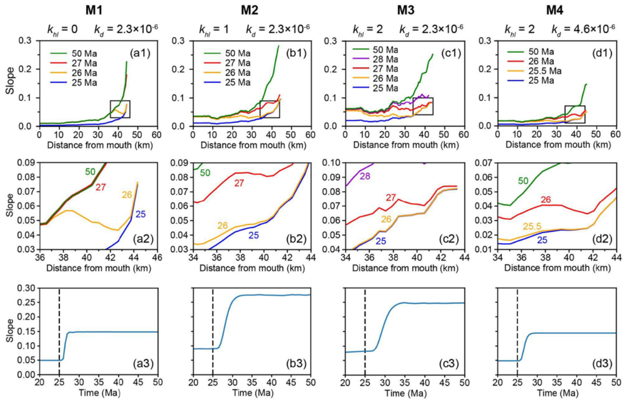
205 Figure 5. Evolution of trunk stream slope following an increase in uplift rate. (a1-d1) Longitudinal slope profiles of the trunk stream at selected time steps (colored lines), with each subplot corresponding to a model (M1-M4). Black rectangles indicate the headwater regions. (a2-d2) Enlarged views of the headwater areas, corresponding to the boxed regions in (a1-d1). (a3-d3) Temporal evolution of the mean channel slope in the upper ~800 m of the trunk stream, capturing the dynamic slope response across model runs. Dashed vertical lines mark the timing of the uplift rate increase (25 Ma).
