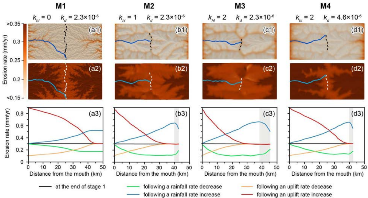
255 Figure 7. Erosion rates (mm/yr) per grid cell, calculated over 1 Myr following (a1-d1) a decrease in rainfall rate and (a2-d2) an increase in uplift rate. Blue lines in (a1-d1) and (a2-d2) represent trunk streams, and dashed lines mark divides. (a3-d3) Longitudinal erosion profiles along trunk streams, with grey bands indicating the regions where the transient slope change reversal occurs.
