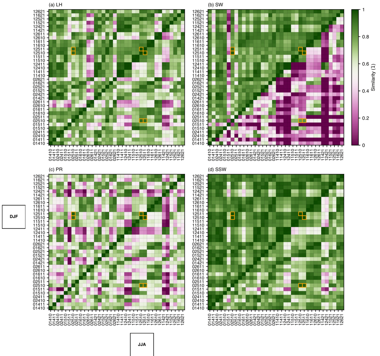
775 Figure C1: Pairwise spatial similarity indices across the 36 experiments and two seasons. Similarity indices are applied to DJF (JJA) patterns in the upper-left (lower-right) section of each subplot. The cells corresponding to the three pairs one can constitute with 12511, 12510 and 02510 are framed in orange.
