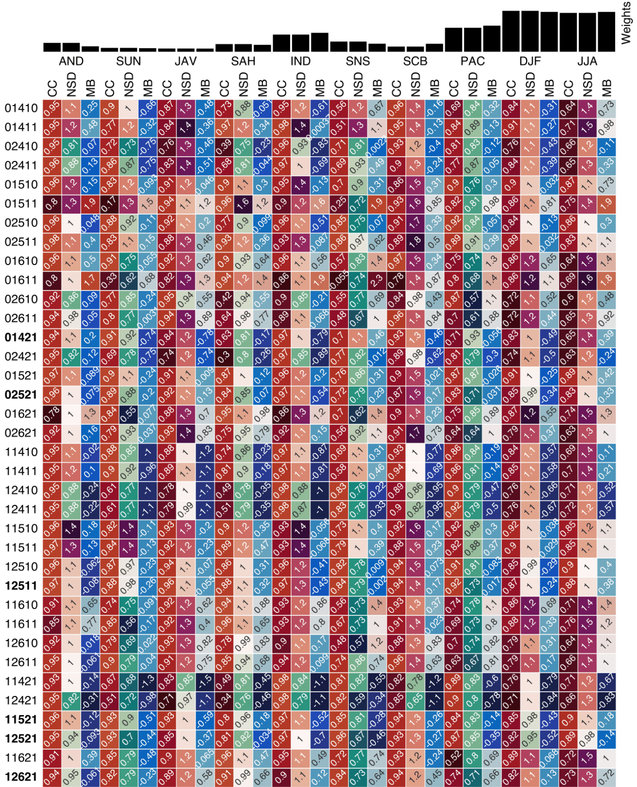
770 Figure B6: As in Fig. B1, but for SSW.
