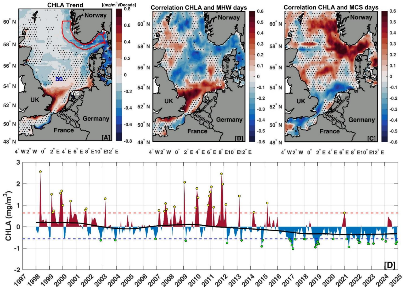
Figure 13: (A) Trend map of CHLA ( \text{mg/m}^3/\text{decade} ) and the correlation maps between (B) MHW days and CHLA and (C) MCS days and CHLA over the period between 1998 and 2024. (D) The average monthly CHLA over the Norwegian Trench (the area bounded by the red contour in panel A) between 1998 and 2024. The thick black line represents the LOWESS trendline. The yellow/green circles show high/low CHL events where CHLA was greater/smaller than the defined 90/10 percentiles (red/blue dashed horizontal lines), which were chosen to be seasonally independent for simplicity (i.e., fixed thresholds). In (A, B, and C), the dotted areas indicate that the trend or correlation is insignificant.
