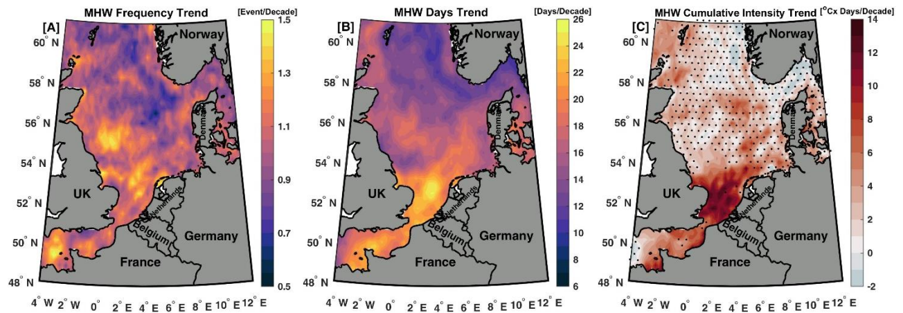
Figure 8: Decadal trends of (A) MHW frequency (events/decade), (B) MHW days (days/decade), and (C) MHW cumulative intensity (°C. days/decade) between 1992 and 2024. The dotted areas in (C) indicate that the trend is insignificant at a 95% significance level.
