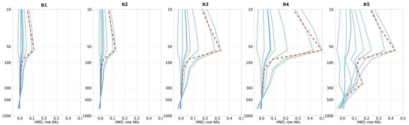
Figure 2: The eight CLIMCAPS averaging kernel (AK) functions (blue lines) for an \text{HNO}_3 retrieval on 2 February 2020 at 70.9^\circ\text{N} , 80.9^\circ\text{E} according to each of the five experimental configurations, (left) R1 to (right) R5. CLIMCAPS retrieves \text{HNO}_3 on eight broad pressure layers as defined in Table 1. The dashed red line is the diagonal vector of the 8 \times 8 AK matrix to summarize the peak SNR of each AK function.
