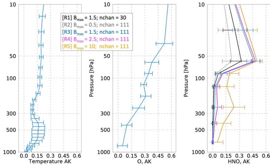
Figure 32: A statistical summary of CLIMCAPS signal-to-noise ratio (SNR) for all the temperature (left), O_3 (middle) and HNO_3 (right) retrievals north of 40^\circ N latitude on 2 February 2020. The profiles represent the average of the respective averaging kernel matrix diagonal vectors (AKD) profiles for (left) T_{air} , (middle) O_3 and (right) HNO_3 . These profiles represent the average of all diagonal elements from the AK matrices reported in the Level 2 product file for each retrieval parameter at every footprint poleward of 40^\circ N latitude on 2 February 2020, with standard deviation. The error bars represent the standard deviation of the AK profiles, indicate the degree to which CLIMCAPS SNR varies across retrieval pressure layers within the study region. CLIMCAPS retrieves temperature on 31 pressure levels, O_3 on 11 layers, and HNO_3 on 8 layers, hence the difference in the number of error bars across the three variables.
