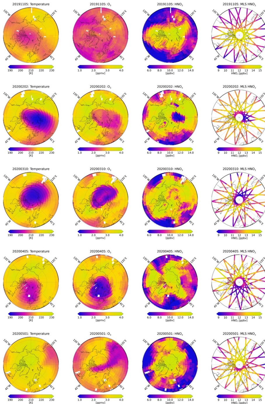
Figure 5: A time series of lower stratospheric (30–90 hPa) CLIMCAPS retrievals of T_{\text{air}} , O_3 , and HNO_3 according to produced by the R4 experimental configuration aggregated onto a 4^\circ equal-angle grid throughout the 2019/2020 Northern Hemisphere winter season poleward of 40^\circ N latitude. The column on the right represents the MLS V5 Level 2 profile HNO_3 retrievals at 1.5^\circ intervals. Both
