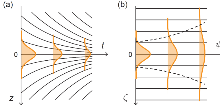
Figure 2. Evolution of a Gaussian signal in (a) t - z space and (b) \psi - \zeta space. Solid black curves signify material trajectories. Dashed curve in (b) marks the unthinned signal width, whose square increases at a rate with respect to \psi that reflects the instantaneous diffusivity.
