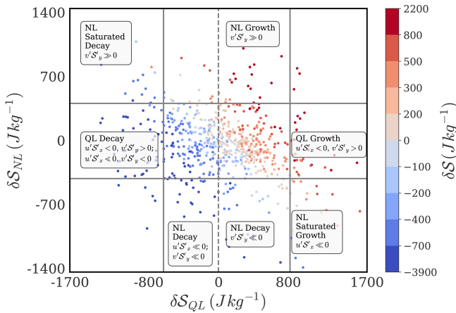
Figure 7. This figure shows the phase relationship between \delta S_{QL} and \delta S_{NL} colored by deciles of \delta S , for pre-existing positive lower tropospheric DSE anomaly ( S'_{Tot, Lag1} > 0 ) conditions during April. Solid grey lines demarcate the 10th and 90th percentiles of \delta S_{QL} and \delta S_{NL} . Regime definitions are provided in Sect. 5.1.1.
