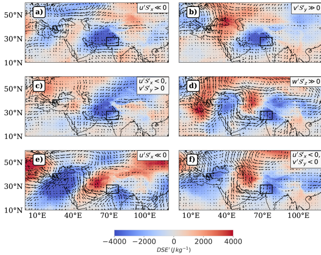
Figure 10. This figure shows the composite representations of horizontal wind anomaly vectors and S'_{\text{Tot, Lag1}} corresponding to the dominant nonlinear combination per advection regime amplifying and dissipating a pre-existing negative lower tropospheric DSE anomaly ( S'_{\text{Tot, Lag1}} < 0 ) during April, as defined in Fig. 9. The order of regimes is as follows: (a) QL + NL Growth, (b) NL Saturated Growth, (c) QL Growth, (d) QL + NL Decay, (e) NL Saturated Decay, (f) QL Decay. The upper right textbox in each panel annotates the dominant nonlinear combination for the corresponding regime. Table S5 clarifies the representativeness of an advection regime by the plotted nonlinear combination in the column “% Contribution”. The color coding represents S'_{\text{Tot}} values ranging from -4000 to 4000 \text{ J kg}^{-1} , with stronger hues indicating larger magnitudes.
