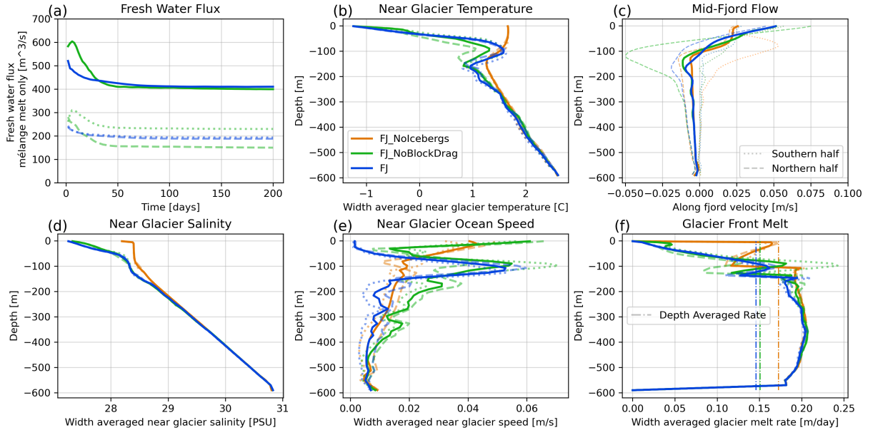
Figure C1. Impact of icebergs and drag on fjord level values. (Aa) Freshwater flux, including only mélange melt for the full 200 days. (Bb) Average temperature within 800 meters of the glacier terminus. (Cc) Average along fjord ocean velocity in the mid-fjord region averaged over the final 18 days. Dashed lines show the northern half of the fjord, dotted lines show the southern half of the fjord, solid lines are the average across the entire width. (Dd) Average salinity within 800 meters of the glacier terminus. (Ee) Average ocean speed within 800 meters of the glacier terminus. (Ff) Average glacier front melting rate. All frames share the color legend of panel (Bb).
