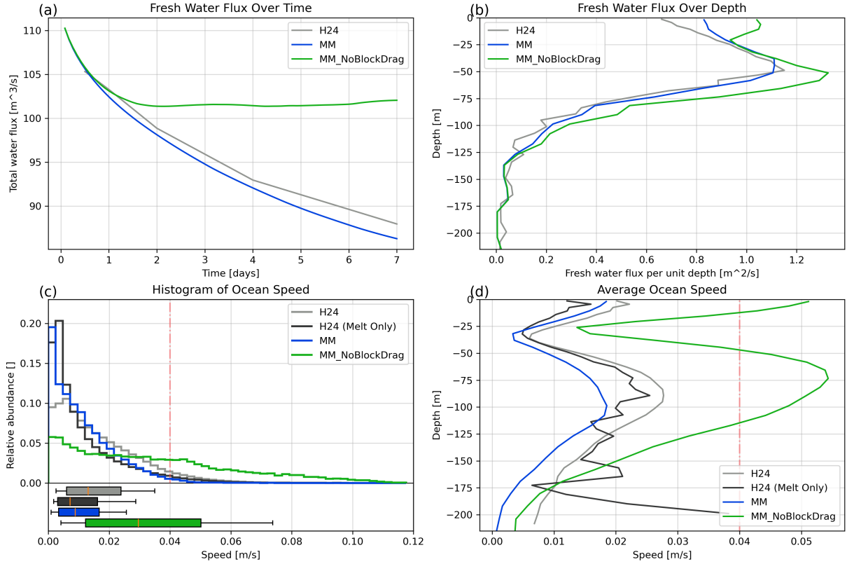
Figure 9. Impact of iceberg drag on meltwater production. (Aa) Total meltwater production over time, (Bb) Meltwater production over depth, (Cc) Histogram of ocean speed within the mélange pack, as well as whisker plots showing 10,25,50,75,90 percentiles. (Dd) Average ocean speed across the mélange pack as a function of depth. The red dash-dot line in Cc,Dd is the minimum melting velocity used in our melt parameterization. Panels b-d show values averaged over the final 2 hours of simulation.
