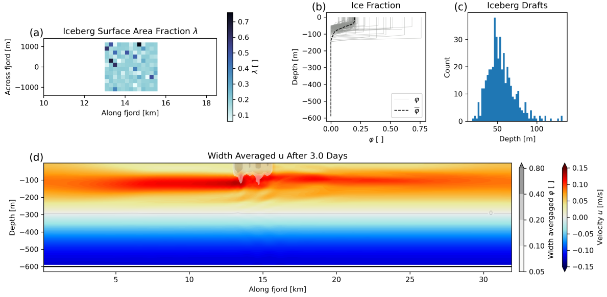
Figure 3. The configuration of our model domain for the \bar{\lambda} = 0.20 , U = 0.12 m/s case. (Aa) Distribution of \lambda across the mélange pack. (Bb) Depth variance of \phi . Light gray shows \phi(z) of every cell containing icebergs, and black dashed line shows the average \phi over the entire mélange area, \bar{\phi}(z) . (Cc) Histogram of iceberg drafts. (Dd) Width-averaged-Width-averaged velocity of our model domain at the end of simulation. Cells are shaded with the width-averaged-width-averaged value of \phi to illustrate the location of the mélange pack.
