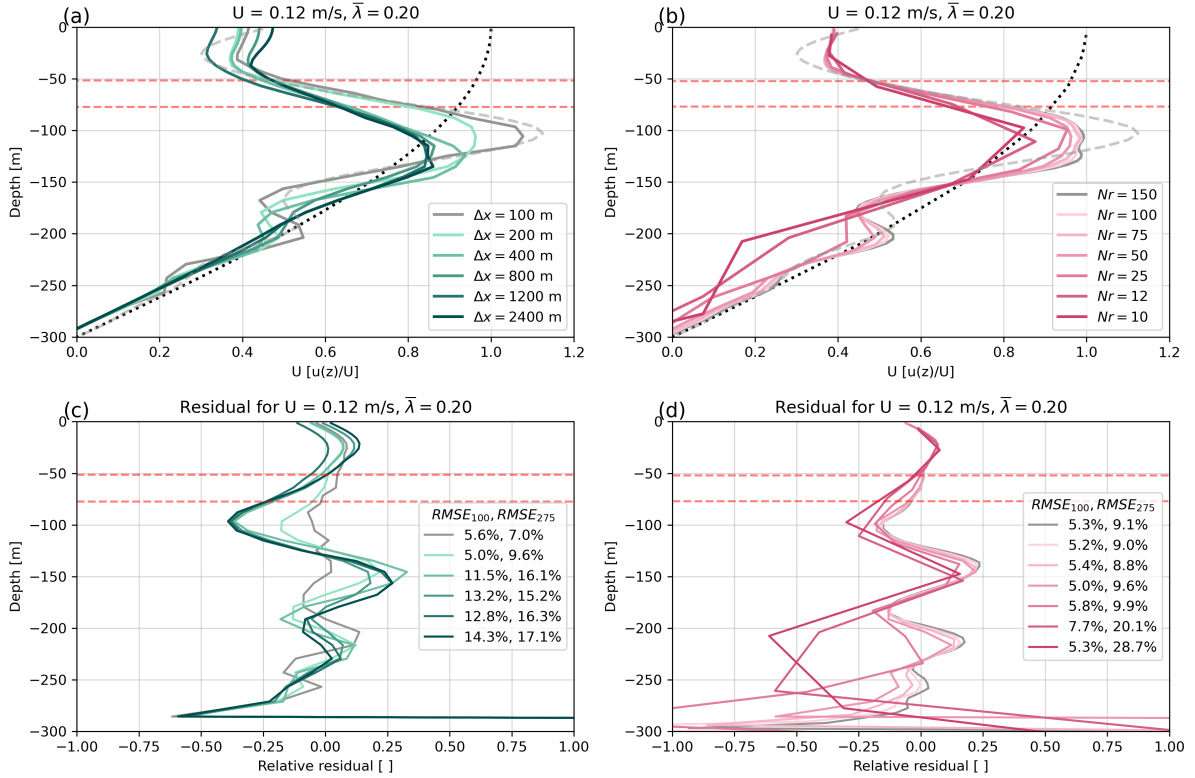
Figure 5. Ocean velocity averaged over the mélange pack for a range of Nr , \Delta x values for U = 0.12 , \bar{\lambda} = 0.2 . Fine gray Black dotted line is the driving velocity, and the coarse gray line is the results from Hughes (2022) for the same U , \bar{\lambda} . Red dashed lines are the median and 90th percentile of iceberg draft. Cc , Dd show the relative residual \epsilon (equation 8) for Aa , Bb respectively, and list the RMSE_{100} , RMSE_{275} for each case in the legend. Cc , Dd share the color scale of Aa , Bb respectively.
