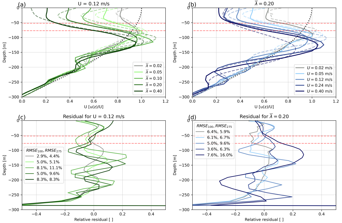
Figure 4. Along-fjord ocean velocity averaged over the mélange pack for a range of \bar{\lambda} in A-a and range of U in B-b . Solid lines are this study, dashed lines are Hughes (2022) for the same conditions. Gray-Black dotted line is the driving velocity. Velocities are normalized by the driving velocity ( U ). Red dashed lines are the median and 90th percentile of iceberg draft for \lambda = 0.2 . C-c , D-d show the relative residual \epsilon (equation 8) for A-a , B-b respectively, and list the RMSE_{100} , RMSE_{275} for each case in the legend. C-c , D-d share the color scale of A-a , B-b respectively.
