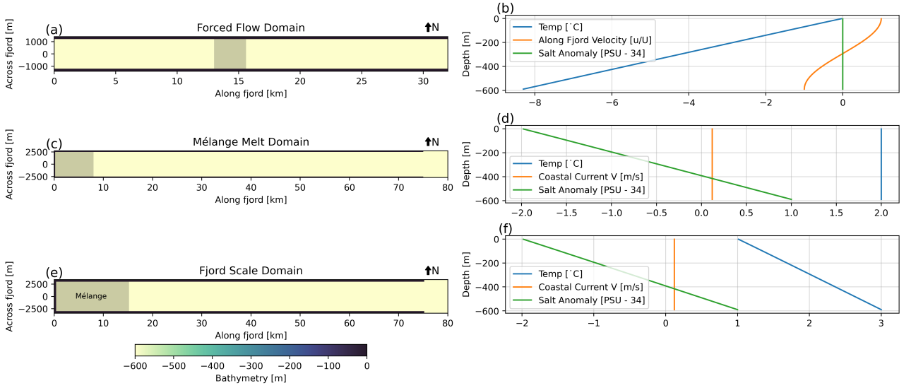
Figure 2. Model domains and boundary conditions for our three model configuration. (Aa,Bb) Bathymetry and forcing conditions for the forced flow domain following Hughes (2022). (Cc,Dd) Bathymetry and initial/boundary conditions for the mélange melt domain following Hughes (2024). (Ee,Ff) Bathymetry and initial/boundary conditions for our fjord scale domain. In Aa,Cc,Ee gray shading indicates the location of the ice mélange and black regions are the wall boundaries of bathymetry = 0.
