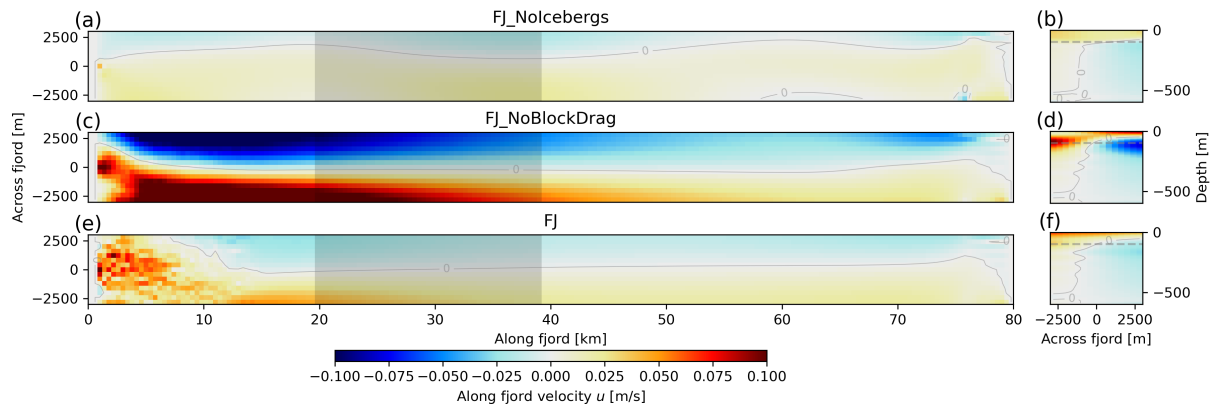
Figure 12. Comparison of Fjord Scale Domain results in map-view for z = -100 meters ( Aa , Cc , Ee ) and cross-sectional view of the midfjord region ( Bb , Dd , Ff ) for along-fjord velocity u . Aa , Bb show along-fjord velocity for the FJ_NoIcebergs case. Cc , Dd show along-fjord velocity for the FJ_NoBlockDrag case. Ee , Ff show along-fjord velocity for the FJ case. Gray shaded region in Aa , Cc , Ee is the midfjord region that is shown in panels Bb , Dd , Ff respectively. Gray dashed line in Bb , Dd , Ff is the -100 m depth that is shown in map-view in panels Aa , Cc , Ee respectively. In all panels the u = 0 contour is plotted as a thin gray line. All panels are temporally averaged over the final 18 days of simulation.
