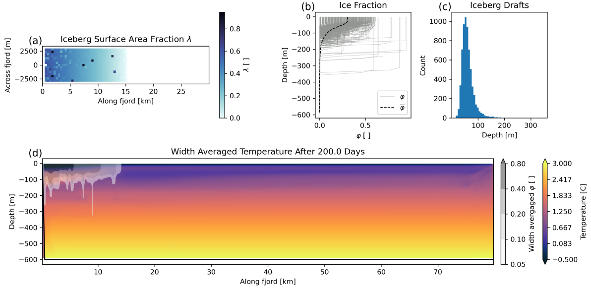
Figure 10. The configuration of our model domain for the full fjord run. (Aa) Distribution of \lambda across the mélange pack. (Bb) Depth variance of \varphi . Light gray shows \varphi(z) of every cell containing icebergs, and black dashed line shows the average \varphi over the entire mélange area, \bar{\varphi}(z) . (Cc) Histogram of iceberg drafts. (Dd) Width-averaged temperature of our model domain at the end of simulation. Cells are shaded with the width-averaged value of \varphi to illustrate the location of the mélange pack.
