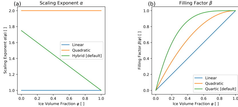
Figure A1. Visualization of the parameters \alpha, \beta and their variation with ice volume fraction \phi .
