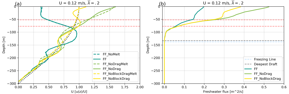
Figure 6. (Aa) Ocean velocity averaged over the mélange pack for a range of blocking, drag, and melt options for U = 0.12 , \bar{\lambda} = 0.2 . Fine gray-Blue dotted line is the driving velocity. Red dashed lines are the median and 90th percentile of iceberg draft. (Bb) Freshwater production rates, averaged over the mélange pack, per unit depth for a range of block and drag options. No melt cases are omitted. Red dashed lines are the median and 90th percentile of iceberg draft, black dashed line is the deepest draft, and the blue dashed line is the depth where the ambient temperature drops below the freezing point.
