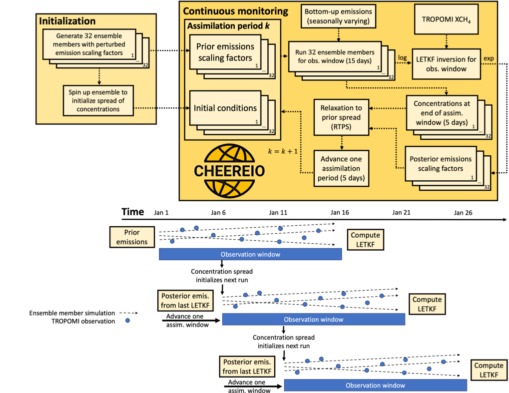
Figure 1: Flowchart of CHEEREIO v1.3.1 LETKF inversion procedure for assimilating TROPOMI methane data. We initialize a GEOS-Chem CTM simulations with randomized multiplicative perturbations to the prior estimates, applied to each of the 32 ensemble members. For assimilation period k , CHEEREIO runs GEOS-Chem for the observation window (15 days) for each ensemble member, then conducts the LETKF inversion by comparing the ensemble of GEOS-Chem values to the TROPOMI observations. over the observation window. Posterior emission scaling factors and concentrations are then inflated to reflect the prior spread using the RTPS procedure. The posterior emission estimates and inflated concentrations then become the prior estimate for the k+1 assimilation period advancing by 5 days.
