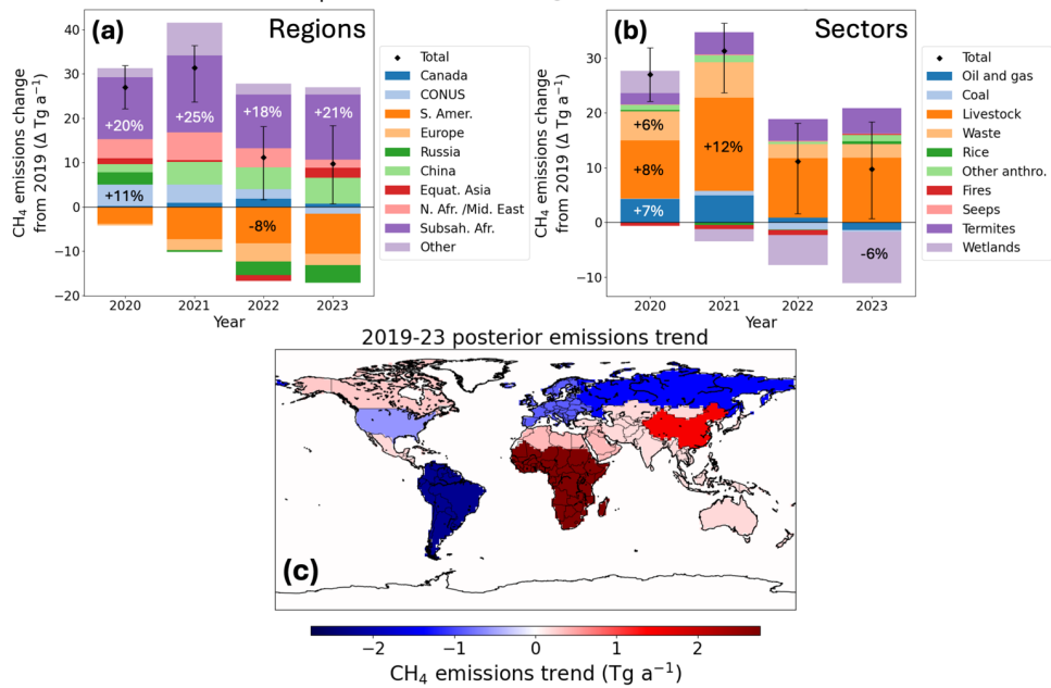
CH 4 emissions change relative to 2019
