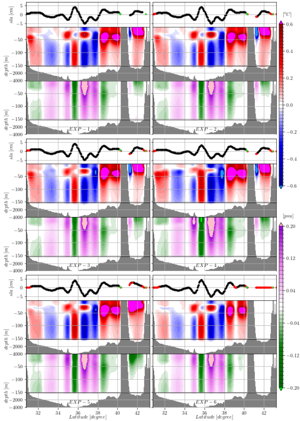
665 Fig.3 SLA, Temperature (red/blue) and Salinity (magenta/green) increments obtained from the different OceanVar2 configurations listed in Table1, starting from the same misfits. The SLA track used is drawn in green in Fig.1. For each experiment in the top panel there are the SLA increments where black dots indicate assimilated data, green dots indicate data
