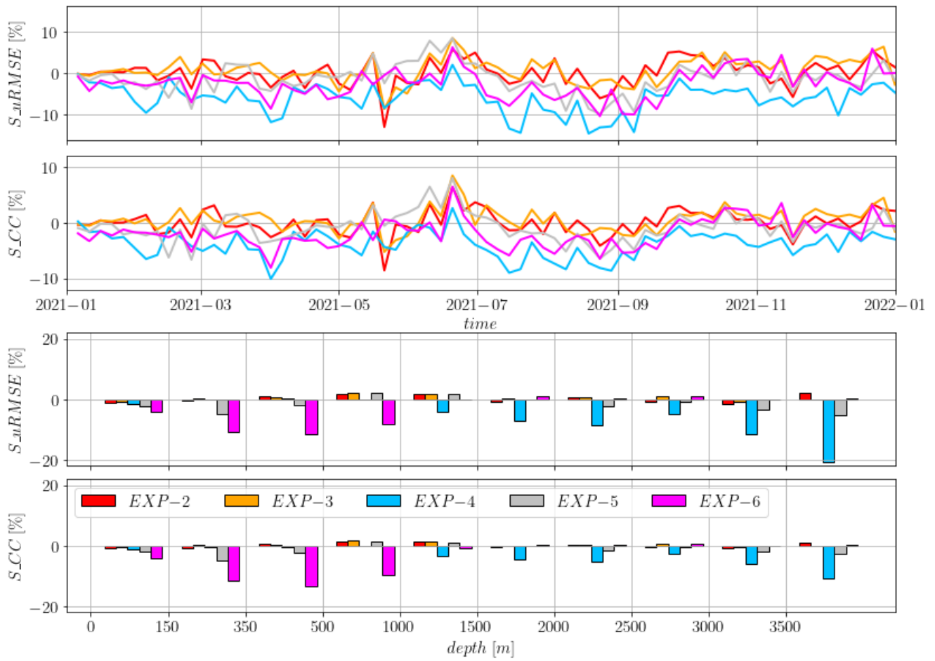
690 Fig.8 S_{uRMSE} and S_{CC} indices for % of improvement of the SLA errors for the different experiments w.r.t Exp-1. Top two panels: time-series. Bottom panels: average indices for bathymetry classes.
