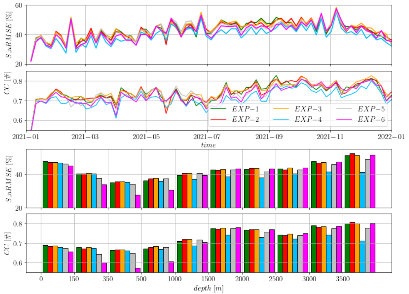
685 Fig.7 S_{uRMSE} and CC indices for the SLA misfit errors for the different experiments. S_{uRMSE} is computed w.r.t the free-run. Top two panels: time-series. Bottom panels: average indices for bathymetry classes.
