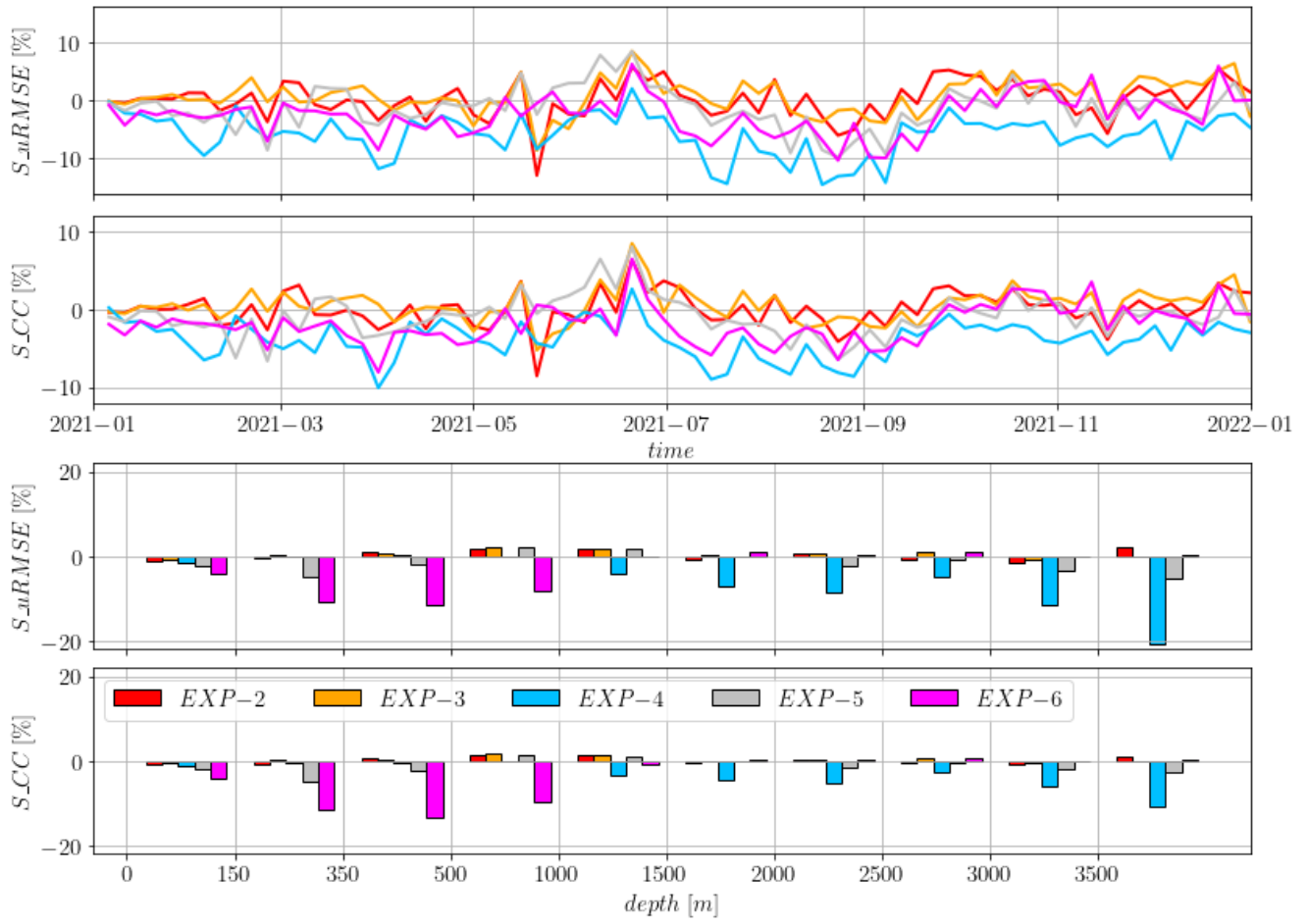
Fig.8 S_{uRMSE} and S_{CC} indices for % of improvement of the SLA errors for the different experiments w.r.t Exp-1. Top two 690 panels: time-series. Bottom panels: average indices for bathymetry classes.
