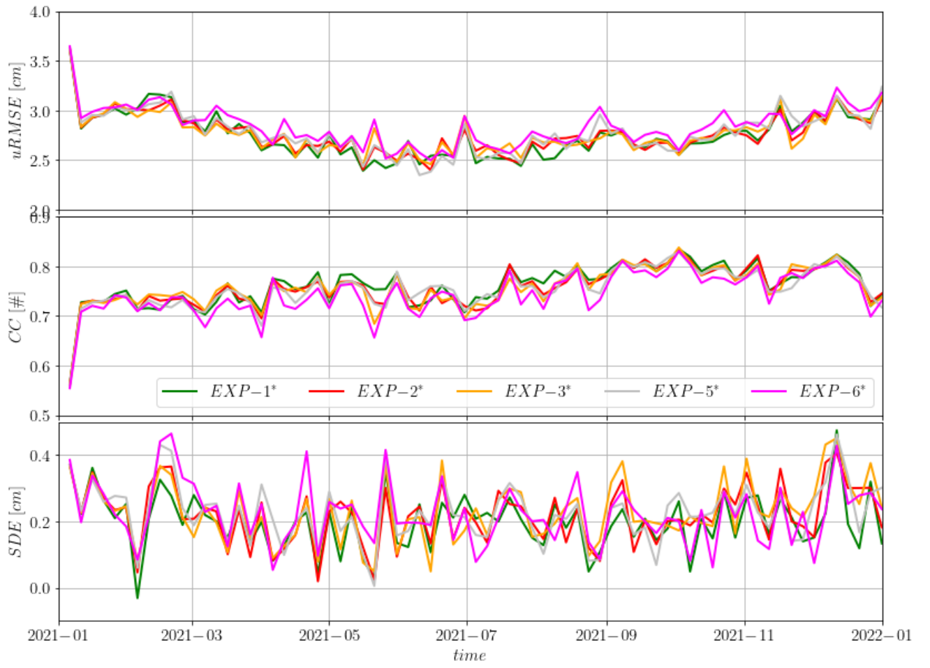
Fig.9 Second set of experiments SLA time series error statistics. Top panel: unbiased root-mean-square error. Middle panel: correlation coefficient. Bottom panel: standard deviation error. Colour code is provided in the middle panel legend.
