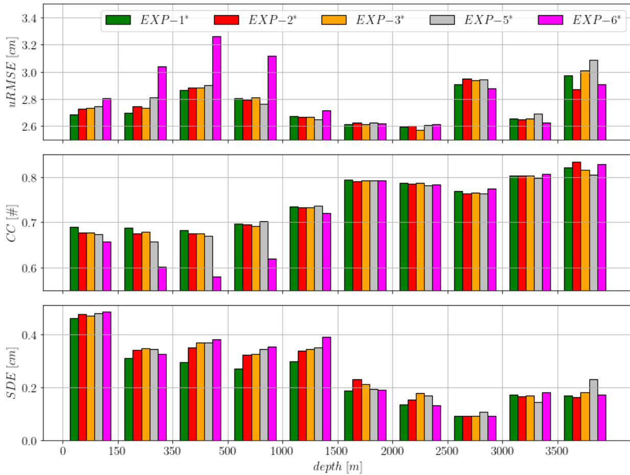
695 Fig.10 SLA statistics as a function of the ocean depth. Top panel: unbiased root-mean-square error. Middle panel: correlation coefficient. Bottom panel: standard deviation error. Colour code is provided in the top panel legend.
