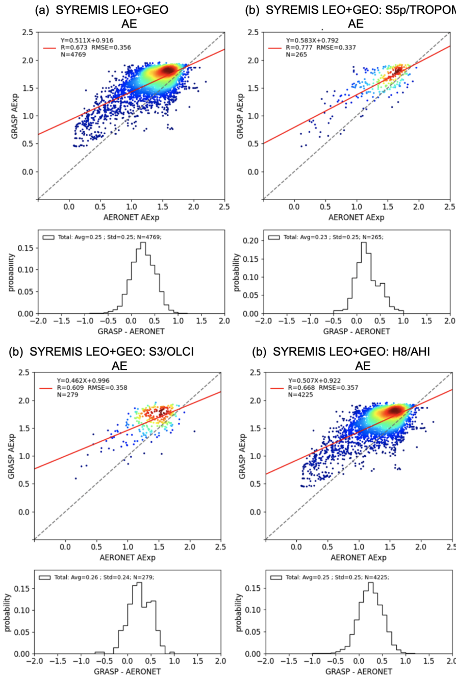
682 683 Figure 15: Angstrom Exponent (AE) validation against AERONET data over land for SYREMIS LEO+GEO synergetic retrieval in 684 2019 March, April, and May. (a): validation of AE of all instruments in the synergy; (b): validation of AE of SSP/TROPOMI
