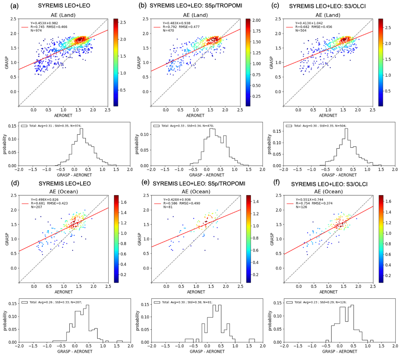
Figure 6: The same as in Fig. 5, but for Angstrom Exponent validation vs AERONET. Similar to AOD validation plots in Figs. 4 and 5, in the scatter plot, the color of each datapoint indicates the 2D probability density function value (increasing PDF value corresponds to color gradient from blue to red). In the legend in the top left corner of the scatter plots, the slope and intercept of the linear fit of the data points, the correlation coefficient R , and RMSE of the data points, and the number of data points N are indicated. Below each scatter plot, there is a corresponding histogram showing the error distribution, and in the legend over the top of the histogram, the bias between SYREMIS and AERONET AE (“Avg”), the standard deviation (“Std”), and the number of data points are indicated. The statistical metrics of each panel are summarized in Table 7.
