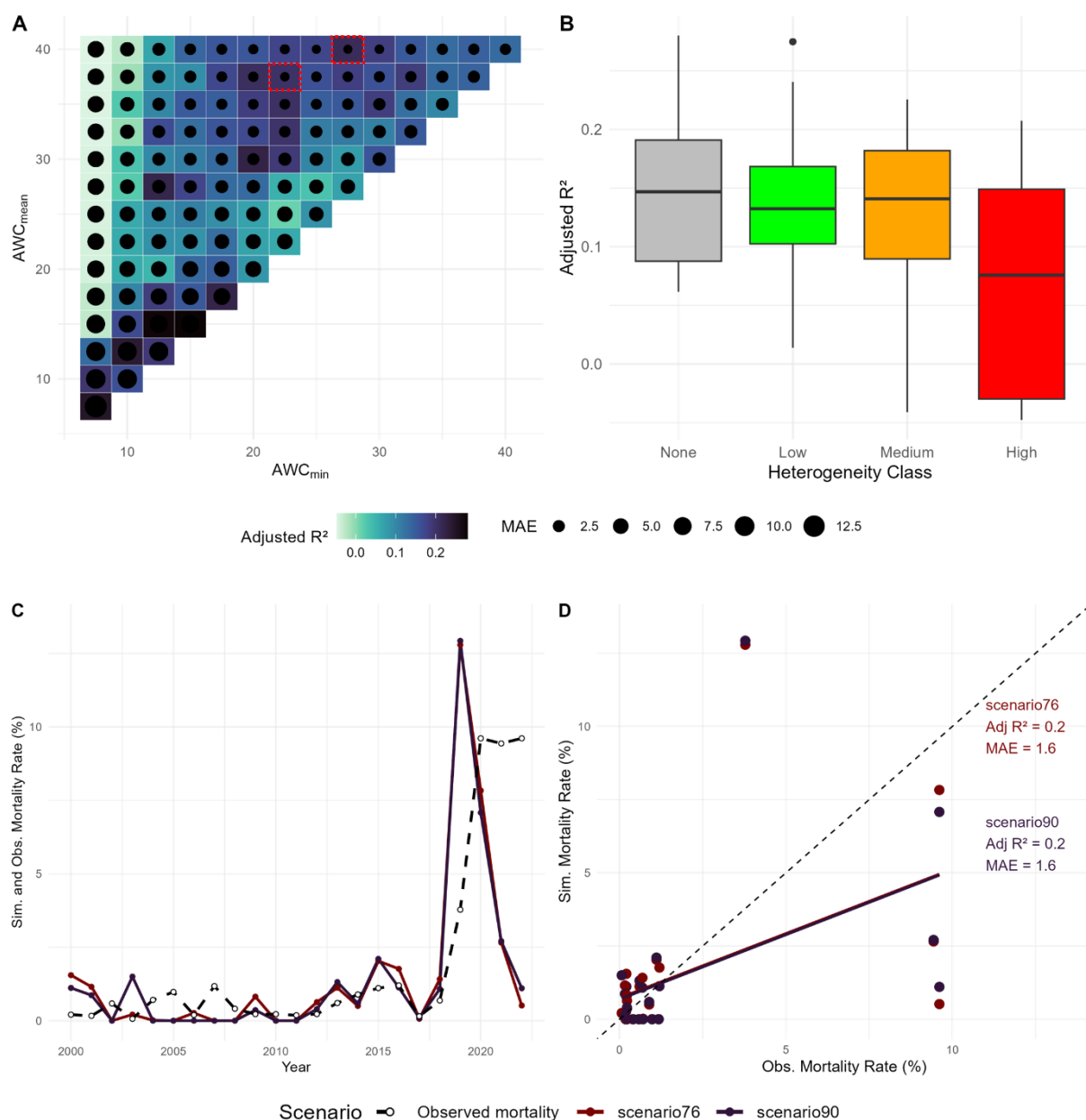
Figure 4. Evaluation of the performance of each soil water scenario in reproducing simulated tree mortality compared to observed tree mortality for Norway spruce dominated sites. (A) AWC scenarios showing adjusted R^2 and MAE. The two top-ranked AWC scenarios are indicated by dashed red boxes. (B) Adjusted R^2 and simulated mortality rate across soil heterogeneity classes (cf. Fig. 2). (C) Simulated (the two best AWC scenarios) and observed mortality rates (dashed line) over time for Norway spruce, and (D) model statistics for the two best AWC scenarios.
