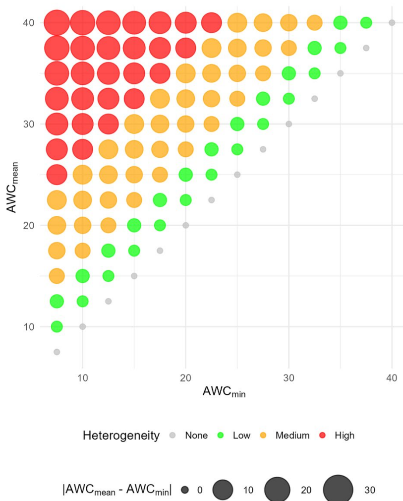
Figure 2. Soil scenarios defined as combinations of minimum and mean AWC. Distinct colors indicate the soil heterogeneity classes, ranging from no heterogeneity ( AWC_{min} = AWC_{mean} , None ), across low and medium to high heterogeneity classes.
