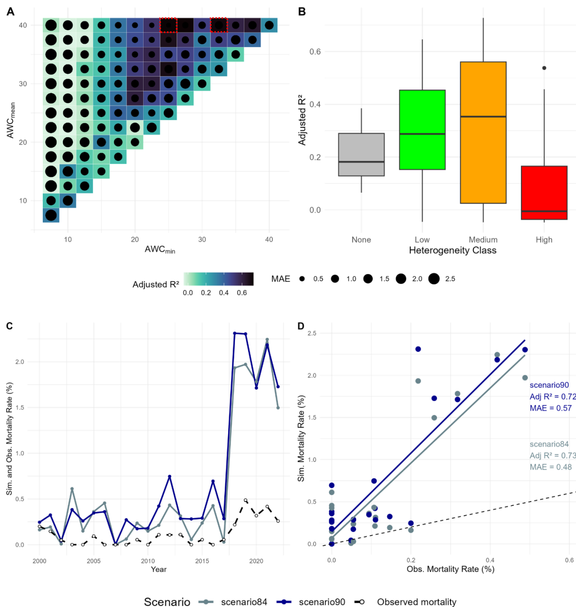
Figure 3. Evaluation of the performance of soil moisture scenarios in reproducing simulated tree mortality compared to observed tree mortality for European beech-dominated sites. (A) AWC scenarios showing adjusted R 2 and MAE. The two top-ranked AWC scenarios are indicated by dashed red boxes. (B) Adjusted R 2 and simulated mortality rate across heterogeneity classes (cf. Fig. 2). (C) Simulated (the two top-ranked AWC scenarios) and observed mortality rates over time across all sites, and (D) model statistics for the two top-ranked AWC scenarios.
