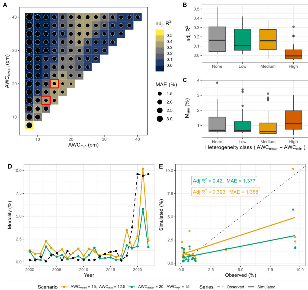
410 Figure 4. Evaluation of the performance of each soil water scenario in reproducing simulated tree mortality compared to observed tree mortality for Norway spruce dominated sites. (A) AWC scenarios showing adjusted R^2 and MAE. The two top- ranked AWC scenarios are indicated by red boxes. The top highest box (sixth row, starting from bottom) represents scenario 42, while the second box (fourth row, starting from the bottom) indicates scenario 29. (B) Adjusted R^2 and simulated mortality rate across soil heterogeneity classes (cf. Fig. 2) (C) Mean simulated mortality rate across heterogeneity classes. (D) Simulated 415 (the two best AWC scenarios, full lines) and observed mortality rates (dashed line) over time for Norway spruce, and (E) model statistics for the two best AWC scenarios. Scenario 29 is indicated in orange, while scenario 42 is in green.
