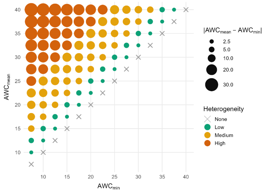
230 Figure 2. Soil scenarios are defined as combinations of minimum and mean AWC. Distinct colors indicate soil heterogeneity classes, ranging from no heterogeneity ( AWC_{min} = AWC_{mean} , None ), across low and medium to high heterogeneity classes.
