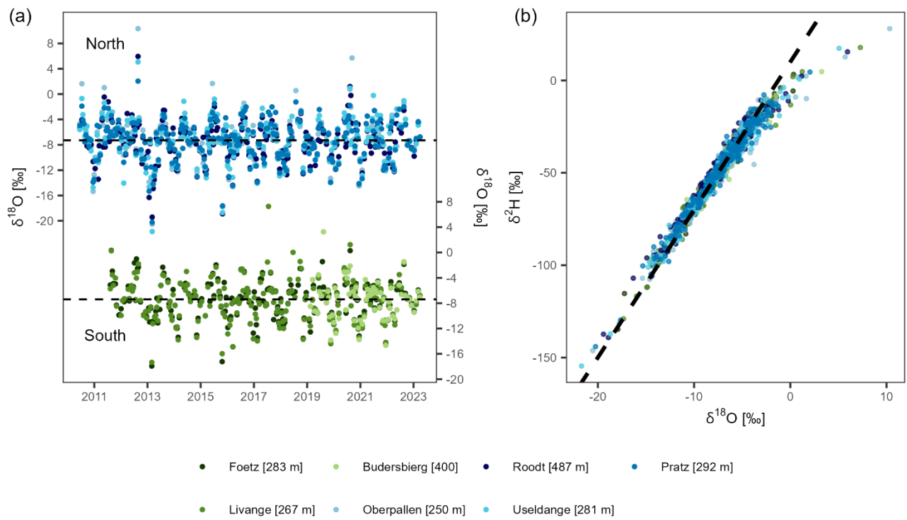
395 Figure 4: (a) Oxygen stable isotope composition of fortnightly precipitation samples of the seven rain gauges between 2011 and 2023. (b) Dual isotope plot (oxygen and hydrogen) and boxplots of the isotope composition at the seven rain gauges. The dashed line indicates the Global Meteoric Water Line (GMWL) with the equation \delta^2\text{H} = 10 + 8 \times \delta^{18}\text{O} .
