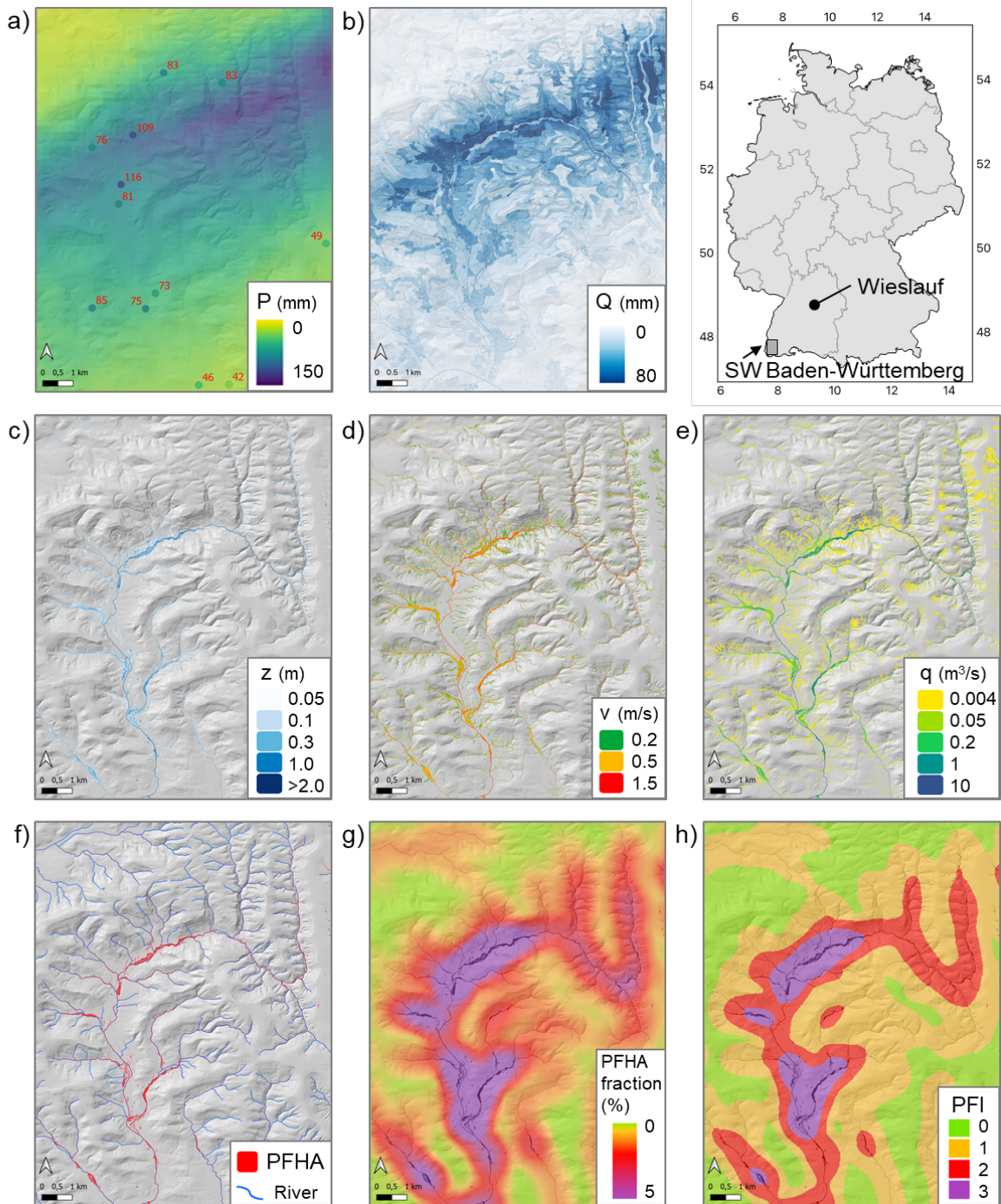
Figure 4: Hindcasting the flash flood event in the Wieslauf catchment at 02.06.2024 with a) total event radar-based QPE including measurements at stations at reported total event rainfall, b) total overland flow, c) maximum water depth (z) of the surface runoff with d) related maximum velocity (v), e) maximum specific surface runoff (q), f) resulting extend of the PFHA, g) PFHA fraction and h) PFI using a moving 2 km 2 circular reference area. Spatial resolution is 5 m. The SW Baden-Württemberg region also marked in the location overview panel is the focus regions of the analysis presented in section 4.2.
