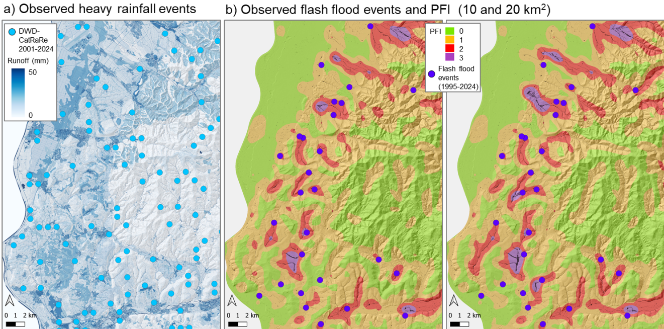
390 Figure 6: Comparison of the PFI hazard map with a) observations of heavy precipitations events with a duration less than 4 hours from the DWD-CatRaRe database and b) the locations of flash floods in comparison with the PFI with an accumulation threshold of (left) 10 km 2 and (right) 20 km 2 .
