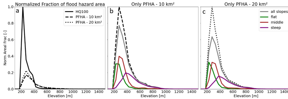
Figure 7: Comparison of PFHA with HQ100 flood extent. Panel a) shows the normalized (by the maximum number of HQ100 cells over all elevation bands) fraction of HQ100 as well as PFHA fractions (for two different accumulation thresholds) over the different elevation bands. Panels b and c show the normalized (by the maximum number of PFHA cells over all elevation bands) PFHA fraction for 10 km 2 and 20 km 2 , respectively. The stippled/dotted black line represent the distribution of PFHA fractions depicted in panel a. The grey line represents the distribution of the PFHA fraction outside of HQ100 areas, independent of cell slope. The coloured lines depict the same, but classified by the cells gradient.
