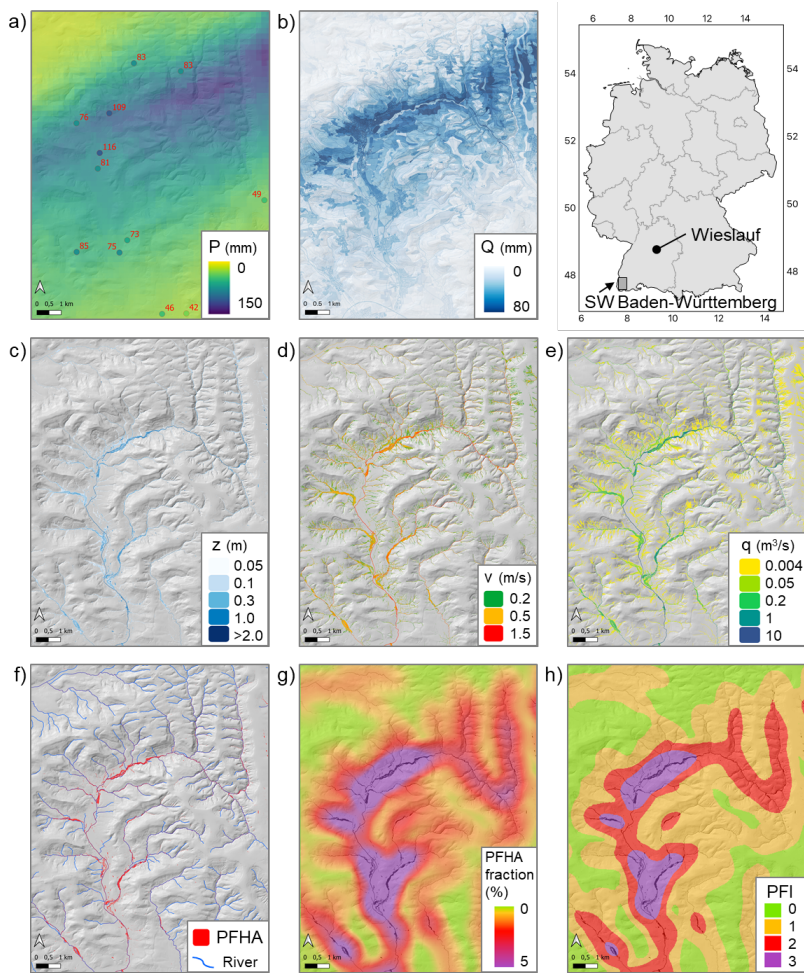
345 Figure 4: Hindcasting the flash flood event in the Wieslauf catchment at 02.06.2024 with a) total event radar-based QPE including 350 measurements at stations at reported total event rainfall, b) total overland flow, c) maximum water depth (z) of the surface runoff with d) related maximum velocity (v), e) maximum specific surface runoff (q), f) resulting extend of the PFHA, g) PFHA fraction and h) PFI using a moving 2 km 2 circular reference area. Spatial resolution is 5 m. The SW Baden-Württemberg region also marked in the location overview panel is the focus regions of the analysis presented in section 4.2.
