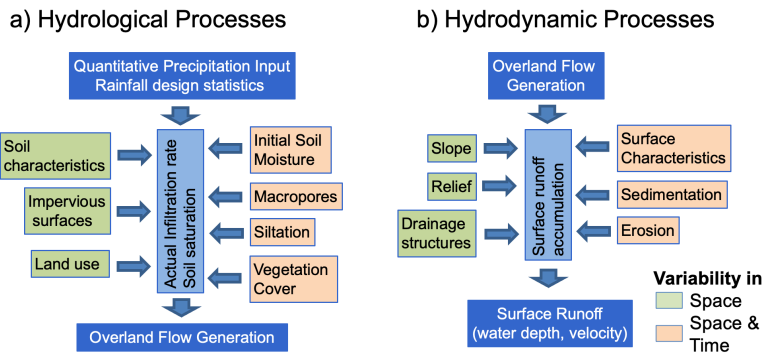
Figure 1: Factors and processes specific to the generation of overland flow and resulting surface runoff due to a) hydrological processes and b) hydrodynamic processes.
