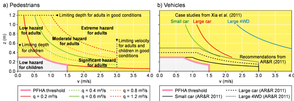
Figure 2: Experimentally derived criteria (water depth z and surface runoff velocity v ) for pedestrians (a) and vehicles (b) modified after Martínez-Gomariz et al. 2016 (a) and Martínez-Gomariz 2018 (b). The figure is supplemented by the selected criteria for delineating pluvial flood hazard areas (purple thick line) and the conditions of PFHA (yellow transparent area). The original citations for the two studies in (b) are provided in the reference section
