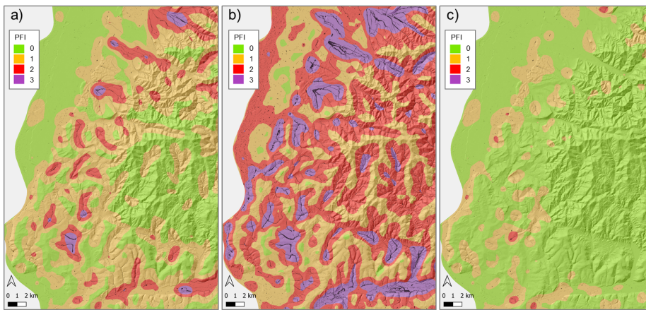
485 Figure 8: Comparison of the PFI hazard map using a) simulated surface runoff and b) precipitation estimates as input. Accumulation threshold for both maps is set to 10km 2 . In panel c) additionally a PFI hazard map based on surface runoff but with the river network as infiltration spots instead of a fixed accumulation threshold is shown.
