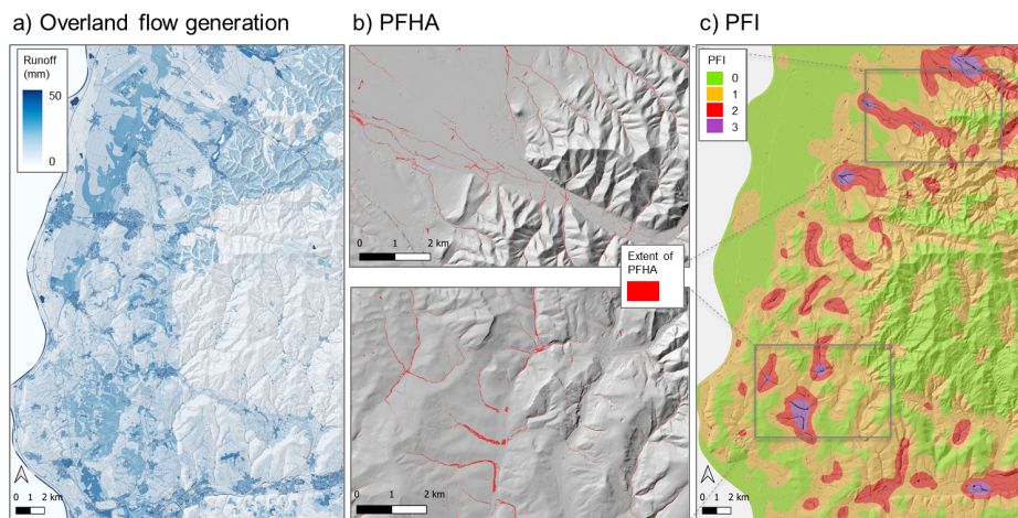
390 Figure 5: The three steps to derive PFI hazard maps: a) overland flow generation for a 1h precipitation event with a return period of 100 years simulated with a hydrological model, b) the resulting PFHA in two selected areas using a 2D hydraulic model with an accumulation threshold of 10 km 2 and c) the resulting PFI using a moving 2 km 2 circular reference area. Spatial resolution is 5 m.
