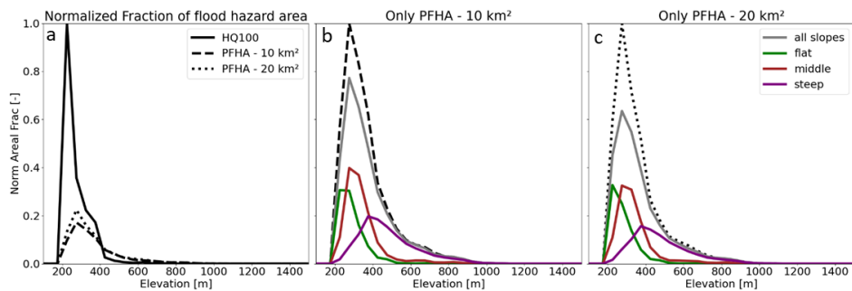
450 Figure 7: Comparison of PFHA with HQ100 flood extent. Panel a) shows the normalized (by the maximum number of HQ100 cells over all elevation bands) fraction of HQ100 as well as PFHA fractions (for two different accumulation thresholds) over the different elevation bands. Panels b) and c) show the normalized (by the maximum number of PFHA cells over all elevation bands) PFHA fraction for 10 km 2 and 20 km 2 , respectively. The stippled/dotted black line represent the distribution of PFHA fractions depicted in panel a). The grey line represents the distribution of the PFHA fraction outside of HQ100 areas, independent of cell slope. The coloured lines depict the same, but classified by the cells gradient.
