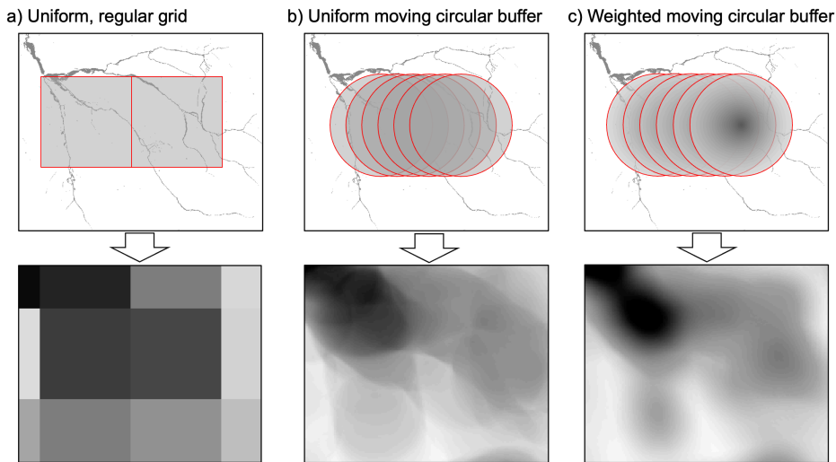
230 Figure 3: Comparison of the three potential approaches to derive the PFHA fraction from the PFHA for a defined reference area with a) shows the example of applying a uniform, regular grid, b) a uniform moving circular buffer and c) a weighted (radial linear) moving circular buffer with the resulting map of PFHA fraction with lower brightness indicating higher fractions.
