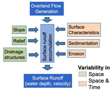
Figure 1: Factors and processes specific to the generation of overland flow and resulting surface runoff due to a) hydrological processes and b) hydrodynamic processes.
