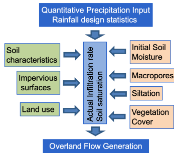
Figure 1: Factors and processes specific to the generation of overland flow and resulting surface runoff due to a) hydrological processes and b) hydrodynamic processes.
