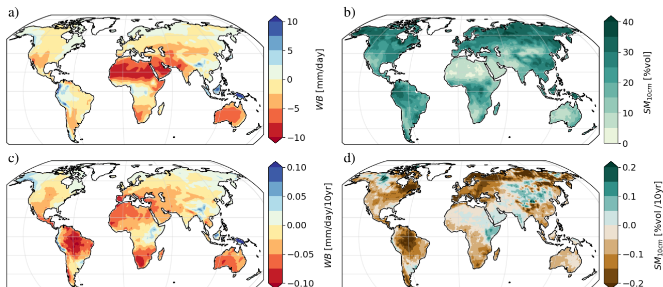
Figure 9. Temporal average a,b) and decadal change c,d) in a,c) global water budget ( PR-ET_0 ) and b,d) soil moisture projected from CMIP6 multi-model ensemble for the SSP2.4-5 scenario (2015-2100).
