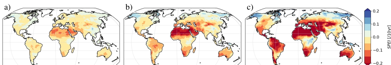
Figure 5. Decadal change rate of SPEI with reference period 1950-2014 derived from CMIP6 projections for different future scenarios. The change is defined as the absolute difference between 2015-2034 and 2081-2100 normalized to the average change over 10 years.
