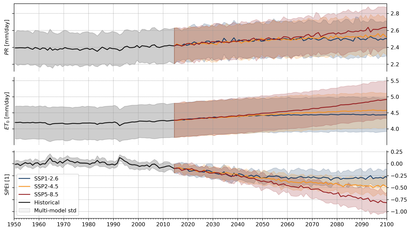
Figure 4. Annual precipitation, reference evapotranspiration and the derived SPEI. All variables are averaged over global land surface. The multi-model means of 18 CMIP6 models are drawn as solid lines, with shaded areas indicating the multi-model standard deviation. For the period (2015-2100) different future scenarios can be distinguished by color.
