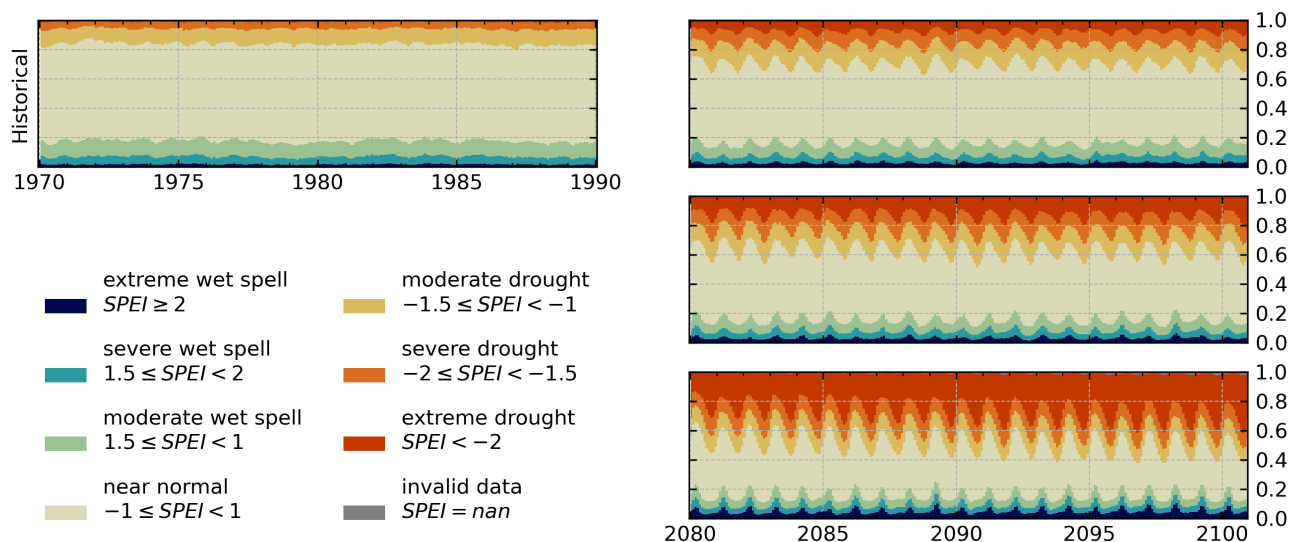
Figure 8. Timeseries of relative drought event area according to SPEI. The color indicates how much of the agricultural relevant regions area is covered by certain drought conditions for each month. A 20 year interval from the baseline period 1950-2014 is shown on the left, while the plots on the right display relative area by drought category over the last 20 years (2080-2100) of different future scenarios.
