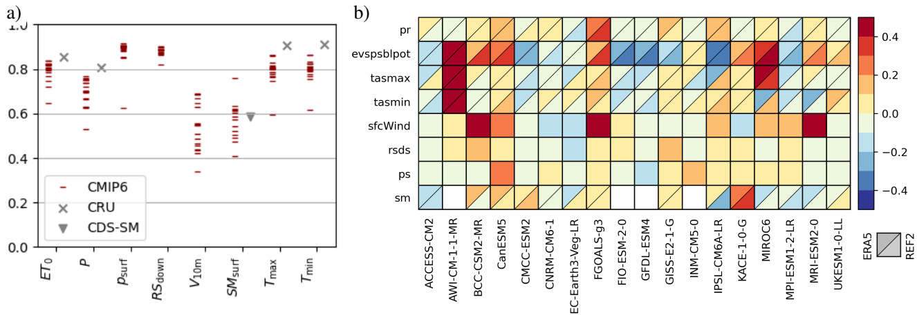
Figure 1. Overview of the CMIP6 multi-model performance compared to ERA5 reanalysis over land surface. In panel a) pattern correlation of historical CMIP6 simulations with ERA5 for precipitation ( PR ), reference evapotranspiration ET_0 , daily minimum and maximum temperature ( T_{min} , T_{max} ), wind speed at 10 m ( V_{10m} ), surface down welling shortwave radiation ( RS_{down} ), surface pressure ( p_{surf} ) and soil moisture ( SM_{surf} ) are shown. The data is averaged over the period 1980 to 2014. The additional markers show pattern correlation of ERA5 to CRU and CDS-SM. In panel b) the relative model performance for the same variables is shown. The root mean squared distance (RMSD) of each model to ERA5 is centered and normalized at the median RMSD. Negative (blue) values indicate that the model predicts results more similar with ERA5 compared to the other models. Red colors indicate worse performance. For some variables the performance compared to CRU is shown as well in the bottom right triangle. The alternative reference for SM_{surf} is CDS-SM.
