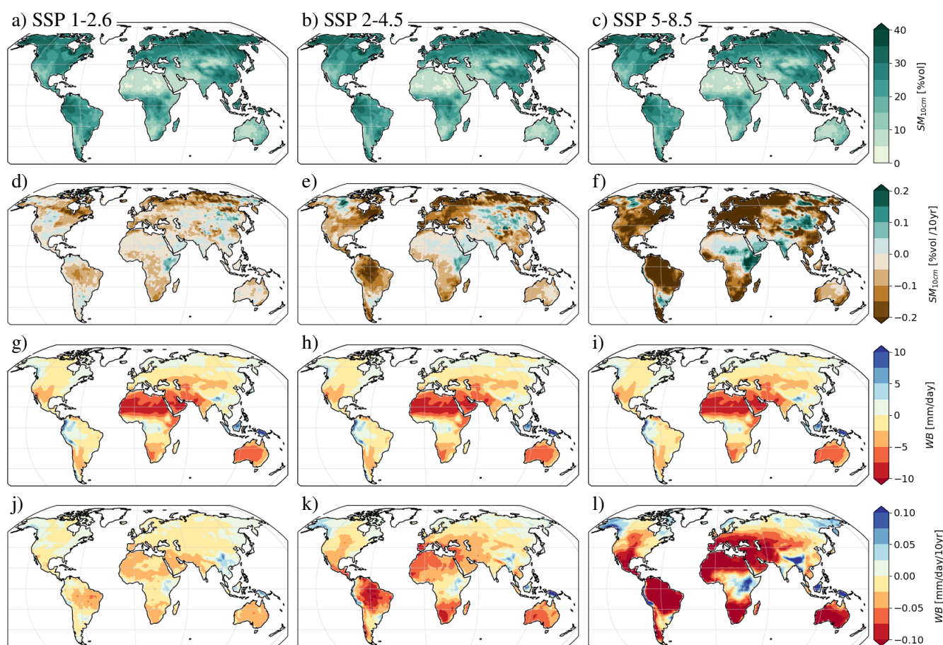
Figure A4. Change rate and average of soil moisture (a-f) and water budget (g-l) in different future scenarios (a,d,g,j: SSP 1-2.6, b,e,h,k: SSP 2-4.5, c,f,i,l: SSP 5-8.5) from 2015-2100.
