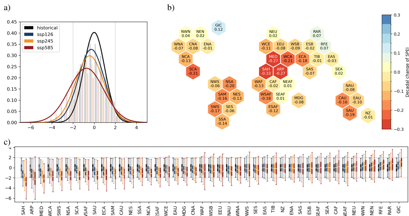
Figure A6. Global overview of SPEI values for the CMIP6 multi-model ensemble for different future scenarios. The global SPEI distributions for all non glaciated land grid cells for the historical period (1950-2014) and end of century (2070-2100) are shown in panel a) and regional distributions for the same periods in form of boxplots for IPCC AR6 WG1 reference regions in panel c). The hexagons in panel b) show the regional mean average decadal change of SPEI for each region only for SSP5-8.5. The regions are positioned relative to each other based on their real locations.
