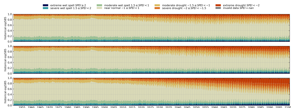
Figure A7. Complete time series of relative drought event area in harvest regions according to SPEI. The color indicates how much of the total non glaciated land surface area is covered by certain drought conditions from near normal.
