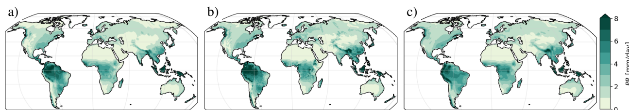
Figure 2. Global pattern of temporal mean precipitation based on a) ERA5, b) CRU and c) CMIP6 multi-model mean over the period 1980-2014.
