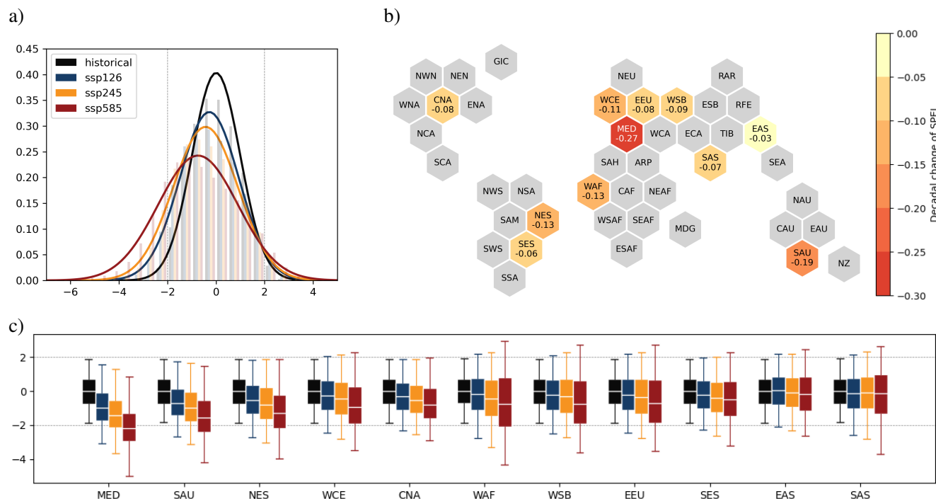
Figure 7. SPEI distributions for the CMIP6 multi-model ensemble in different future scenarios. The SPEI distributions for all grid cells in selected harvest regions are shown in panel a) and regional distributions in form of boxplots for IPCC AR6 WG1 reference regions (Antarctic excluded) in panel c). The hexagons in panel b) show the mean decadal change of mean SPEI for each of the selected region but only for the SSP5-8.5 scenario. The regions are positioned relative to each other based on their real locations.
