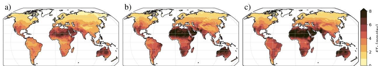
Figure 3. Global pattern of temporal mean of reference evapotranspiration ( ET_0 ) based on a) ERA5, b) CRU and c) CMIP6 multi-model mean over the period 1980-2014. For CRU the variable is taken from the dataset. For ERA5 and CMIP6 ET_0 is calculated from other atmospheric variables (Eq. 1) similar to the method used for CRU.
