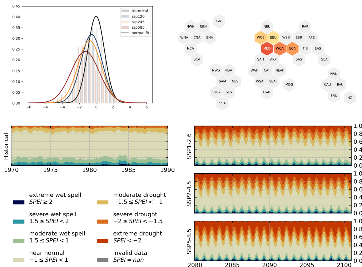
Figure A8. Analysis for 5 selected semi arid european and asian regions: WCE, EEU, MED, WCA, ECA.
