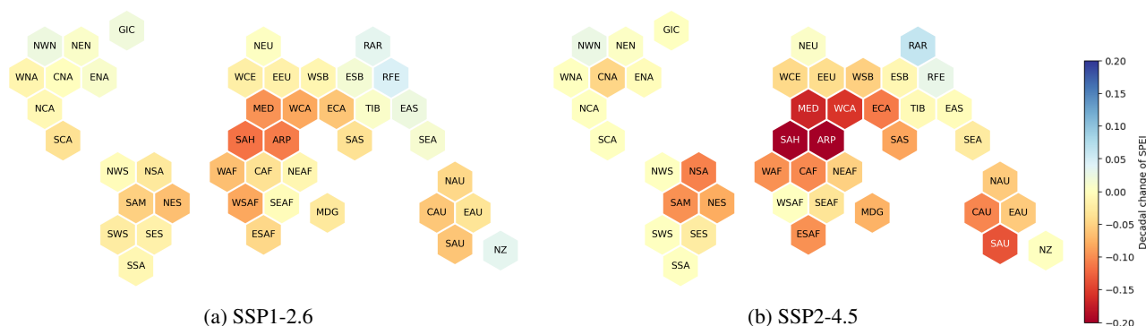
Figure A5. Average decadal change between 2015-2034 and 2081-2100 of SPEI in different future scenarios. Similar plot for SSP5-8.5 is shown in Figure 7b.
