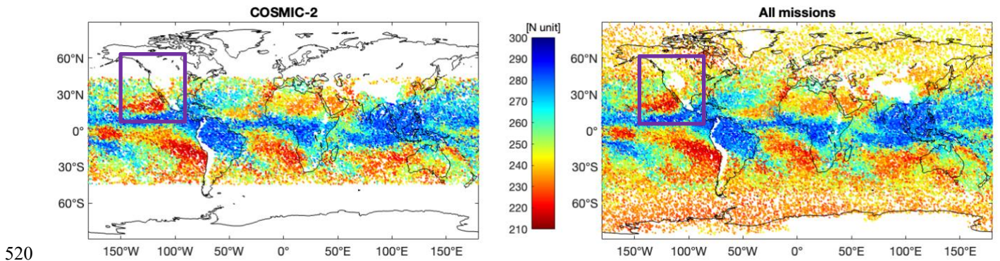
520 Figure 13: Refractivity at 2 km height from COSMIC-2 (left panel) and all available missions (right panel), during 22 nd and 27 th October 2021. The purple rectangle highlights the AR scene.
